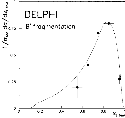
Fig. 5. Inclusive B^* cross-section in bins of x_{E}^{true} . The points are unfolded data; the curve is the JETSET 7.4 prediction fitted to the data with \langle x_E \rangle = 0.695
