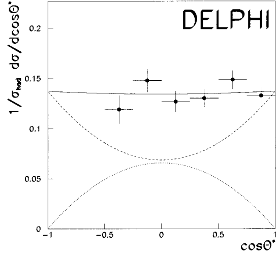
Fig. 6. Decay angular distribution for B^* photons in the B^* rest frame. The acceptance corrected data are represented by points. The solid line displays the result of a fit to longitudinal and transverse polarisation contributions. The dashed and dotted curves are the contributions from the transverse and longitudinal states
