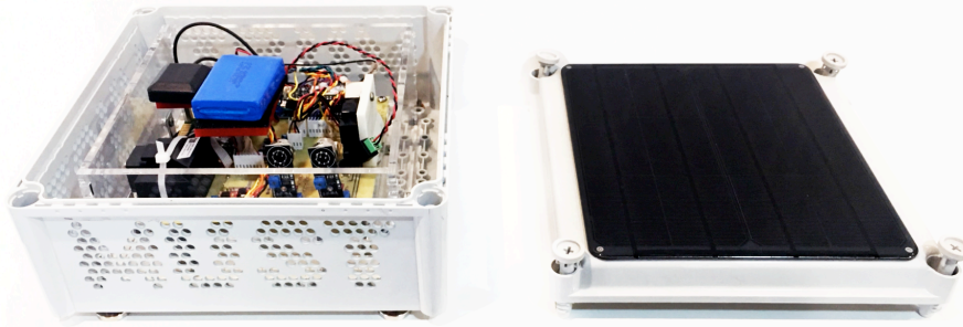
Figure 1. MUST Sensing Kit
