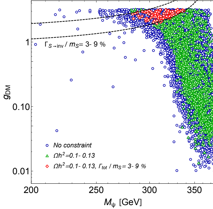
Figure 3: Markov-chain scan over the four dimensional model parameter space, projected onto the M_\psi, g_{DM} plane. The scan assumes a Gaussian likelihood function centered around \Omega h^2 = 0.12 , where the range of allowed parameters is bounded by g_{BB} = [10^{-2}, 2] , g_{GG} = [10^{-2}, 1] , g_{DB} = [10^{-2}, 3] and m_\psi = [200, 375] GeV. The blue circles represent the total of 10000 points scanned over by the Markov-chain, with no additional constraints. The green triangles represent a subset of the sampled points which give relic density in the range of 0.1 < \Omega h^2 < 0.13 . The red diamonds assume an additional requirement of \frac{\Gamma_{tot}}{m_S} = (3-9)\% GeV. The dashed lines represent the range in which the total width in the range of (3-9)\% of m_S can be explained by dominant decays into dark matter.
