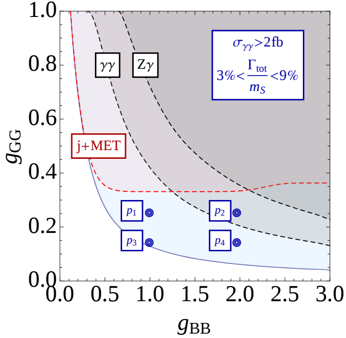
Figure 5: Summary of the parameter space allowed by collider constraints, in the g_{GG} and g_{BB} plane. We marginalise over M_\psi = [0, 600] GeV and g_{DM} = [0, 3] . Regions above dashed lines are ruled out by individual collider searches specified on the plot. The solid blue line corresponds to the region of parameter space which can provide \sigma(pp \rightarrow S \rightarrow \gamma\gamma) > 2 fb with dark matter mass of 300 GeV. The blue points labeled as p_{1-4} represent the benchmark model points we use as illustrations in the paper.
