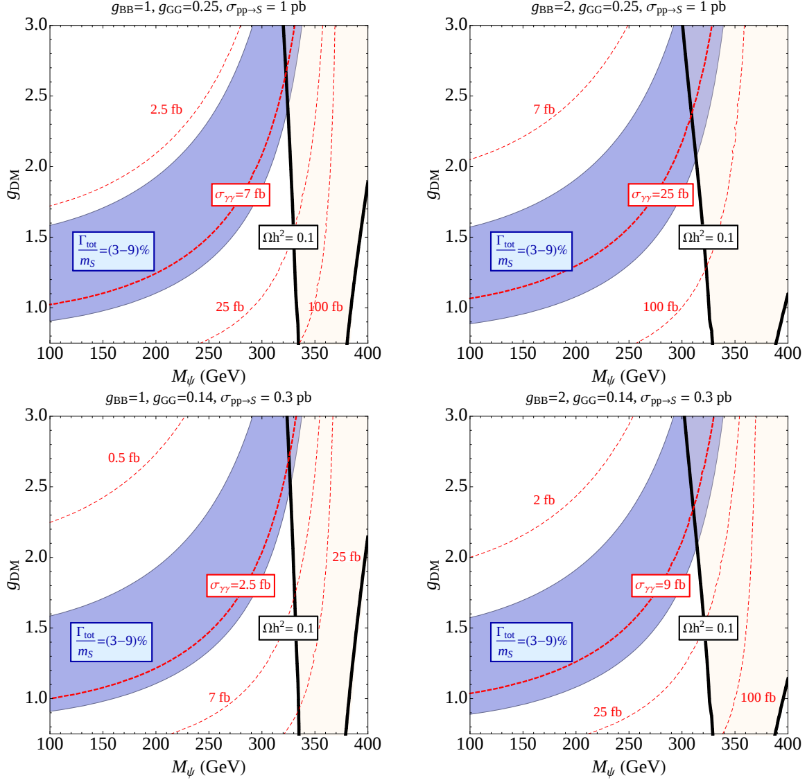
Figure 4: Interplay between the di-photon signal parameters and DM relic density. The four plots from the top left to the bottom right corresponds to our four benchmark choices in (2.3). The blue band shows regions where \frac{\Gamma_{\text{tot}}}{m_S} \approx (3-9)\% (in blue) while the region where \Omega h^2 < 0.1 is shown in pink. At the boundaries of the pink region (black, solid lines) the Dirac fermion accounts for all the DM relic abundance. We overlaid the contours of the di-photon production cross section at LHC 13 as dashed red curves. The thicker curve is the one corresponding to our selected benchmark with \Gamma_{\text{tot}} \approx 30 GeV. Notice that the regions where the width bands intersect the regions allowed by relic density constrains essentially fix the dark matter parameters.
