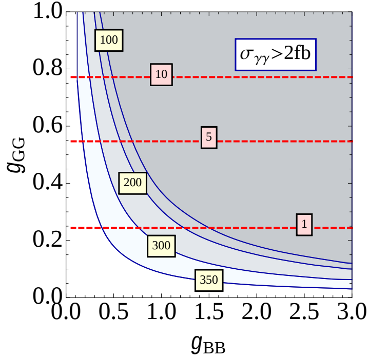
Figure 2: Parameter space (from blue to gray) in the plane of couplings (g_{BB}, g_{GG}) leading to \sigma(pp \rightarrow S \rightarrow \gamma\gamma) > 2 \text{ fb} at \sqrt{s} = 13 \text{ TeV} , for different choices of the DM mass M_\psi = (350, 300, 200, 100) \text{ GeV} , indicated on the boundaries of the regions. For the purpose of illustration, we fixed g_{DM} = 2.7 and \Lambda = 10 \text{ TeV} . The red dashed contours correspond to the production cross section at 13 TeV for a scalar singlet \sigma(pp \rightarrow S) in pb.
