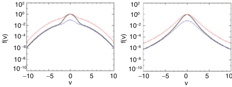
Fig. 2.6 Velocity filtration for a sum of two Maxwellians (left) and a Kappa (right). Here, v is the velocity normalized to the thermal speed w = \sqrt{2k_B T/m} . Black: VDF at low radial distance r_0 (e.g., r_0 = 1.1R_s ), blue: VDF at an upper radial distance r_1 ( = 3R_s ), and red: VDF at r_1 normalized so that the top of the distribution corresponds to the initial distribution, enabling to illustrate the velocity filtration and the temperature increase
