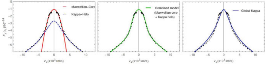
Fig. 2.2 Left panel: electron velocity distribution shown with dots (symmetric perpendicular cut) is fitted by a Maxwellian core (solid red) and a Kappa halo (dashed blue). The resulting dual fit (green) in the middle panel is more accurate than a global Kappa fit (solid blue) in the right panel. Credit: Lazar et al. (2017), reproduced with permission ©ESO
