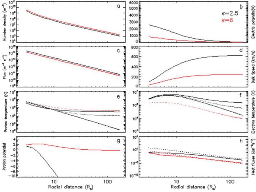
Fig. 2.11 Profiles of the moments for Kappa VDFs with \kappa = 2.5 in black and \kappa = 6 in red. Panel a. Density n(r) , b. Electric potential V(r) , c. Escape flux F(r) , d. Bulk speed u(r) , e. Proton temperature T_p(r) (dotted: total, solid upper at high r : T(r) parallel, lower solid at high r : T(r) perpendicular), f. Electron temperature T_e(r) (idem), g. Proton potential energy \Phi_p(r) , h. Heat flux Q(r) (solid: protons, dotted: electrons). Obtained with the exospheric model from Pierrard and Pieters (2014)
