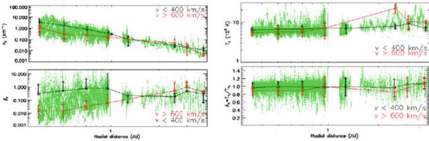
Fig. 2.4 Electron halo properties measured in the ecliptic with average values and their standard deviations estimated for the slow (black) and fast (red) winds. Credit: Lazar et al. (2020b), reproduced with permission ©ESO
