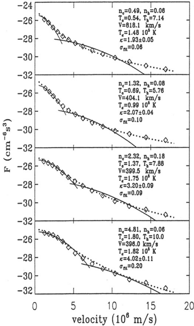
Fig. 2.1 Ulysses observations of electron velocity distributions (averaged over all pitch-angles) shown with diamonds are better fitted by a Kappa distribution function (dotted line) than a sum of two Maxwellians (solid lines). The core is well fitted by a cooler Maxwellian (subscript 'c'), but suprathermal tails are not reproduced by the second, hotter Maxwellian (subscript 'h'). The corresponding parameters from fitting, i.e., number densities n in \text{cm}^{-3} , temperatures in units of 10^5 \text{ K} , power exponent \kappa , as well as their (maximum) deviations \sigma_m are given in the legends. Reproduced with permission from Maksimovic et al. (1997b). © John Wiley and Sons
