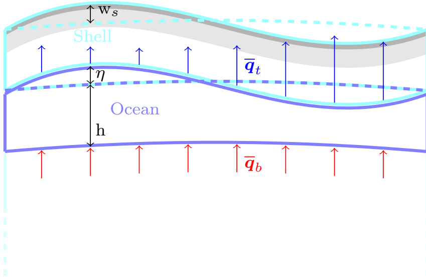
Figure 1: Geometry of a part of the domain. w_s denotes the vertical displacement of the ice shell (positive upwards), h is the unperturbed ocean depth, \eta is the surface elevation (positive upwards), \bar{q}_b is the (incoming) uniform heat flux at the bottom of the ocean, and \bar{q}_t is the (outgoing) spatially varying heat flux at the surface of the ocean. Light and dark blue represent the icy parts of the domain and the ocean, respectively. The dashed lines represent the unperturbed ocean/shell. The dark and light grey areas at the top of the ice shell represents the shell upper layer (which is assumed elastic and conductive) for a relative thickness of 10% and 40% of the ice shell, respectively. The shell lower layer (not colorized) is assumed to be convective and elastic-like, viscoelastic, or fluid-like depending on the viscosity ratio.
