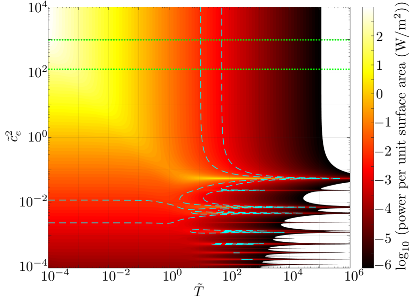
Figure 5: Tidal power as a function of non-dimensional time scale ( \tilde{T} ) and non-dimensional squared wave speed ( c_e^2 ) assuming potential energy is dissipated. The dotted green lines are limits for ocean depths between 50 and 400 km while the dashed cyan lines delimit the observationally inferred range described by Kvorka et al. (2018).
