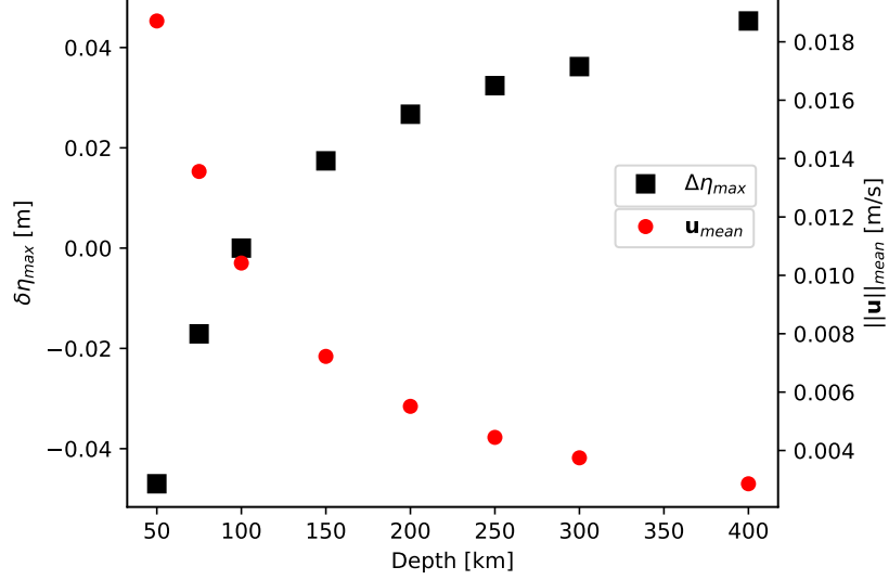
Figure 13: Spatially and temporally averaged speed (circles) for various depths, and maximum variation between the associated surface elevation and the elevation of a 100 km deep ocean (squares). For the same depth variation, the elevation and speed variations are larger for an ocean shallower than 100 km than for a deeper ocean. The larger the depth difference, the larger the elevation and speed variations.
