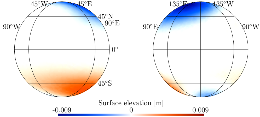
Figure 10: Ocean surface elevation generated by the heat flux predicted by Kvorka et al. (2018). It is at rest over most of the ocean, positive near the south pole and negative near the north pole and in a small area near the south pole. The area where the ocean surface elevation is positive is larger but the maximum is smaller than the absolute value of the minimum.
