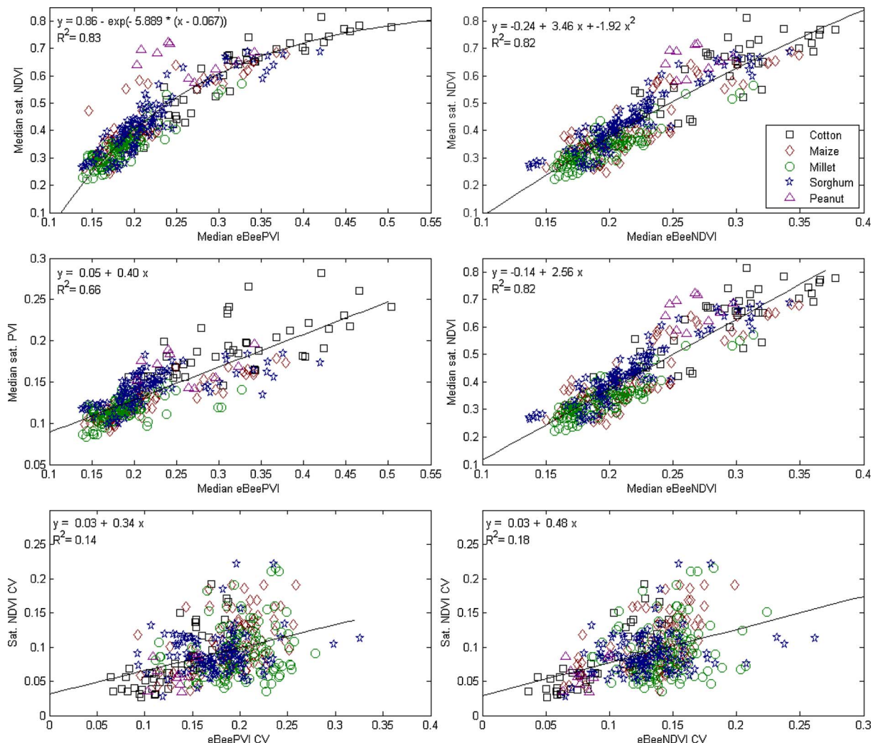
Fig. 5. Relationships between spatial coefficients of variation (CV, standard deviation/mean) and median eBeePVI / eBeeNDVI values for plots derived from 2014 UAV mosaics and WorldView-2 satellite images (PVI/NDVI).
