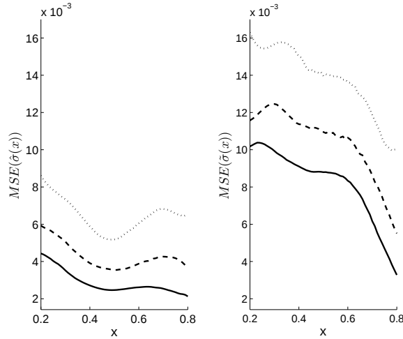
Figure 4: MSE of \hat{\sigma}(x) (left panel) and \tilde{\sigma}(x) (right panel) for samples of size n = 100 (dotted line), n = 200 (dashed line) and n = 400 (solid line).
