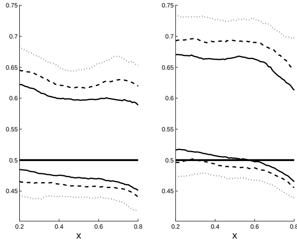
Figure 6: Quantiles of order 0.05 and 0.95 of the distribution of \hat{\sigma}(x) (left panel) and \tilde{\sigma}(x) (right panel) for samples of size n = 100 (dotted line), n = 200 (dashed line) and n = 400 (solid line).
