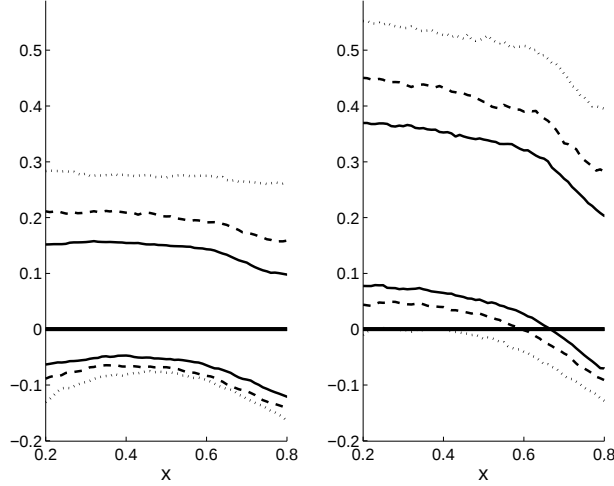
Figure 5: Quantiles of order 0.05 and 0.95 of the distribution of \hat{m}(x) - m(x) (left panel) and \tilde{m}(x) - m(x) (right panel) for samples of size n = 100 (dotted line), n = 200 (dashed line) and n = 400 (solid line).
