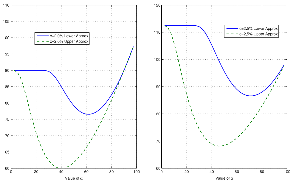
Fig. 8.2. Market value of debts as a function of \alpha .
