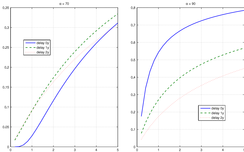
Fig. 8.3. Influence of a delay on probabilities of default (lower approximation).
