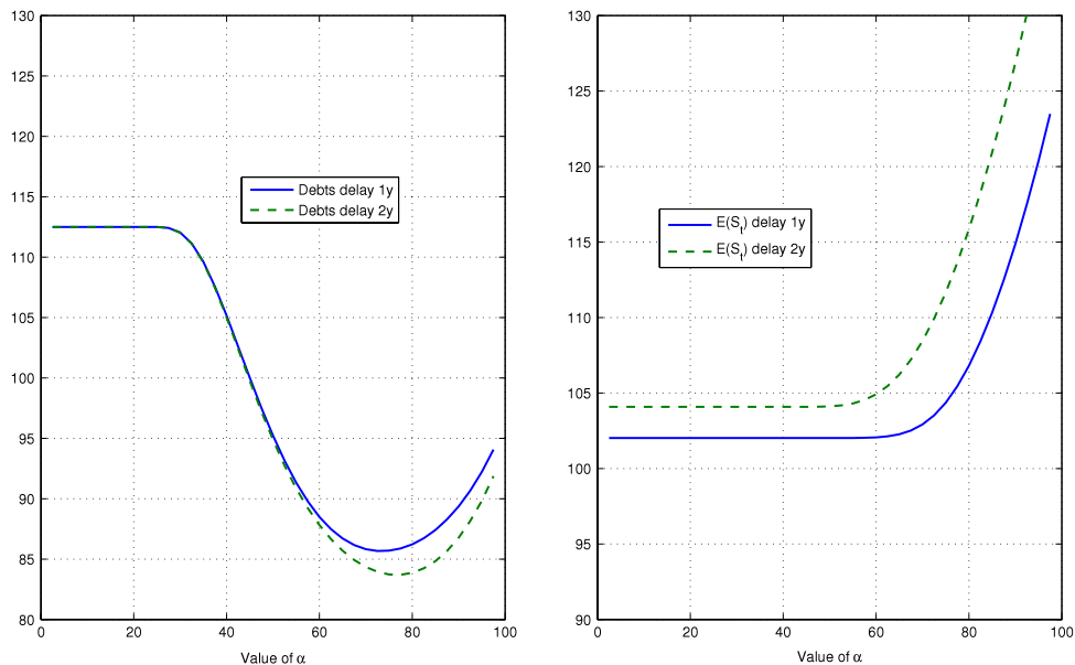
Fig. 8.4. Market values of debts and equity, in function of \alpha .
