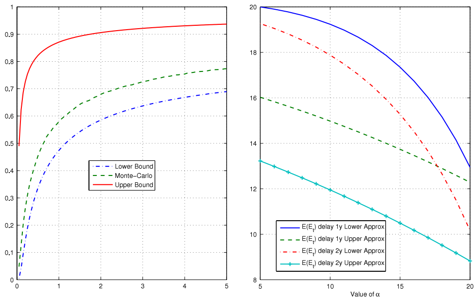
Fig. 8.5. Probabilities of default and expected equity.
