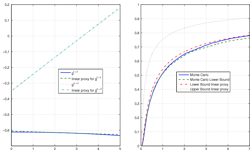
Fig. 8.1. Example of function (g^{l,c})^{-1}(t, \alpha) and default probabilities.
