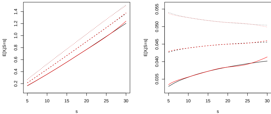
Fig. 4 Upper panel: Respective contributions s \mapsto E[X_i|S = s] for participant 1 (solid line appearing at the bottom), for a participant of type 2 (broken line appearing in the middle), and a participant of type 3 (dotted line appearing at the top). Black curves correspond to exact values. Red curves correspond to values obtained with the proposed approximation based on the first 3 moments. Lower panel: Respective relative contributions
