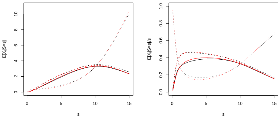
Fig. 3 Left panel: Respective contributions s \mapsto E[X_i|S = s] for participant 1 (solid line appearing at the bottom), participant 2 (broken line appearing in the middle), and participant 3 (dotted line appearing at the top). Black curves correspond to exact values. Red curves correspond to values obtained with the proposed approximation based on the first 3 moments, with h = -0.15 . Right panel: Respective relative contributions
