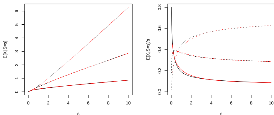
Fig. 1 Left panel: Respective contributions s \mapsto E[X_i | S = s] for participant 1 (solid line appearing at the bottom), participant 2 (broken line appearing in the middle), and participant 3 (dotted line appearing at the top). Black curves correspond to values obtained with Panjer algorithm. Red curves correspond to values obtained with the proposed approximation based on the first 3 moments (mean, variance and skewness). Right panel: Respective relative contributions
