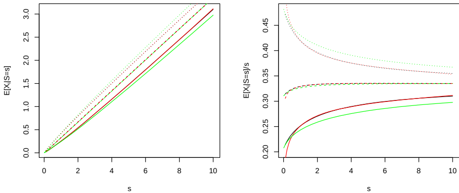
Fig. 2 Left panel: Respective contributions s \mapsto E[X_i|S = s] for participant 1 (solid line appearing at the bottom), participant 2 (broken line appearing in the middle), and participant 3 (dotted line appearing at the top). Black curves correspond to exact values. Red curves correspond to values obtained with the proposed approximation based on the first 3 moments. Green curves correspond to approximations obtained with Panjer algorithm. Right panel: Respective relative contributions
