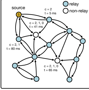
Fig. 3. Broadcast using counter-based controlled flooding, example with c = 2 , and details of counter and timer initial values for 4 sample nodes.
