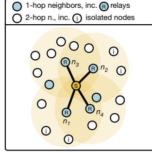
Fig. 4. MPR selection of overlay nodes: n_1 and n_2 are selected during the first phase as they connect to isolated nodes, n_3 and n_4 in the second phase as they allow to cover the most two-hop neighbors.
