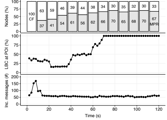
Fig. 9. Timeline of an overlay emergence, with the number of nodes using the two protocols (first plot), the average LBC for nodes inside the POI (second plot) and the average number of incoming messages (third plot).
