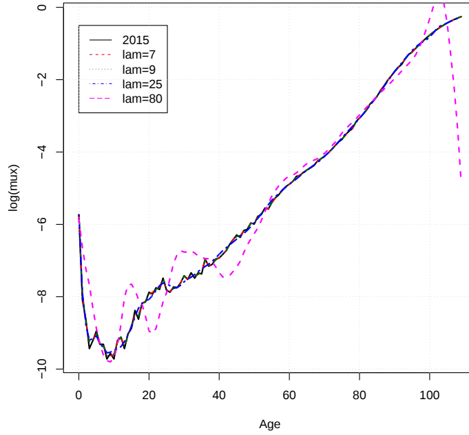
Figure 4: Smoothing with Lasso, year 2015. Comparison of smoothed curves for different penalty weights.
