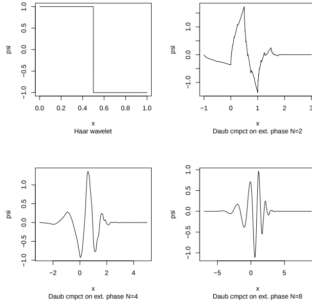
Figure 12: Daubechies wavelets with vanishing moments up to M=1, 2, 4, 8 . For M=1 , we retrieve the Haar wavelet.
