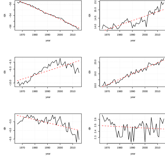
Figure 7: Time-series of coefficients of wavelets 1 to 6. The red dotted line is the linear regression.
