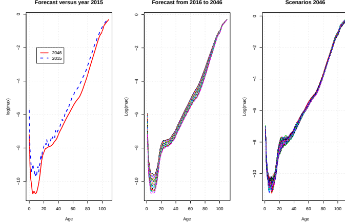
Figure 11: Left plot: log-forces of mortality in 2015 and 2046. Mid plot: Average log-forces of mortality from 2016 to 2046. Right plot: 1000 scenarios of log-mortality rates, year 2046.
