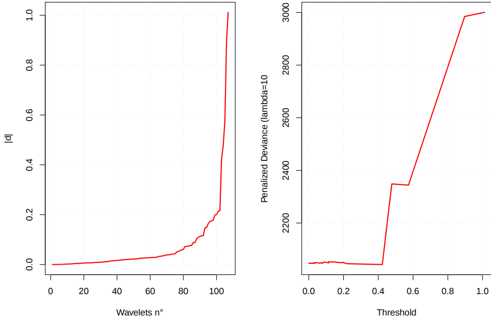
Figure 3: Smoothing with Lasso, year 2015. Left plot: series of thresholds, |\mathbf{d}| , sorted by ascending order. Right graph penalized deviances. Lasso parameter: \lambda = 10 .
