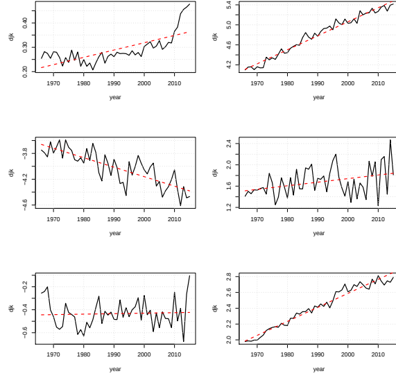
Figure 9: Time-series of coefficients of wavelets 13 to 18. The red dotted line is the linear regression.
