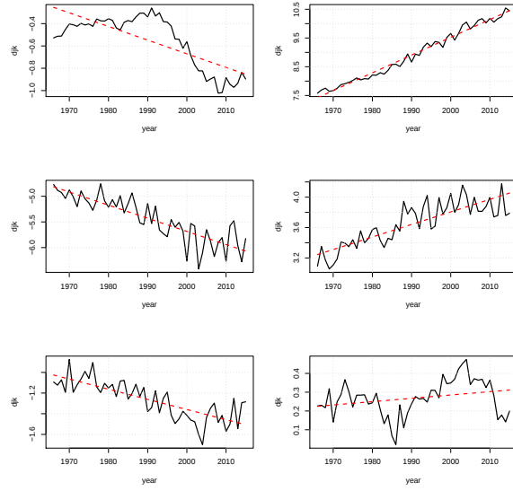
Figure 8: Time-series of coefficients of wavelets 7 to 12. The red dotted line is the linear regression.
