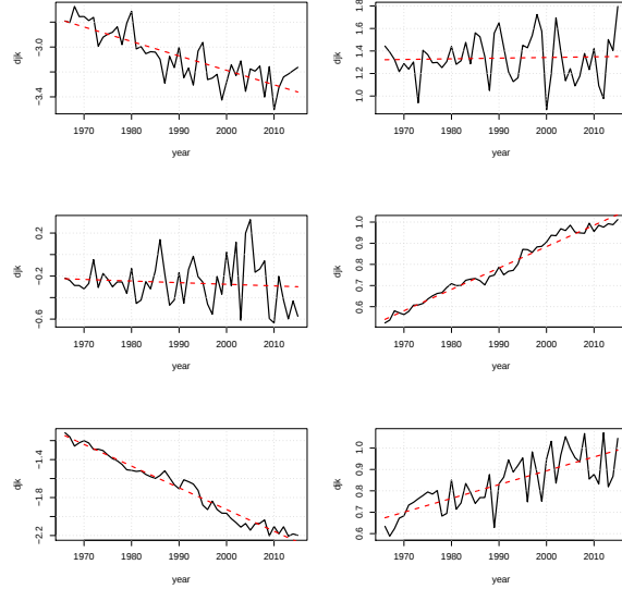
Figure 10: Time-series of coefficients of wavelets 19 to 24. The red dotted line is the linear regression.
