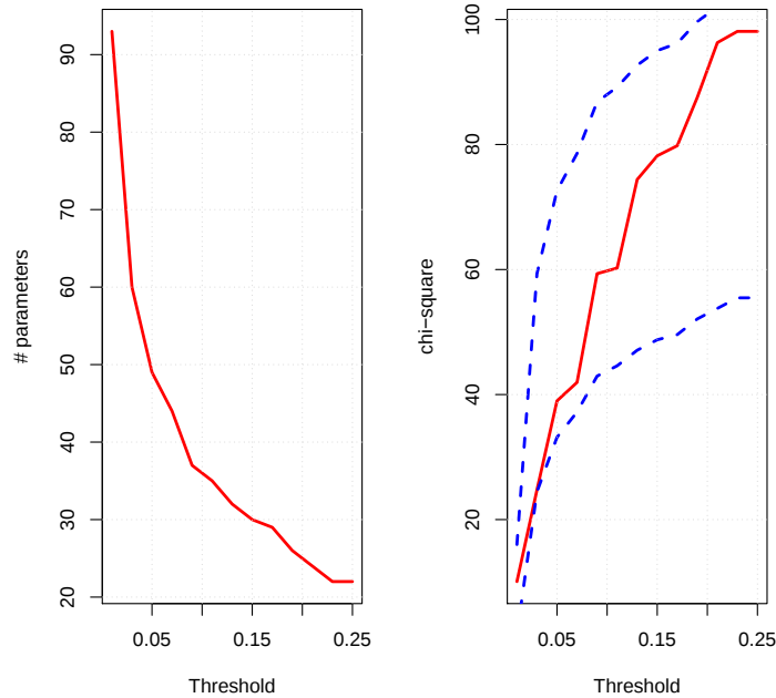
Figure 1: Belgian population, year 2015. Left and right plots respectively show the evolution of the number of non-null \hat{d}_{j,k} and Chi-Square statistics in function of the threshold d^* . In the right graph, blue lines correspond to the 2.5% and 97.5% Chi-Square quantiles with n - p - 1 degrees of freedom.
