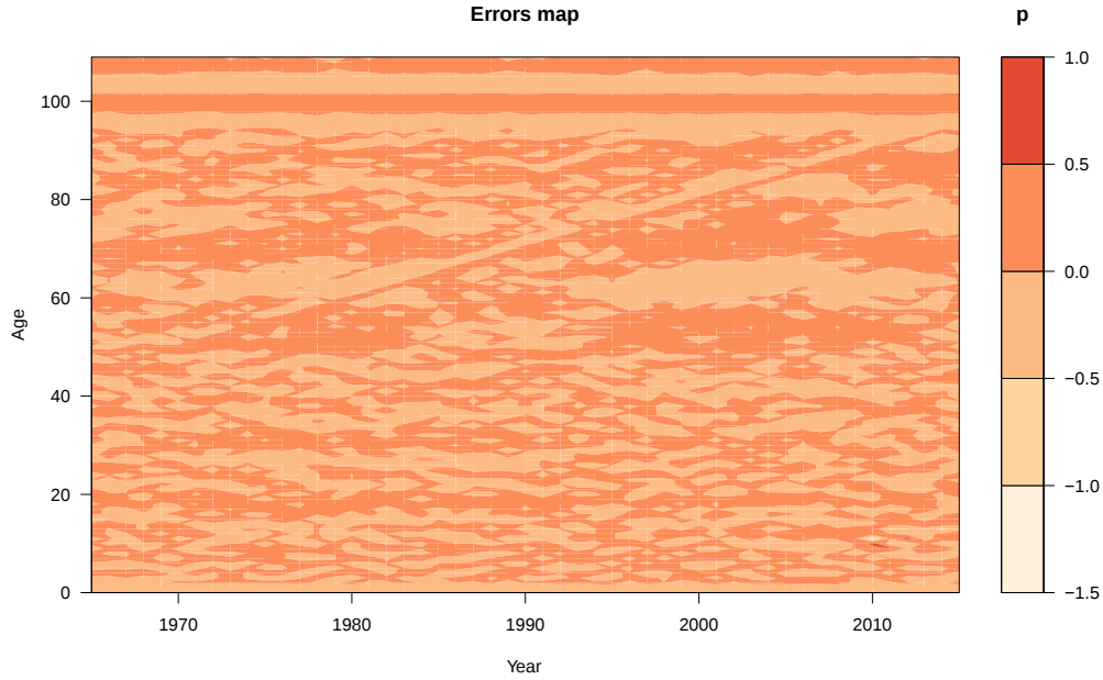
Figure 6: Heat-map of differences between smoothed and observed log-mortality rates.
