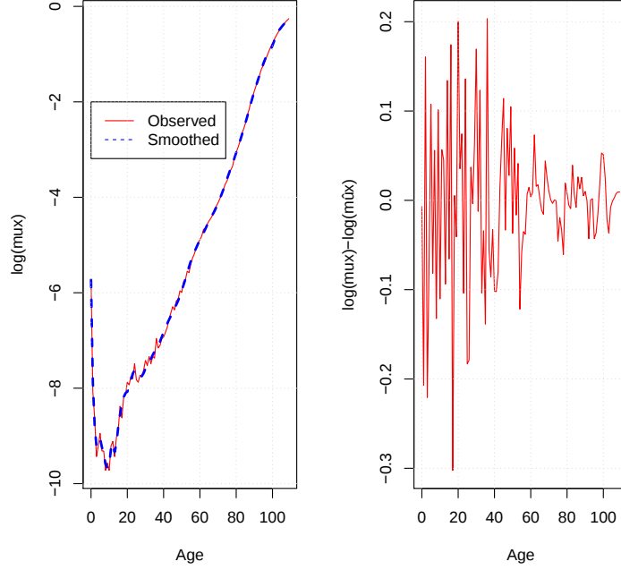
Figure 2: Belgian population, year 2015. The left plot shows the smoothed and original curves of log-forces of mortality. The right graph reports the spreads between observed and smoothed log-mortality rates.
