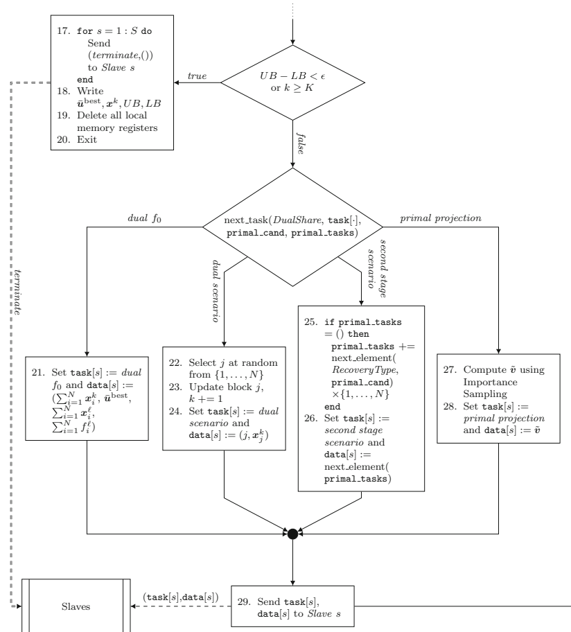
Fig. 5 Control flow of the Master process (cont.)
