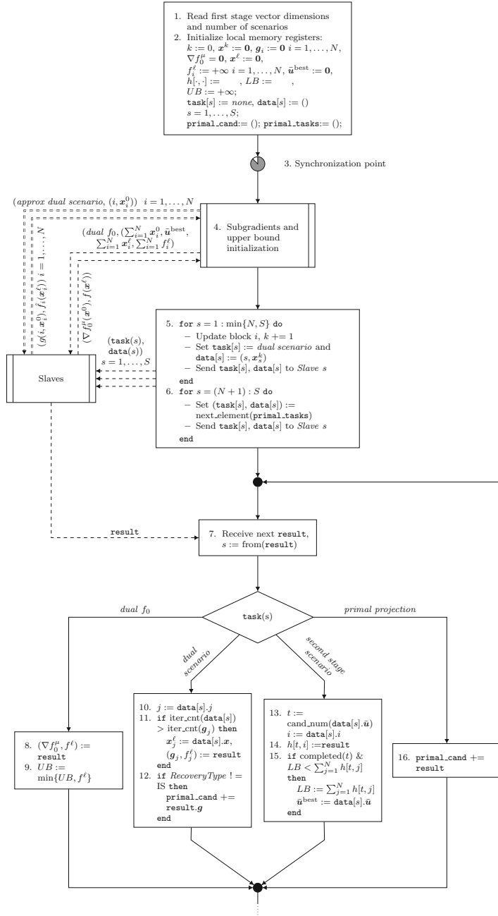
Fig. 4 Control flow of the Master process
