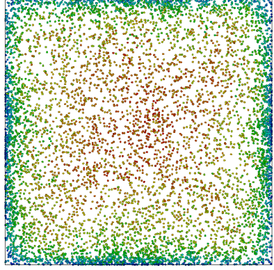
(b) Re_\tau = 600 , \rho_p/\rho = 1000 , F_{el}/F_g = 0.026
