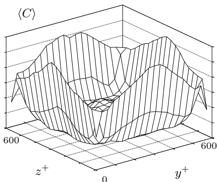
(a) Re_\tau = 600 , \rho_p/\rho = 1000 , F_{el}/F_g = 0
