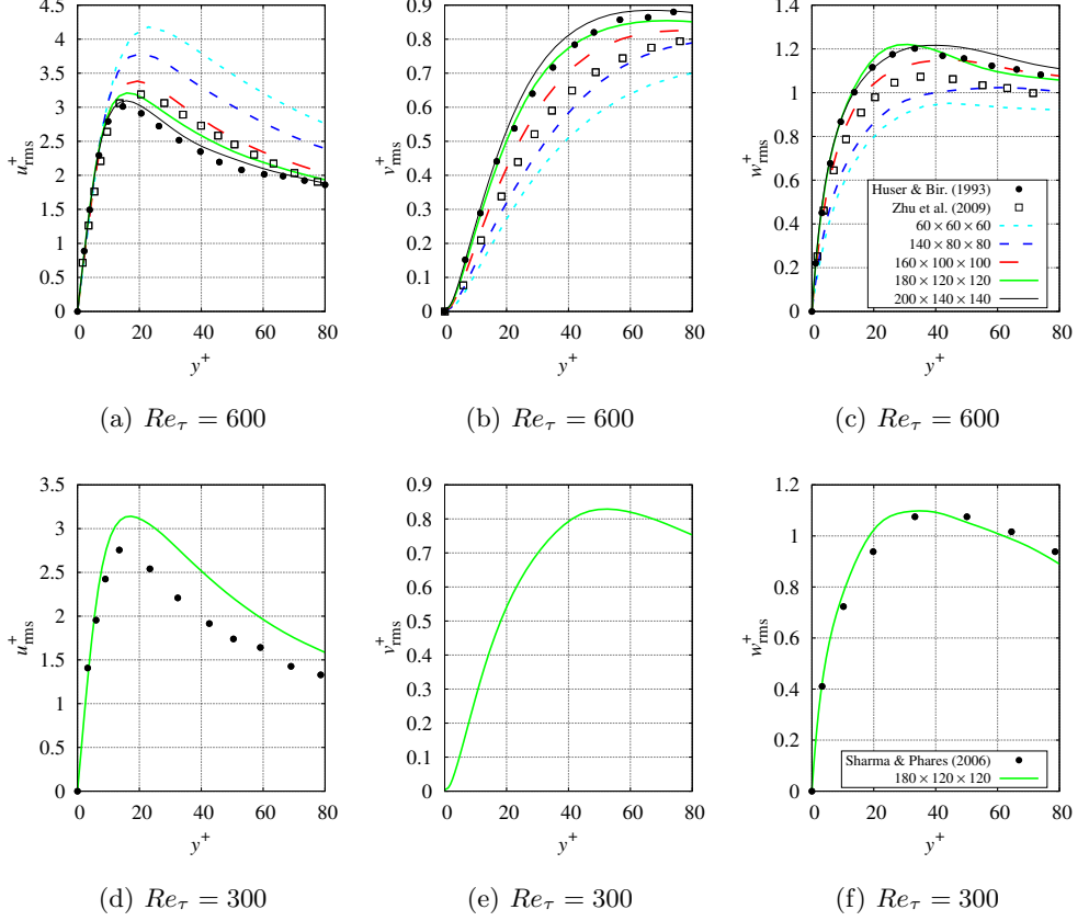
FIGURE 13. DNS of flow in a duct without particles. Comparison of the rms velocity components with the DNS data of Huser & Biringen (1993), Zhu et al. (2009), and Sharma & Phares (2006). The profiles for Re_\tau = 600 are computed on five different grid resolutions, as shown in the legend of the figure. Note that Sharma & Phares (2006) did not provide data for v_{\text{rms}}^+ .
