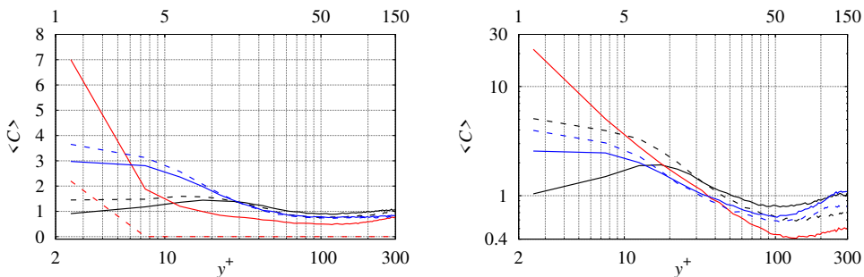
(c) Slice: 27.5 < z^+ < 30 Re_\tau = 300 and 55 < z^+ < 60 for Re_\tau = 600 . (d) Slice 147.5 < z^+ < 150 for Re_\tau = 300 and 295 < z^+ < 300 for Re_\tau = 600 .
