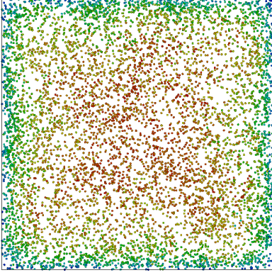
(a) Re_\tau = 600 , \rho_p/\rho = 1000 , F_{el}/F_g = 0
