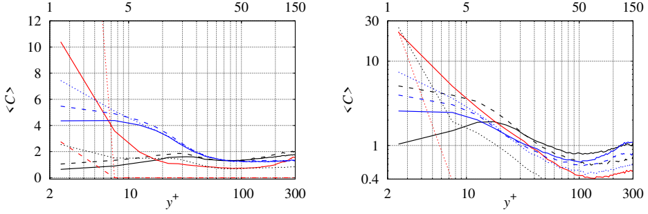
(a) Slice: 10 < z^+ < 12.5 for Re_\tau = 300 and 20 < z^+ < 25 for Re_\tau = 600 . (b) Slice 147.5 < z^+ < 150 for Re_\tau = 300 and 295 < z^+ < 300 for Re_\tau = 600 .
