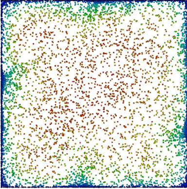
(c) Re_\tau = 300 , \rho_p/\rho = 1000 , F_{el}/F_g = 0
