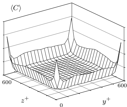
(f) Re_\tau = 600 , \rho_p/\rho = 7500 , F_{el}/F_g = 0.004
