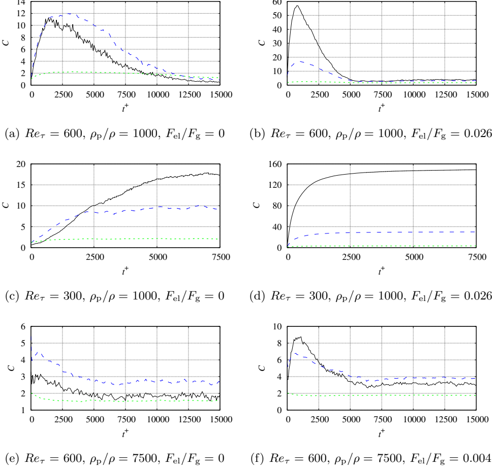
FIGURE 4. Temporal evolution of the normalized particle number density C near the walls.
