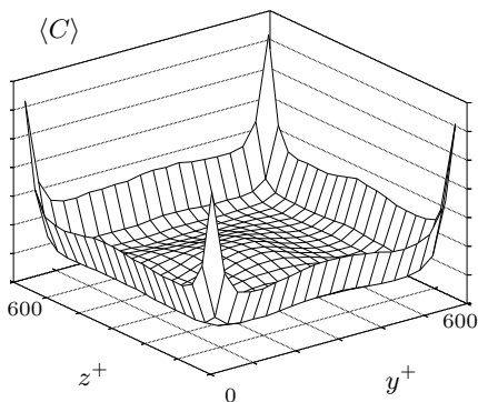
(e) Re_\tau = 600 , \rho_p/\rho = 7500 , F_{el}/F_g = 0
