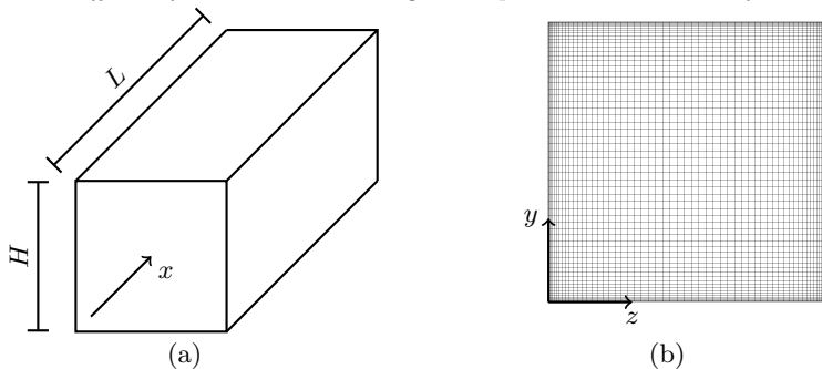
FIGURE 3. (a) Graphic representation and dimensions of the flow domain. The arrow points to the direction of the flow. (b) Computational mesh in the cross section, consisting of 60 \times 60 cells.
