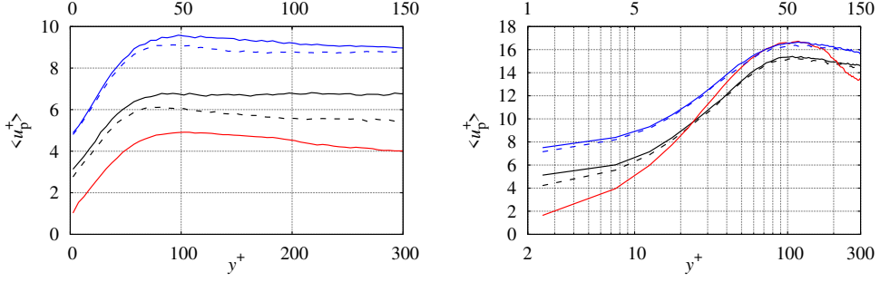
(a) Slice: 2.5 < z^+ < 5 for Re_\tau = 300 and 5 < z^+ < 10 for Re_\tau = 600 . (b) Slice: 22.5 < z^+ < 25 for Re_\tau = 300 and 45 < z^+ < 50 for Re_\tau = 600 .
