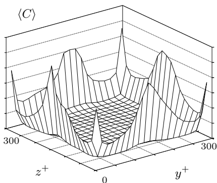
(c) Re_\tau = 300 , \rho_p/\rho = 1000 , F_{el}/F_g = 0
