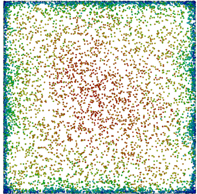
(f) Re_\tau = 600 , \rho_p/\rho = 7500 , F_{el}/F_g = 0.004
