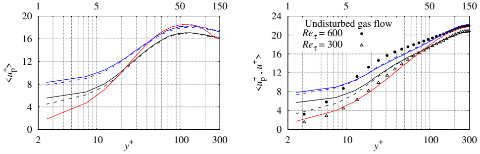
(c) Slice: 35 < z^+ < 37.5 for Re_\tau = 300 and 70 < z^+ < 75 for Re_\tau = 600 . (d) Slice: 147.5 < z^+ < 150 for Re_\tau = 300 and 295 < z^+ < 300 for Re_\tau = 600 .
