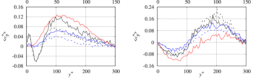
(a) Slice: 2.5 < z^+ < 5 for Re_\tau = 300 and 5 < z^+ < 10 for Re_\tau = 600 .
