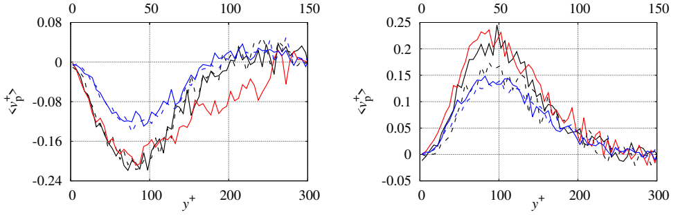
(c) Slice: 35 < z^+ < 37.5 for Re_\tau = 300 and 70 < z^+ < 75 for Re_\tau = 600 .
