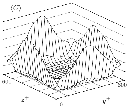
(b) Re_\tau = 600 , \rho_p/\rho = 1000 , F_{el}/F_g = 0.026
