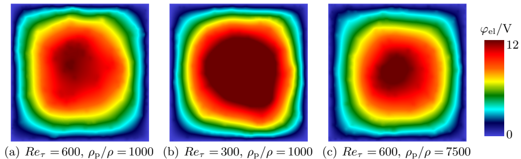
FIGURE 9. Instantaneous snapshots of the electric potential across the cross-section of the duct, induced by charges carried by the particles.
