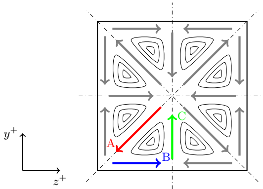
FIGURE 1. Symmetry planes of the duct and streamlines of the induced Prandtl's secondary flow of the second kind. The arrows indicate the direction of the possible particle motion in the cross-section following the gas phase.
