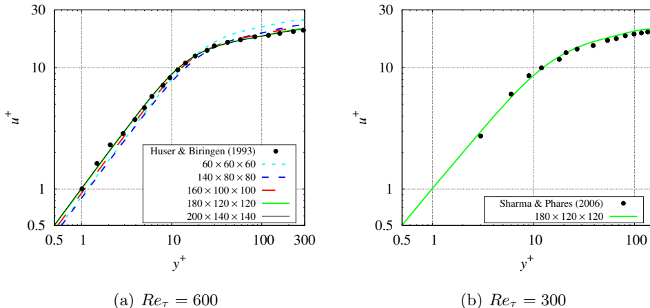
FIGURE 12. DNS of flow in a duct without particles. Comparison of the mean streamwise velocity at the centre plane of the duct with the DNS data of Huser & Biringen (1993) and Sharma & Phares (2006). The profiles for Re_\tau = 600 are computed on five different grid resolutions, as shown in the legend of the figure.
