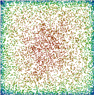
(e) Re_\tau = 600 , \rho_p/\rho = 7500 , F_{el}/F_g = 0
