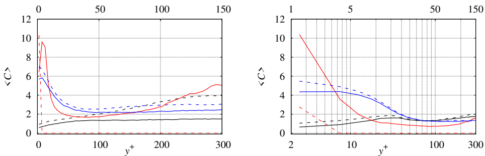
(a) Slice: 2.5 < z^+ < 5 for Re_\tau = 300 and 5 < z^+ < 10 for Re_\tau = 600 . (b) Slice: 10 < z^+ < 12.5 for Re_\tau = 300 and 20 < z^+ < 25 for Re_\tau = 600 .
