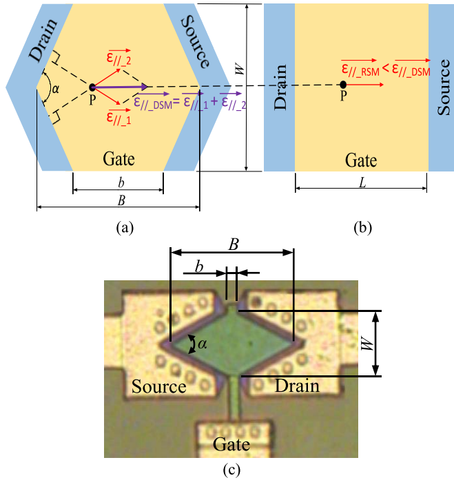
FIGURE 1. Schematic layouts of a DSM (a) and its RSM counterpart (b), illustrating their LEF components ( \vec{E}_{//1} and \vec{E}_{//2} ), with same A_G , W and bias conditions. Besides, in (c) is illustrated a photograph of a Diamond SOI MOSFET manufactured ( \alpha = 90^\circ ).
