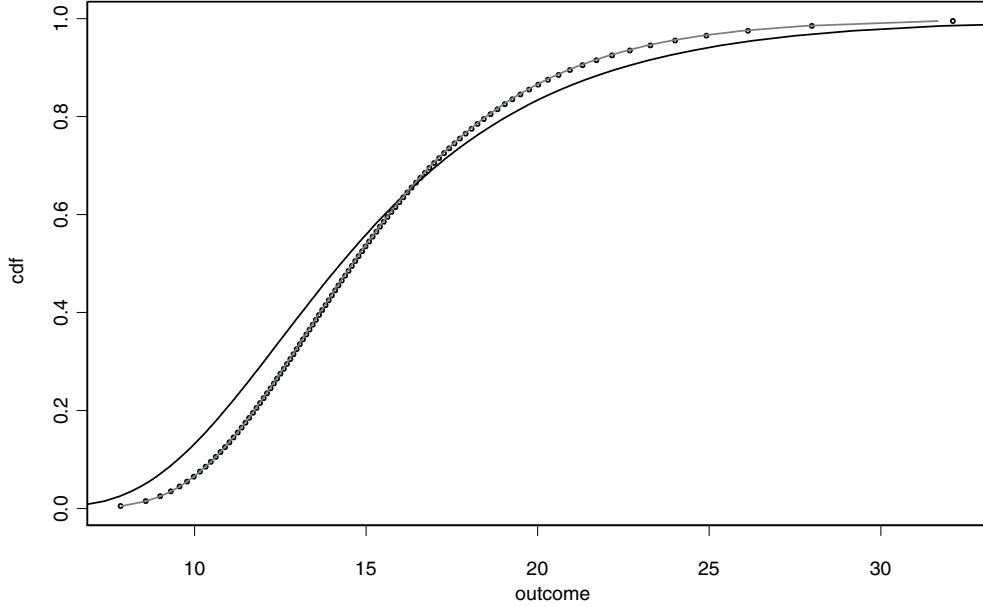
Figure 7: The cdf's of S_\infty (dotted line), S_\infty^l (solid grey line) and S_\infty^c (solid black line).
