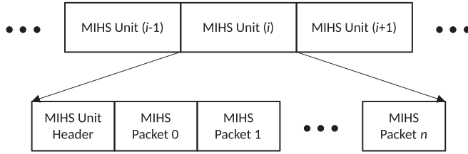
Fig. 8. MIHS packetization.
