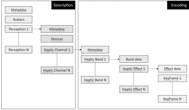
Fig. 4. Data structure.
