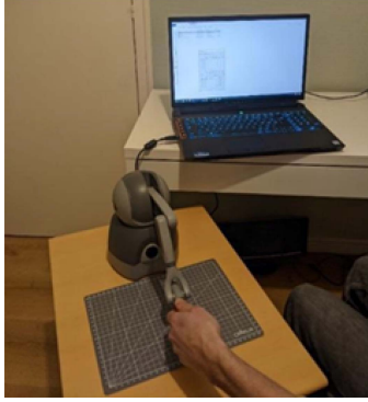
Fig. 12. Kinesthetic evaluation platform with the geomagic touch stylus held with the non-dominant hand.
