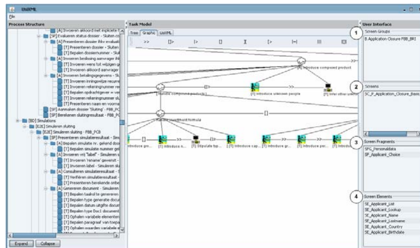
Fig. 2 Prototype of Usi4Biz showing business process, task model and UI components.
