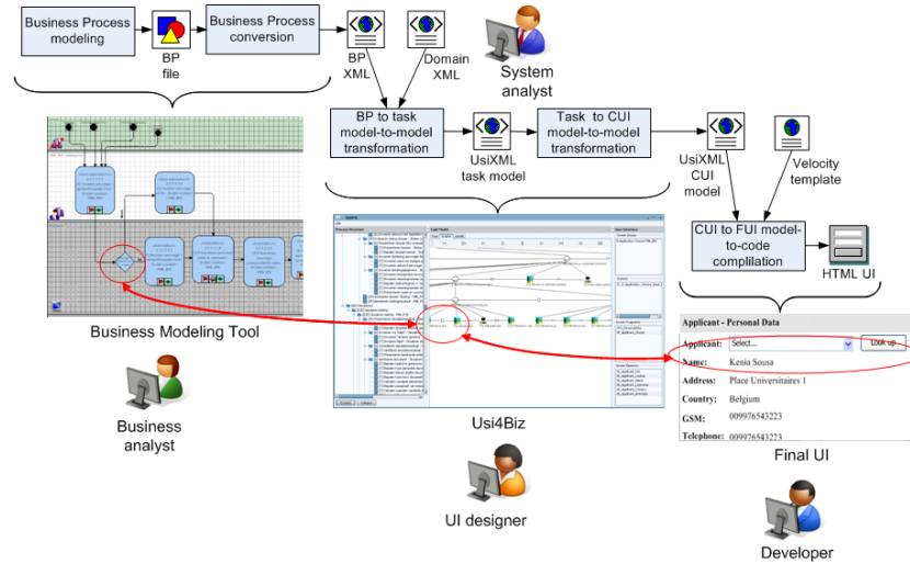
Fig. 1 Outline of the method with roles, artifacts and tools.
