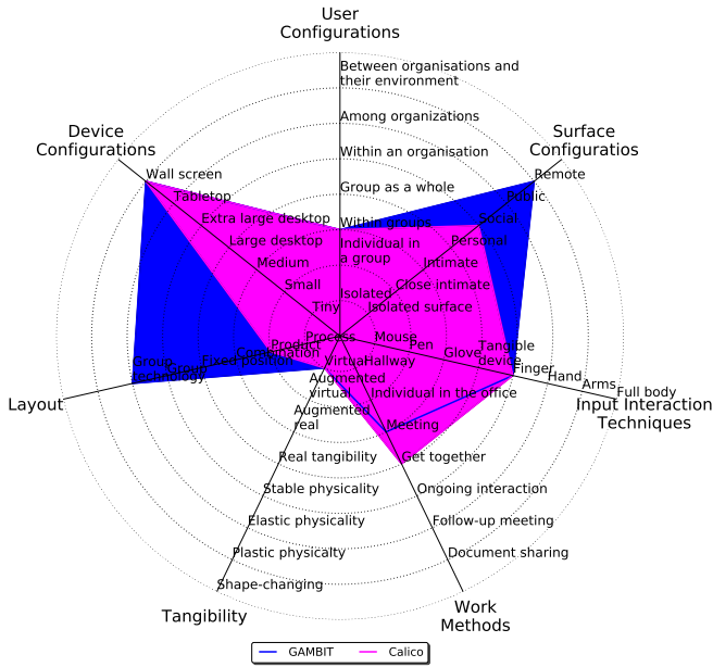
Fig. 9. CROSSIDE instantiation for CALICO superimposed to the instantiation for GAMBIT.
