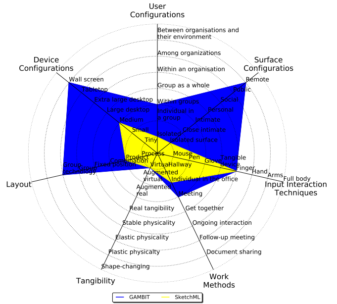
Fig. 10. CROSSIDE instantiation for SKETCHML superimposed to the instantiation for GAMBIT.
