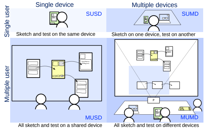
Fig. 5. Quadrant of the four configurations.
