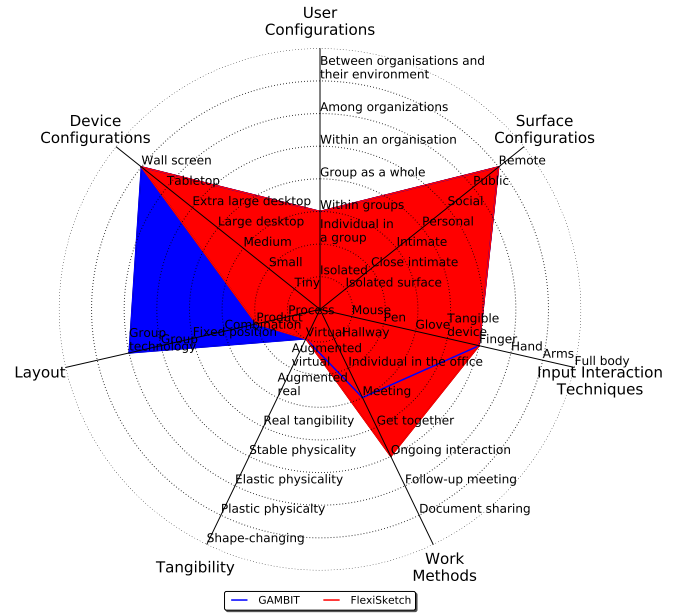
Fig. 8. CROSSIDE instantiation for FLEXISKETCH on GAMBIT.
