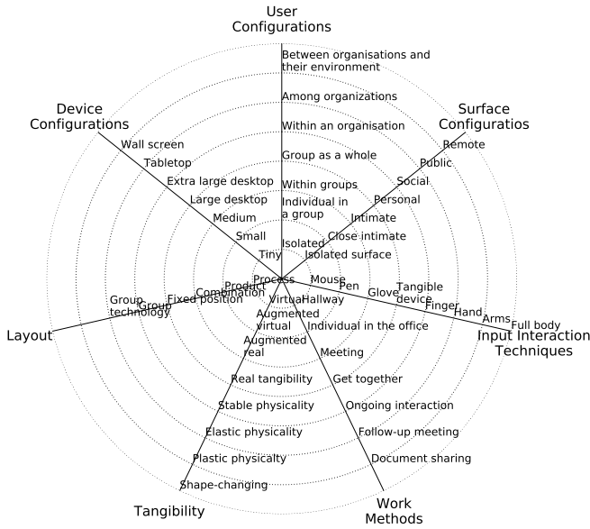
Fig. 1. A design space for Cross-Surface Collaboration by Sketching.
