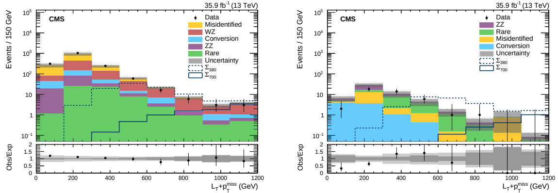
Figure 1: The L_T + p_T^{\text{miss}} distribution for events with three leptons and one OSSF pair with mass above-Z (left) and the L_T + p_T^{\text{miss}} distribution for events with four or more leptons and one OSSF pair (right). The total SM background is shown as a stacked histogram of all contributing processes. The predictions for signal models (sum of all production and decay modes) with m_\Sigma = 700 \text{ GeV} (solid line) and m_\Sigma = 380 \text{ GeV} (dashed line) are also shown. The lower panels show the ratio of observed to expected events. The hatched gray band in the upper panel, and the dark and light gray bands in the lower panel represent the total, statistical, and systematic uncertainties in the expected background, respectively.
