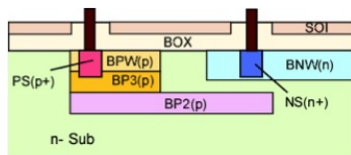
Normal Process for n- substrate
