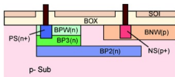
Reverse Process for p- substrate
