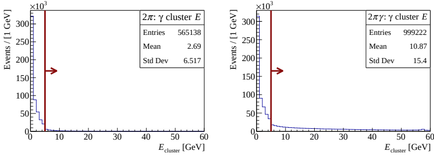
Figure 4.42: Left: Energy of additional LKr clusters in A' \rightarrow \pi^+\pi^- decay which can promote the event to an h^+h^-\gamma topology. Right: Energy of LKr clusters not associated to \pi in a \rightarrow \pi^+\pi^-\gamma decay. The energy limit on photon association is indicated by the red line.
