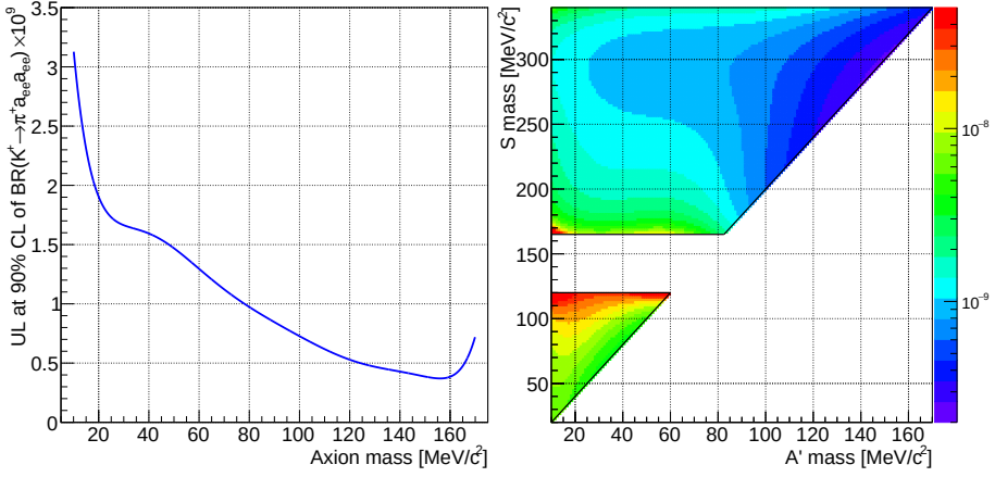
Figure 2.23: Left: Bound on the axion \text{BR}_{K^+ \rightarrow \pi^+ aa} as a function of m_a . Right: Bound on the BR of the K^+ \rightarrow \pi^+ S , S \rightarrow A' A' , A' \rightarrow e^+ e^- decay chain as a function of the dark scalar and dark photon masses [156].
