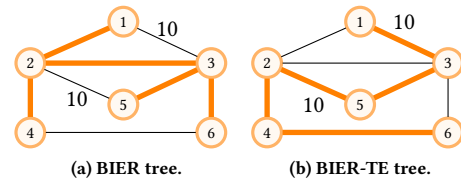
Figure 1: Small network topology with 6 nodes.
