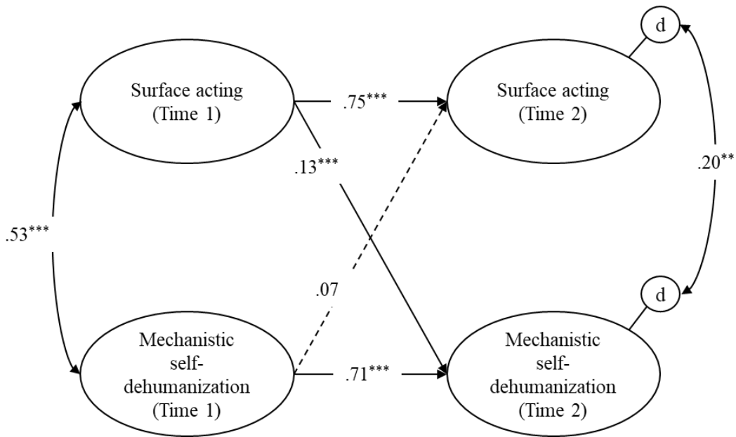
Figure 3. Study 3: Structural equation model of the relationships between surface acting and self-dehumanization over time ( N = 436 ). Dashed lines indicated non-significant paths.
