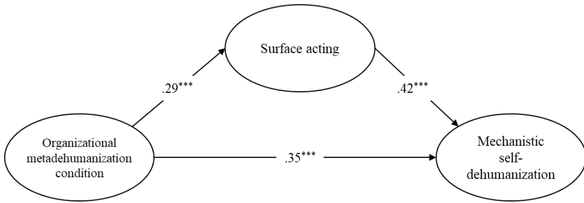
Figure 2. Study 2: Completely standardized coefficients for the mediation model ( N = 200 ).
