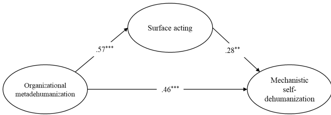
Figure 1. Study 1: Completely standardized coefficients for the mediation model ( N = 341 ).
