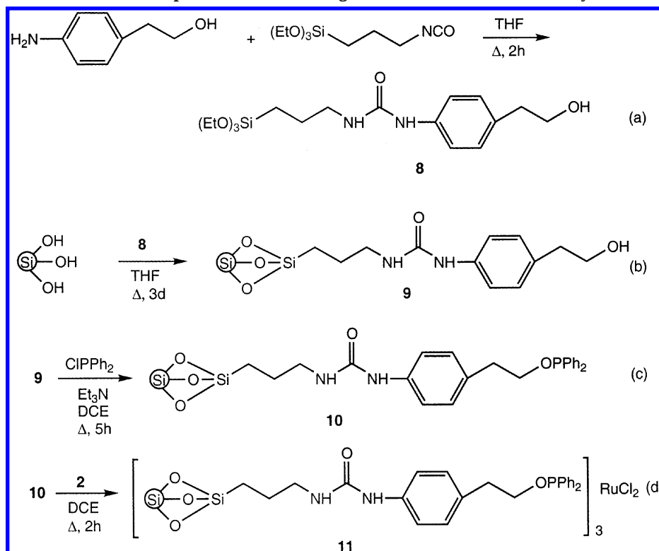
Scheme 3. Preparation of Heterogenized Monodentate Catalyst 11
