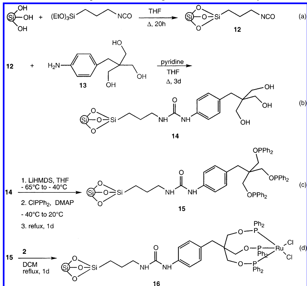
Scheme 4. Preparation of Heterogenized Tridentate Catalyst 16
