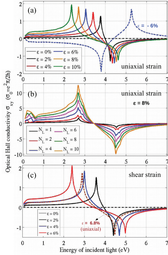
Figure 3. Optical Hall conductivity in monolayer graphene with different strains ((a) and (c)) and in few-layer systems (b). Uniaxial ( \theta = 90^\circ )/shear ( \theta = 45^\circ ) strains are applied in ((a)–(c)), respectively. The light polarization is fixed to \phi = -45^\circ .
