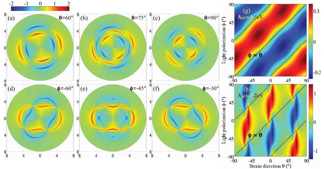
Figure 4. Optical Hall conductivity in monolayer graphene with respect to the light energy \hbar\omega ( >0 and in eV) and polarization \phi , and the strain direction \theta . The polar axis of (a)–(f) presents the energy \hbar\omega while the azimuthal direction indicates the angles \phi in (a)–(c) and \theta in (d)–(f). The dashed lines in ((g) and (h)) indicate the cases \phi - \theta = n\pi/2 . The amplitude of uniaxial strain is fixed to \epsilon = 8\% .
