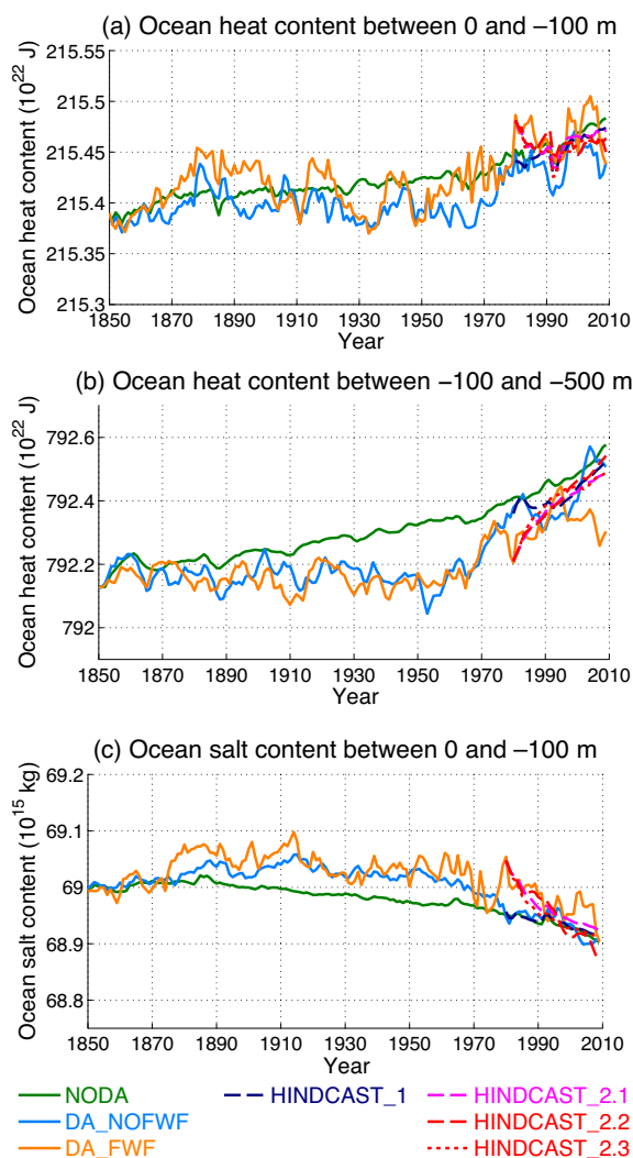
Figure 4. Ensemble mean of yearly mean (a) ocean heat content in the first 100 m below the surface, (b) ocean heat content between -100 and -500 m and (c) ocean salt content in the first 100 m below the surface, for the simulations summarised in Table 1. The ocean heat and salt contents are computed south of 60^\circ S. The ocean heat content is computed against absolute zero.
