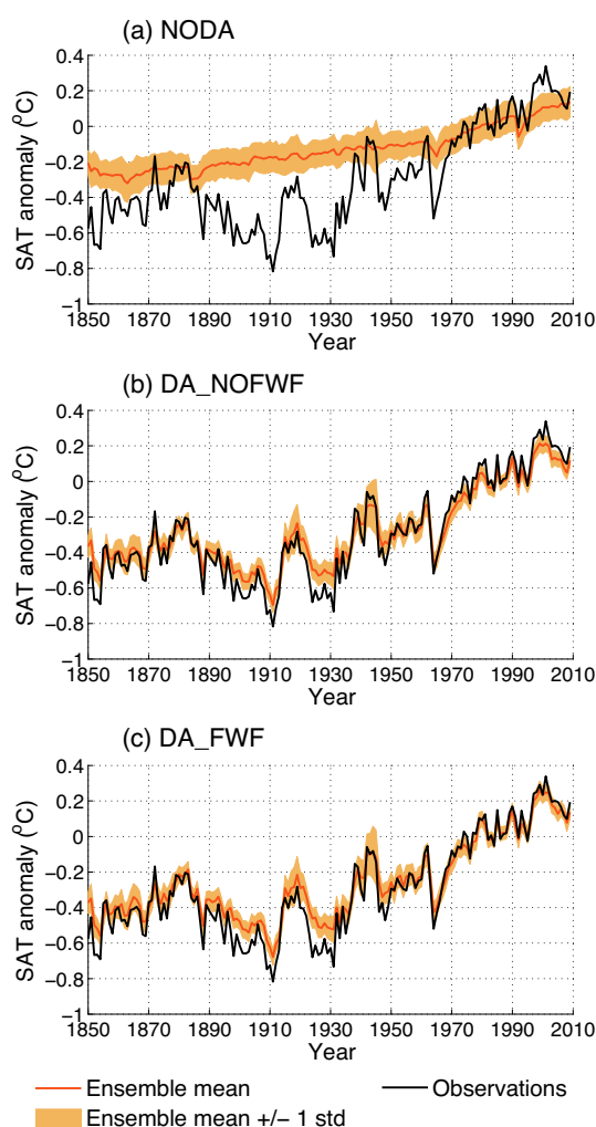
Figure 5. Yearly mean surface air temperature anomalies with regard to 1961–1990, averaged over the area south of 30^\circ S, from (a) the model simulation without data assimilation (NODA), (b) the model simulation that assimilates anomalies of surface air temperature (DA_NOFWF) and (c) the model simulation that assimilates anomalies of surface air temperature and that is forced by an additional autoregressive freshwater flux following Eq. (1) (DA_FWF). The model ensemble mean is shown as the orange line, surrounded by one standard deviation shown as the light orange shading. Observations (Brohan et al., 2006) are shown as the black line.
