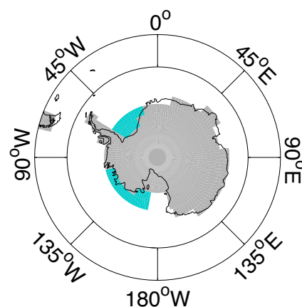
Figure 1. Spatial distribution of the additional freshwater flux included in model simulations (shaded blue). The shaded grey areas correspond to the land mask of the ocean model.
