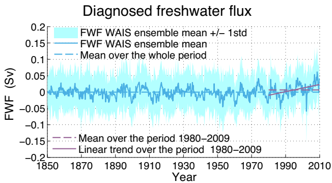
Figure 6. Freshwater flux from the model simulation with data assimilation and additional autoregressive freshwater flux following Eq. (1) (DA_FWF). The ensemble mean is shown as the blue solid line, surrounded by one standard deviation shown as the light blue shading. The dashed blue (purple) line shows the mean over the period 1850–2009 (1980–2009). The linear fit between 1980 and 2009 is shown as the solid purple line.
