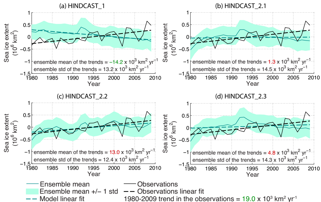
Figure 7. Yearly mean sea ice extent anomalies with regard to 1980–2009, for the four hindcast simulations initialised on 1 January 1980 through data assimilation (see Table 1 for details). The model ensemble mean is shown as the dark green line, surrounded by one standard deviation shown as the light green shading. Observations (Comiso, 1999) are shown as the black line. The green (black) dashed line shows the linear fit of the model simulation (observations). The values of the trend indicated in each panel correspond to the ensemble mean of the trends, computed over the period 1980–2009, along with the ensemble standard deviation. Trends that are (non-)significant at the 99 % level are shown in green (red).
