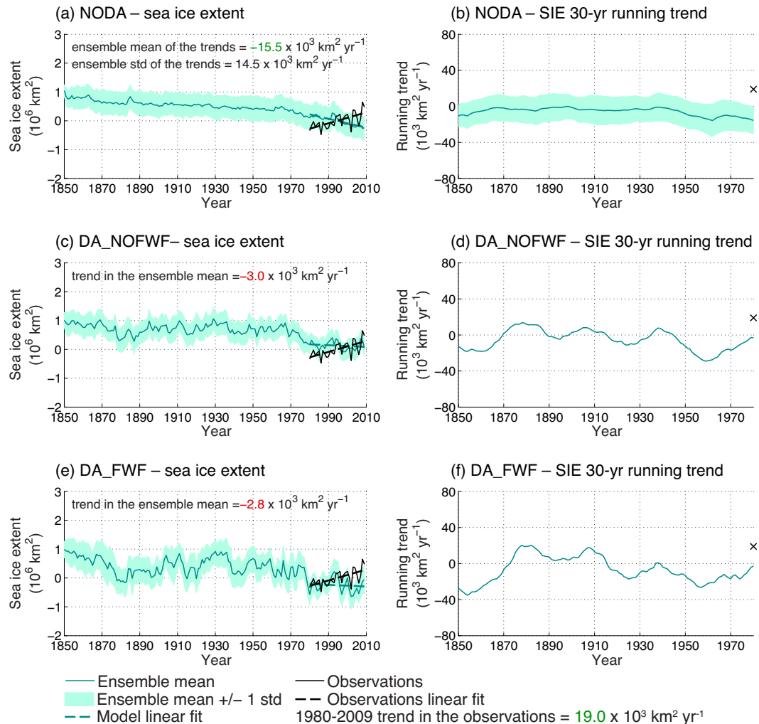
Figure 2. (a, c, e) Yearly mean sea ice extent anomalies with regard to 1980–2009 and (b, d, f) 30-year running trend in sea ice extent. Results are from (a, b) the simulation without data assimilation (NODA), (c, d) the model simulation that assimilates anomalies of surface air temperature (DA_NOFWF) and (e, f) the model simulation that assimilates anomalies of surface air temperature and that is forced by an additional autoregressive freshwater flux following Eq. (1) (DA_FWF). The model ensemble mean is shown as the dark green line surrounded by one standard deviation shown as the light green shading. Observations (Comiso, 1999) are shown as the black line (cross) in (a, c, e) (in b, d, f). The green (black) dashed line shows the linear fit of the model simulation (observations) in (a, c, e). The values of the trend indicated in (a, c, e) correspond to the ensemble mean of the trends, computed over the period 1980–2009, along with the ensemble standard deviation for NODA. Trends that are (non-)significant at the 99 % level are shown in green (red).
