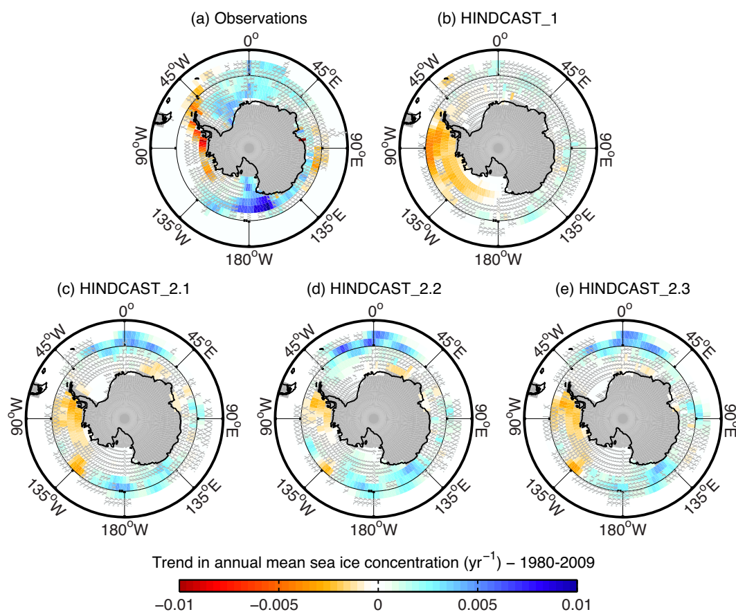
Figure 8. Trend in yearly mean sea ice concentration between 1980 and 2009, for (a) the observations (Comiso, 1999) and (b, c, d, e) the four hindcast simulations initialised on 1 January 1980 through data assimilation (see Table 1 for details). Hatched areas highlight the grid cells where the trend is not significant at the 99 % level. The shaded grey areas correspond to the land mask of the ocean model.
