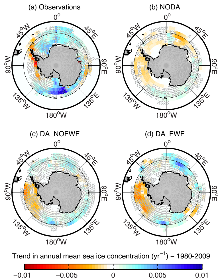
Figure 3. Trend in yearly mean sea ice concentration between 1980 and 2009, shown for (a) the observations (Comiso, 1999), (b) the model simulation without data assimilation (NODA), (c) the model simulation that assimilates anomalies of surface air temperature (DA_NOFWF) and (d) the model simulation that assimilates anomalies of surface air temperature and that is forced by an additional autoregressive freshwater flux following Eq. (1) (DA_FWF). Hatched areas highlight the grid cells where the trend is not significant at the 99 % level. The shaded grey areas correspond to the land mask of the ocean model.
