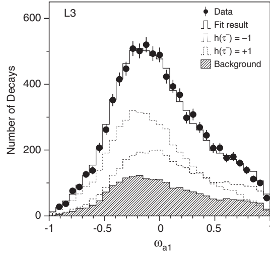
Fig. 4.5. The measured spectrum of the polarisation-sensitive variable \omega_{a_1} , described in the text, for the \tau \rightarrow a_1 \nu decays in the L3 experiment. The distributions for both a_1^- \rightarrow \pi^- \pi^+ \pi^- and a_1^- \rightarrow \pi^- \pi^0 \pi^0 decays are combined in this figure. The two helicity components and the background are shown separately.
