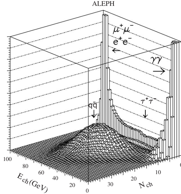
Fig. 2.1. Experimental separation of the final states using only two variables, the sum of the track momenta, E_{\text{ch}} , and the track multiplicity, N_{\text{ch}} , in the central detector of the ALEPH experiment.
