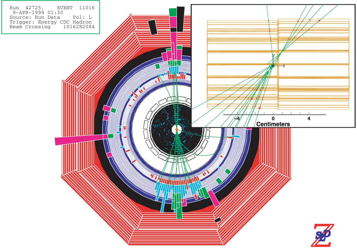
Fig. 1.8. Front view of an event classified as Z \rightarrow b\bar{b} . The displaced secondary vertex is visible in the expanded side view ( r - z view) of the beam interaction point.
