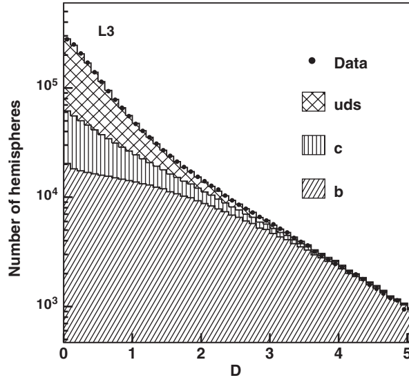
Fig. 5.2. Impact parameter b-tag from L3 [124]. D is the negative logarithm of the hemisphere impact parameter probability.
