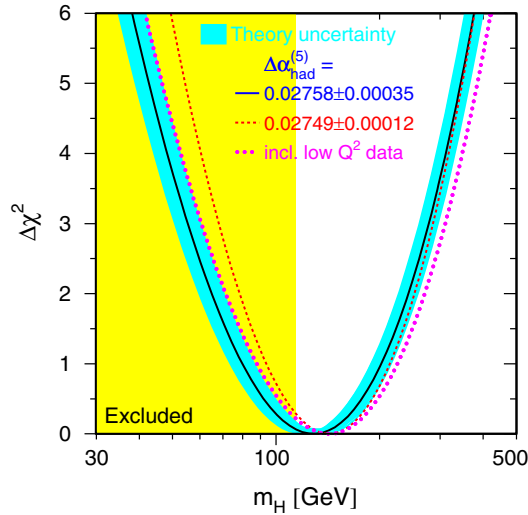
Fig. 8.13. \Delta\chi^2(m_H) = \chi_{\text{min}}^2(m_H) - \chi_{\text{min}}^2 as a function of m_H . The line is the result of the fit using all 18 results. The associated band represents the estimate of the theoretical uncertainty due to missing higher-order corrections as discussed in Section 8.4. The vertical band shows the 95% confidence level exclusion limit on m_H of 114.4 GeV derived from the direct search at LEP-II [39]. The dashed curve is the result obtained using the theory-driven \Delta\alpha_{\text{had}}^{(5)}(m_Z^2) determination of Eq. (8.4). The direct measurements of m_W and \Gamma_W used here are preliminary.
