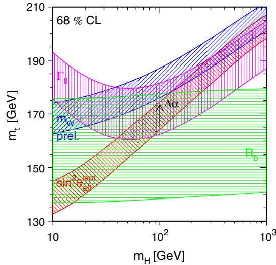
Fig. 8.3. Constraints on m_t and m_H from measurements of R_b^0 , \Gamma_{\ell\ell} , \sin^2 \theta_{\text{eff}}^{\text{lept}} and m_W . Each band gives the \pm 1\sigma constraint from the indicated measurement. The parametric uncertainty due to the uncertainty in the hadronic vacuum polarisation, \Delta\alpha_{\text{had}}^{(5)}(m_Z^2) = 0.02758 \pm 0.00035 , is not included in the width of these bands as it is small except for the \sin^2 \theta_{\text{eff}}^{\text{lept}} band, where the \pm 1\sigma uncertainty is indicated by the arrow labeled \Delta\alpha . The direct measurement of m_W used here is preliminary.
