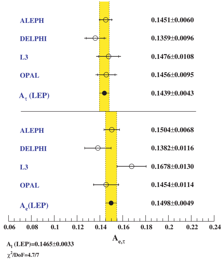
Fig. 4.8. Measurements of \mathcal{A}_{\tau} and \mathcal{A}_e from the four LEP experiments. The error bars indicate the quadrature sum of the statistical and systematic errors. The magnitude of the statistical error alone is indicated by the small tick marks on each error bar. The value of \mathcal{A}_{\ell} and the \chi^2 of the fit assuming lepton universality are also quoted.
