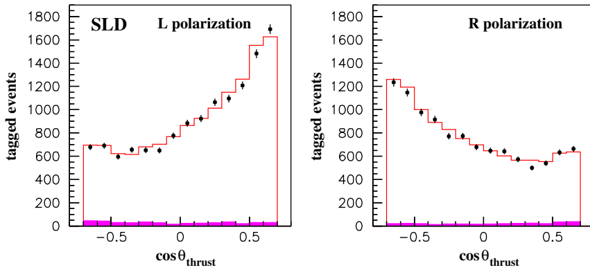
Fig. 5.11. Reconstructed \cos \theta distributions from the SLD vertex charge \mathcal{A}_b analysis for events with left-handed and right-handed electron beam polarisations. The shaded region corresponds to udsc background in the sample estimated from Monte Carlo.
