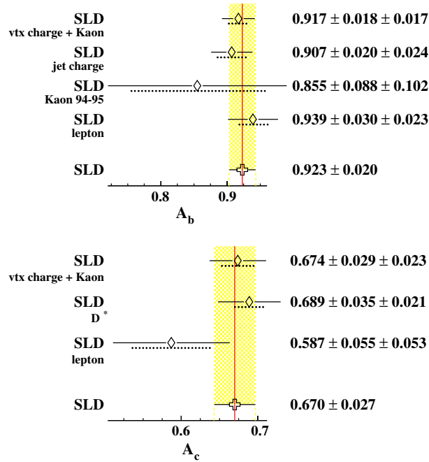
Fig. 5.15. \mathcal{A}_b and \mathcal{A}_c measurements used in the heavy flavour combination, corrected for their dependence on parameters evaluated in the multi-parameter fit described in the text. The dotted lines indicate the size of the systematic error.
