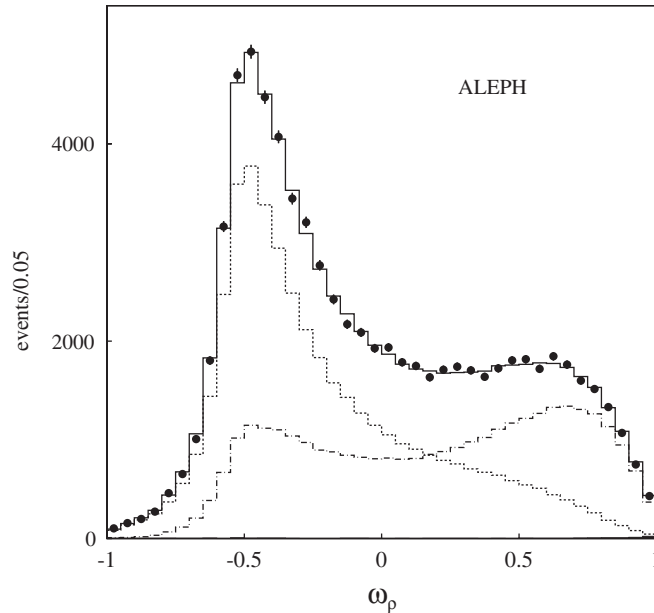
Fig. 4.4. The measured spectrum of the polarisation-sensitive variable \omega_\rho , described in the text, for the \tau \rightarrow \rho \nu decays in the ALEPH experiment. The dashed and dashed-dotted lines correspond to the contributions of negative and positive helicity \tau 's, respectively. The small shaded area near \omega = 1 is the non- \tau background contribution.
