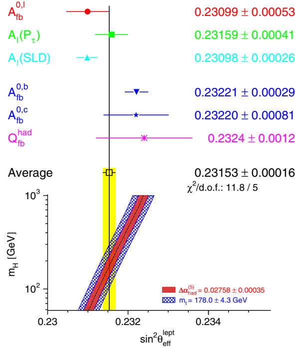
Fig. 7.6. Comparison of the effective electroweak mixing angle \sin^2 \theta_{\text{eff}}^{\text{lept}} derived from measurements depending on lepton couplings only (top) and also quark couplings (bottom). Also shown is the SM prediction for \sin^2 \theta_{\text{eff}}^{\text{lept}} as a function of m_H . The additional uncertainty of the SM prediction is parametric and dominated by the uncertainties in \Delta\alpha_{\text{had}}^{(5)}(m_Z^2) and m_t , shown as the bands. The total width of the band is the linear sum of these effects.
