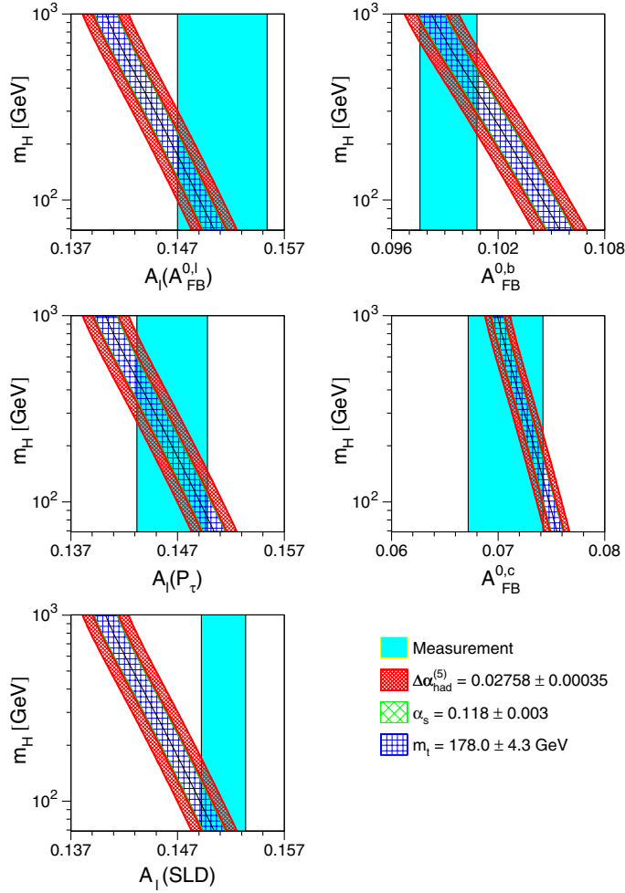
Fig. 8.5. Comparison of the LEP/SLD combined measurements of \mathcal{A}_\ell(A_{\text{FB}}^{0,\ell}) , \mathcal{A}_\ell(P_\tau) , \mathcal{A}_\ell(\text{SLD}) , A_{\text{FB}}^{0,b} and A_{\text{FB}}^{0,c} with the SM prediction as a function of the mass of the Higgs boson. The measurement with its uncertainty is shown as the vertical band. The width of the SM band arises due to the uncertainties in \Delta\alpha_{\text{had}}^{(S)}(m_Z^2) , \alpha_S(m_Z^2) and m_t in the ranges indicated. The total width of the band is the linear sum of these uncertainties.
