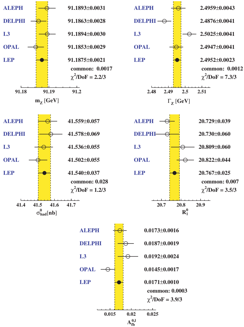
Fig. 2.9. Measurements of m_Z , \Gamma_Z , \sigma_{\text{had}}^0 , R_\ell^0 and A_{\text{FB}}^{0,\ell} . The averages indicated were obtained using the common errors and combination method discussed in the text. The values of \chi^2 per degree of freedom were calculated considering error correlations between measurements of the same parameter, but not error correlations between different parameters.
