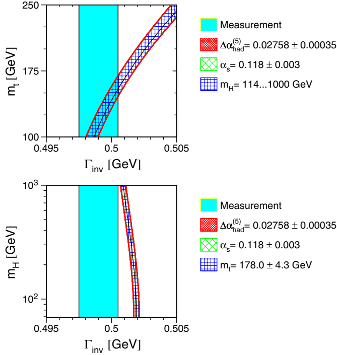
Fig. 7.1. Comparison of the LEP combined result on \Gamma_{\text{inv}} with the SM prediction as a function of (top) the top quark mass, and (bottom) the Higgs boson mass. The measurement with its uncertainty is shown as the vertical band. The width of the SM band arises due to the uncertainties in \Delta\alpha_{\text{had}}^{(5)}(m_Z^2) , \alpha_s(m_Z^2) , m_H and m_t in the ranges indicated. The total width of the band is the linear sum of these uncertainties.
