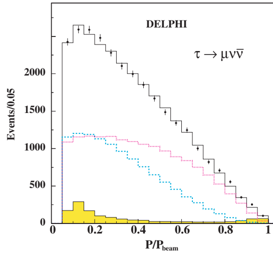
Fig. 4.6. The measured spectrum of the polarisation-sensitive variable for the \tau \rightarrow \mu \nu \bar{\nu} decays in the DELPHI experiment. The variable is the ratio of the measured muon momentum to the beam energy, which is an approximation of x_\mu = E_\mu/E_\tau . The data are compared to the results of the polarisation fit. The points with error bars are data and the solid line is simulated data for the fitted values of \mathcal{A}_\tau and \mathcal{A}_e . The shaded area is background and the dashed and dotted lines correspond to the positive and negative helicity contributions, respectively.
