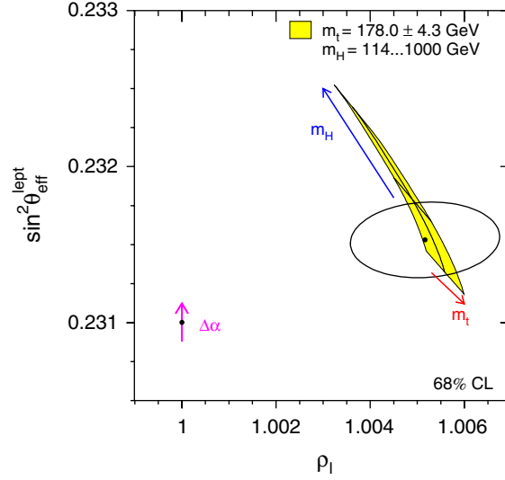
Fig. 7.7. Contour curve of 68% probability in the (\rho_\ell, \sin^2 \theta_{\text{eff}}^{\text{lept}}) plane. The prediction of a theory based on electroweak Born-level formulae and QED with running \alpha is shown as the dot, with the arrow representing the uncertainty due to the hadronic vacuum polarisation \Delta\alpha_{\text{had}}^{(5)}(m_Z^2) . The same uncertainty also affects the SM prediction, shown as the shaded region drawn for fixed \Delta\alpha_{\text{had}}^{(5)}(m_Z^2) while m_t and m_H are varied in the ranges indicated.
