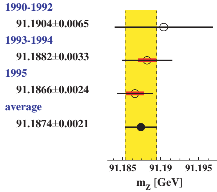
Fig. 2.10. m_Z in GeV for three different periods of data taking, before 1993, 1993–1994 and 1995. The second, smaller error bar represents the correlated error component of 1.2 MeV between m_Z^{93-94} and m_Z^{95} . The value of m_Z^{90-92} is essentially uncorrelated with the other two.
