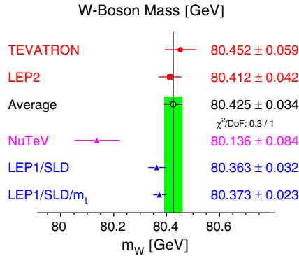
Fig. 8.9. Results on the mass of the W boson, m_W . The direct measurements of m_W at LEP-II (preliminary) and at Run-I of the Tevatron (top) are compared with the indirect determinations (bottom). The NuTeV result interpreted in terms of m_W is shown separately.
