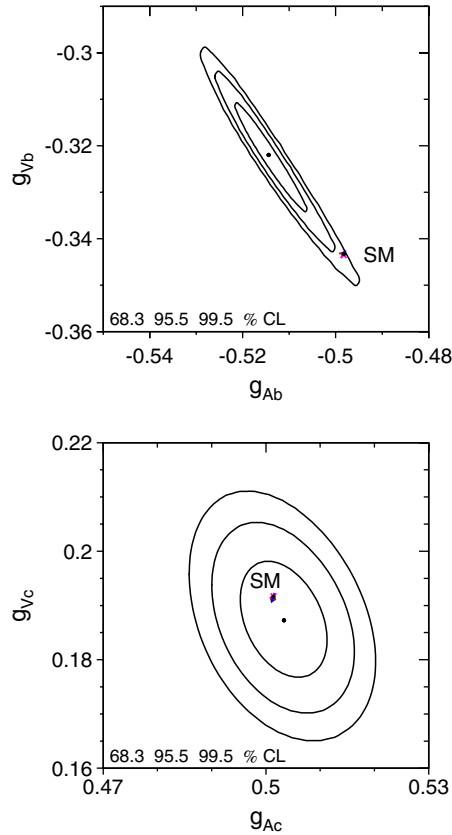
Fig. 7.4. Comparison of the effective vector and axial-vector coupling constants for heavy quarks, using results on leptons and assuming lepton universality (Table 7.9). Top: b-quarks; bottom: c-quarks. Compared to the experimental uncertainties, the SM predictions for the heavy quarks b and c have negligible dependence on the SM input parameters.
