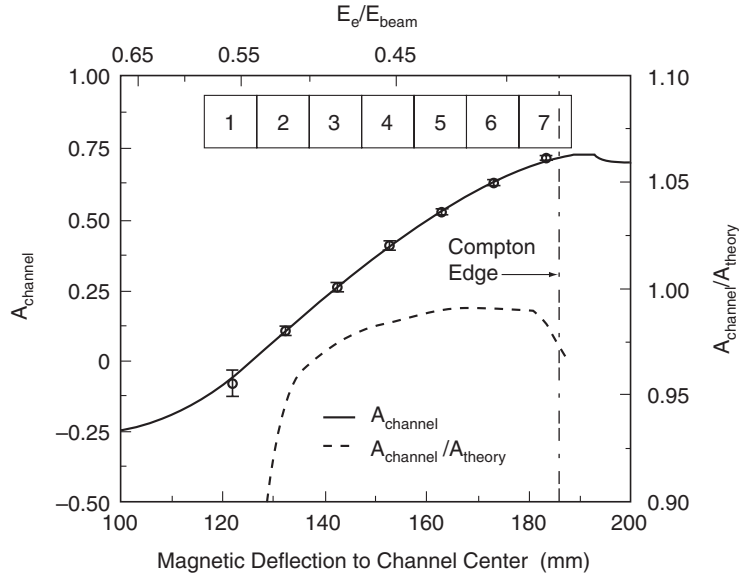
Fig. 3.2. Compton scattering asymmetry as a function of channel position. The deflection of the electron beam in the spectrometer is shown on the horizontal axis as the distance in mm from the centre of the detector channels, each 1 cm wide, to the path of a hypothetical infinite momentum electron beam. The inset shows the seven inner detector channels, sized to match the horizontal scale. The per channel asymmetry data is plotted as open circles, and the corrected asymmetry function is the solid curve. The relative size of the correction to the theoretical QED calculation is indicated by the dashed curve and the right-side vertical scale.
