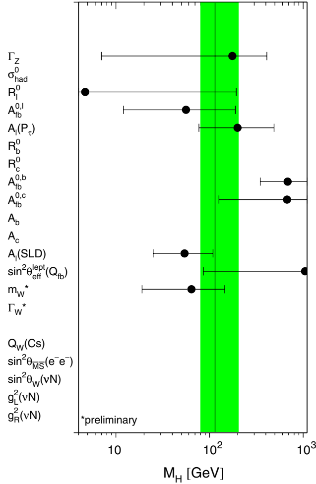
Fig. 8.15. Constraints on the mass of the Higgs boson from each pseudo-observable. The Higgs-boson mass and its 68% CL uncertainty is obtained from a five-parameter SM fit to the observable, constraining \Delta\alpha_{\text{had}}^{(5)}(m_Z^2) = 0.02758 \pm 0.00035 , \alpha_S(m_Z^2) = 0.118 \pm 0.003 , m_Z = 91.1875 \pm 0.0021 GeV and Tevatron Run-I m_t = 178.0 \pm 4.3 GeV. Only significant constraints are shown. Because of these four common constraints the resulting Higgs-boson mass values cannot be combined. The shaded band denotes the overall constraint on the mass of the Higgs boson derived from all pseudo-observables reported in Table 8.3. The direct measurements of m_W and \Gamma_W used in that analysis are preliminary.
