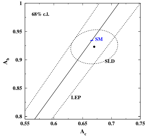
Fig. 5.17. Contours in the \mathcal{A}_c – \mathcal{A}_b plane and ratios of forward–backward asymmetries from the SLD and LEP, corresponding to 68% confidence levels assuming Gaussian systematic errors. The SM prediction for m_t = 178.0 \pm 4.3 GeV, m_H = 300_{-186}^{+700} GeV and \Delta\alpha_{\text{had}}^{(5)}(m_Z^2) = 0.02758 \pm 0.00035 is also shown.
