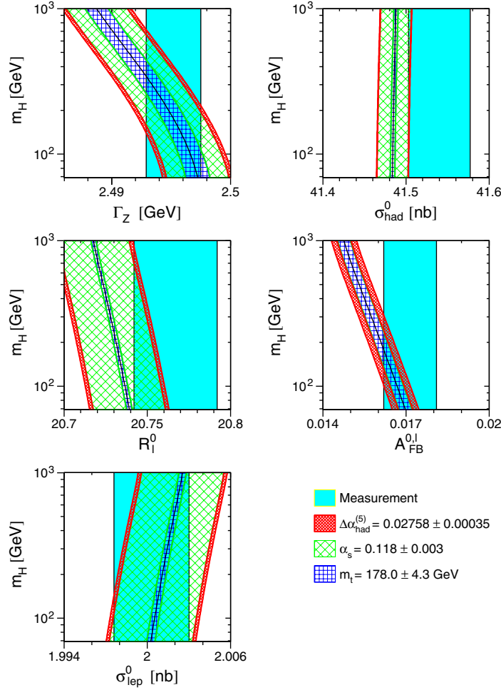
Fig. 8.4. Comparison of the LEP combined measurements of \Gamma_Z , \sigma_{\text{had}}^0 , R_\ell^0 , A_{\text{FB}}^{0,\ell} and \sigma_{\text{lep}}^0 with the SM prediction as a function of the mass of the Higgs boson. The measurement with its uncertainty is shown as the vertical band. The width of the SM band arises due to the uncertainties in \Delta\alpha_{\text{had}}^{(5)}(m_Z^2) , \alpha_S(m_Z^2) and m_t in the ranges indicated. The total width of the band is the linear sum of these uncertainties.
