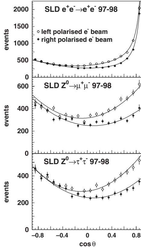
Fig. 3.7. Polar-angle distributions for Z decays to e, \mu and \tau pairs for the 1997–1998 SLD run. The solid line represents the fit, while the points with error bars show the data in bins of 0.1 in \cos \theta_{\text{thrust}} . For |\cos \theta_{\text{thrust}}| > 0.7 , the data are corrected for a decrease in the detection efficiency with increasing |\cos \theta_{\text{thrust}}| . Note that the polarisation independence at \cos \theta = -1 implied by Eq. (3.12), for the case of lepton universality, is apparent.
