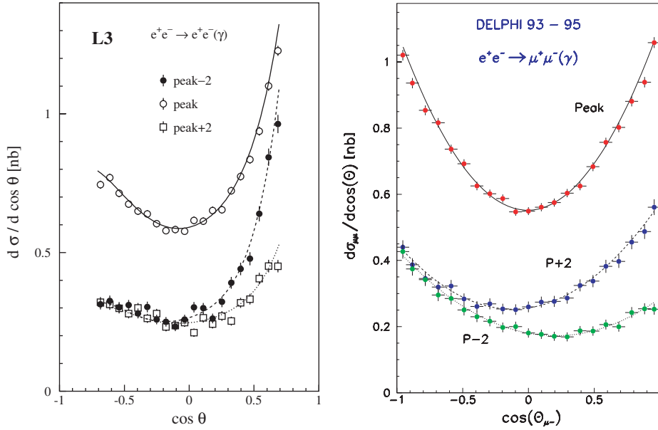
Fig. 2.5. Distribution of the production polar angle, \cos \theta , for e^+e^- and \mu^+\mu^- events at the three principal energies during the years 1993–1995, measured in the L3 (left) and DELPHI (right) detectors, respectively. The curves show the SM prediction from ALIBABA [52] for e^+e^- and a fit to the data for \mu^+\mu^- assuming the parabolic form of the differential cross-section given in the text.
