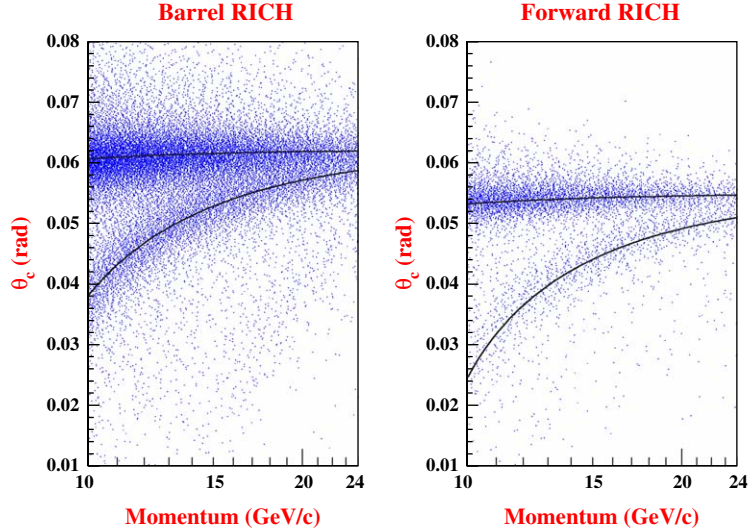
Fig. F.1. For a sample of tracks in DELPHI 1994 data, the reconstructed average Cherenkov angle in the gaseous radiator of (left) the barrel RICH and (right) the forward RICH as a function of the particle momentum. The two solid lines show the Cherenkov angle for the pion (upper) and kaon (lower) hypotheses.
