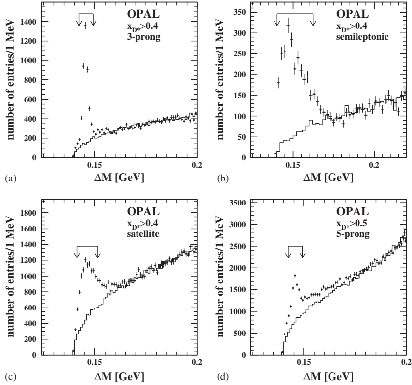
Fig. 5.8. Mass difference spectrum m(\pi^+D^0) - m(D^0) from OPAL in different channels [130]. In (a) and (d) the D^0 is fully reconstructed in the decay modes D^0 \rightarrow K^- \pi^+ and D^0 \rightarrow K^- \pi^+ \pi^- . In (c) the decay mode D^0 \rightarrow K^- \pi^+ \pi^0 is used, where the \pi^0 is not reconstructed. This K^- \pi^+ mass peak is enhanced due to the large polarisation of the intermediate \rho^+ produced in the D^0 \rightarrow K^- \rho^+ \rightarrow K^- \pi^+ \pi^0 decay. In (b) the D^0 is partially reconstructed in the semileptonic decay mode. The points with the error bars are the measured data. The solid histogram is the background estimated from measured data by a hemisphere mixing technique.
