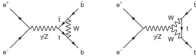
Fig. 1.10. Vertex corrections to the process e^+e^- \rightarrow b\bar{b} .
