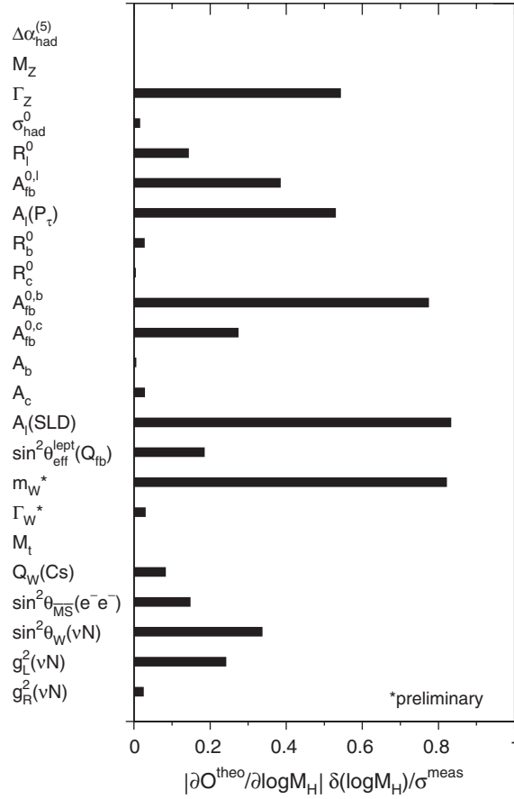
Fig. 8.2. Sensitivity of each pseudo-observable to the mass of the Higgs boson, defined as the partial derivative of the SM calculation of the observable with respect to \log_{10}(m_H/\text{GeV}) , relative to the total measurement error \sigma on the pseudo-observable, and multiplied by the \pm 0.2 uncertainty \delta in \log_{10}(m_H/\text{GeV}) (see Tables 8.1 and 8.3). The other SM input parameters are kept fixed at values \Delta\alpha_{\text{had}}^{(5)}(m_Z^2) = 0.02758 , \alpha_S(m_Z^2) = 0.118 , m_Z = 91.1875 \text{ GeV} , and m_t = 178 \text{ GeV} . The direct measurements of m_W and \Gamma_W used here are preliminary.
