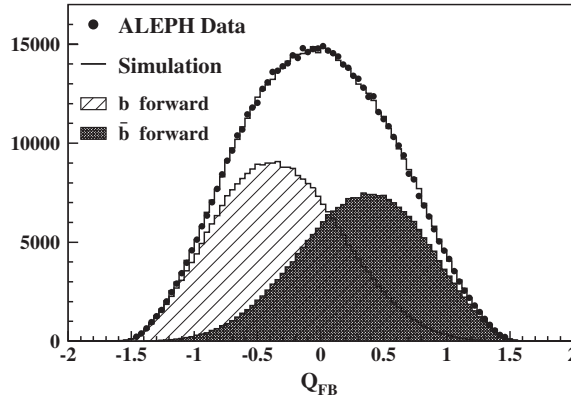
Fig. 5.12. Charge separation of the ALEPH neural net tag using jet charge, vertex charge and charged kaons [142]. The asymmetry reflects A_{\text{FB}}^{\text{b}\bar{\text{b}}} diluted by the non-perfect charge tagging.
