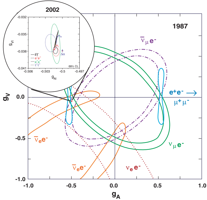
Fig. 1.15. The neutrino scattering and e^+e^- annihilation data available in 1987 constrained the values of g_{V\ell} and g_{A\ell} to lie within broad bands, whose intersections helped establish the validity of the SM and were consistent with the hypothesis of lepton universality. The inset shows the results of the LEP/SLD measurements at a scale expanded by a factor of 65 (see Fig. 7.3). The flavour-specific measurements demonstrate the universal nature of the lepton couplings unambiguously on a scale of approximately 0.001.
