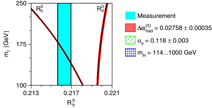
Fig. 7.8. Comparison of the LEP combined measurement of R_b^0 with the SM prediction as a function of the mass of the top quark. The measurement with its uncertainty is shown as the vertical band. The two curves show the expectations for R_b^0 and R_d^0 as a function of m_t . The SM prediction for R_d^0 displays a markedly smaller m_t dependence which is also of opposite sign. The parametric uncertainties on the SM expectations due to the uncertainties in \Delta\alpha_{\text{had}}^{(5)}(m_Z^2) , \alpha_s(m_Z^2) and m_H are shown as the width of the curves, they are negligible compared to the uncertainty of the measurement.
