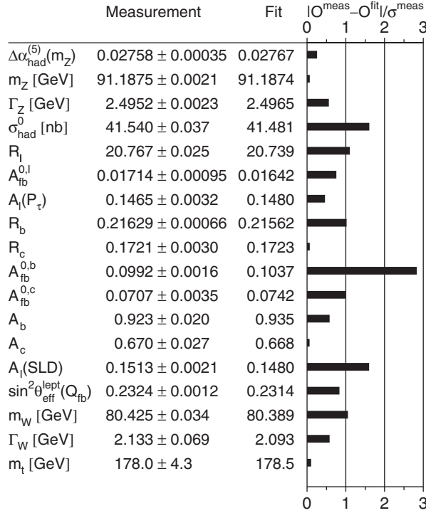
Fig. 8.14. Comparison of the measurements with the expectation of the SM, calculated for the five SM input parameter values in the minimum of the global \chi^2 of the fit. Also shown is the pull of each measurement, where pull is defined as the difference of measurement and expectation in units of the measurement uncertainty. The direct measurements of m_W and \Gamma_W used here are preliminary.
