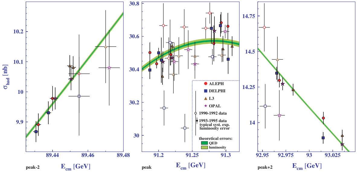
Fig. 2.3. Measurements by the four experiments of the hadronic cross-sections around the three principal energies. The vertical error bars show the statistical errors only. The open symbols represent the early measurements with typically much larger systematic errors than the later ones, shown as full symbols. Typical experimental systematic errors on the determination of the luminosity are indicated in the legend; these are almost fully correlated within each experiment, but uncorrelated among the experiments. The horizontal error bars show the uncertainties in LEP centre-of-mass energy, where the errors for the period 1993–1995 are smaller than the symbol size in some cases. The centres of the bands represent the cross-section parametrisation in terms of the combined pseudo-observables of the four experiments. The width of the bands represents the linear superposition of the two most important common theoretical errors from initial-state photon radiation and from the calculations of the small-angle Bhabha cross-section.
