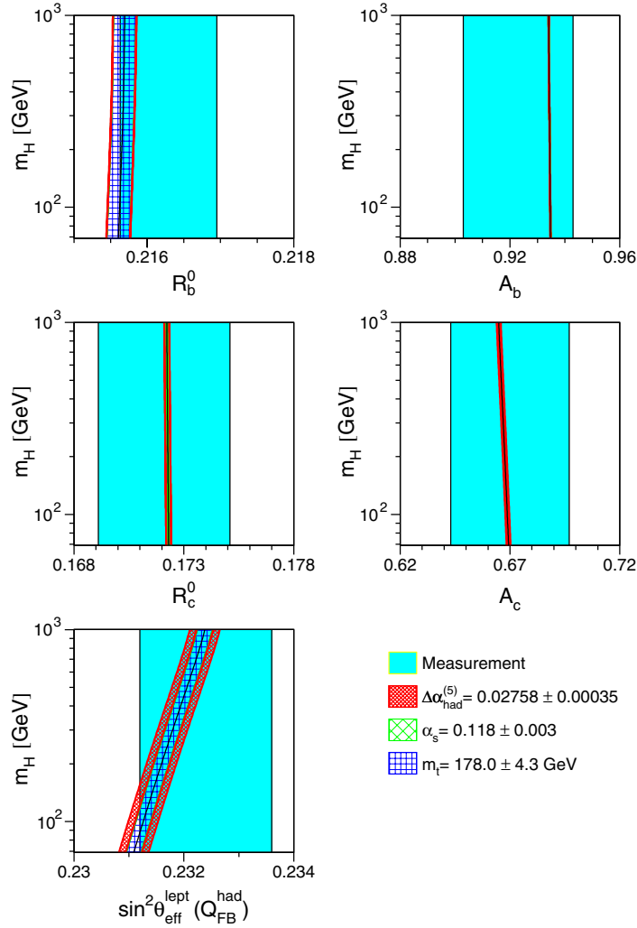
Fig. 8.6. Comparison of the LEP/SLD combined measurements of R_b^0 , R_c^0 , A_b , A_c and \sin^2 \theta_{\text{eff}}^{\text{lept}}(Q_{\text{FB}}^{\text{had}}) with the SM prediction as a function of the mass of the Higgs boson. The measurement with its uncertainty is shown as the vertical band. The width of the SM band arises due to the uncertainties in \Delta\alpha_{\text{had}}^{(5)}(m_Z^2) , \alpha_s(m_Z^2) and m_t in the ranges indicated. The total width of the band is the linear sum of these uncertainties.
