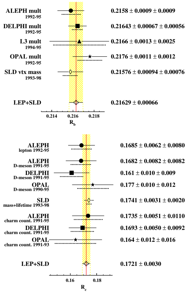
Fig. 5.13. R_b^0 and R_c^0 measurements used in the heavy flavour combination, corrected for their dependence on parameters evaluated in the multi-parameter fit described in the text. The dotted lines indicate the size of the systematic error.
