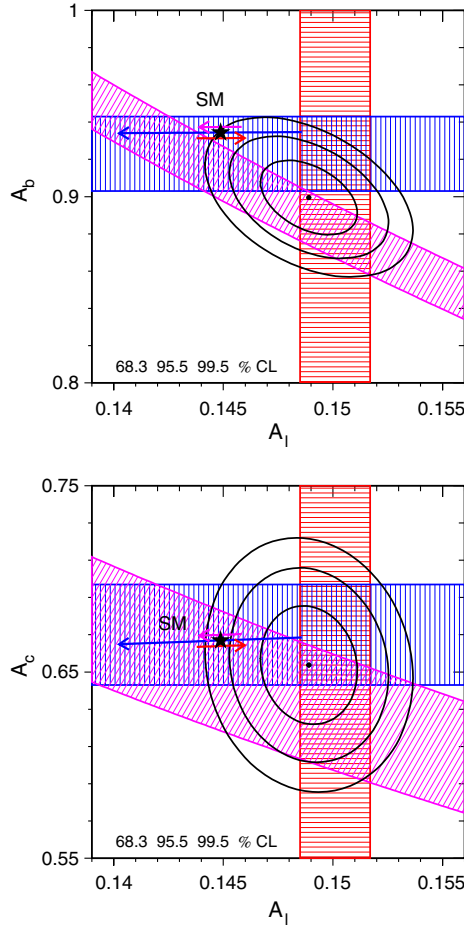
Fig. 7.2. Comparison of the measurements of \mathcal{A}_\ell , \mathcal{A}_q and A_{\text{FB}}^{0,q} for (top) b-quarks, and (bottom) c-quarks, assuming lepton universality. Bands of \pm 1 standard deviation width in the (\mathcal{A}_\ell, \mathcal{A}_q) plane are shown for the measurements of \mathcal{A}_\ell (vertical band), \mathcal{A}_q (horizontal band), and A_{\text{FB}}^{0,q} = (3/4)\mathcal{A}_e\mathcal{A}_q (diagonal band). Also shown are the 68%, 95% and 99.5% confidence level contours for the two asymmetry parameters resulting from the joint analysis (Table 7.6). The arrows pointing to the right and to the left show the variation in the SM prediction for varying \Delta\alpha_{\text{had}}^{(5)}(m_Z^2) in the range 0.02758 \pm 0.00035 (arrow displaced vertically upwards), m_H in the range 300^{+700}_{-186} GeV, and m_t in the range 178.0 \pm 4.3 GeV (arrow displaced vertically downwards). All arrows point in the direction of increasing values of these parameters.
