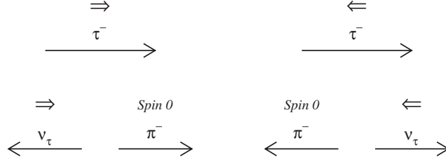
Fig. 4.1. Decay configurations for two \tau helicity states for the decay \tau^- \rightarrow \pi^- \nu_\tau . The positive helicity configuration is on the left and the negative configuration is on the right. For each particle, the long arrow depicts the momentum direction while the short double arrow that of the spin. The lower pair of figures is depicted in the helicity rest frame of the parent \tau .
