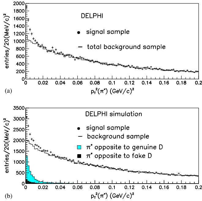
Fig. 5.9. p_T^2 spectrum of the slow pion opposite a high energy D-meson candidate [132]. The points show pions with charge opposite that of the charm quark in the D-meson, while the histogram shows those with the same charge. The data is shown in (a) and the simulation in (b), with the signal component indicated separately.
