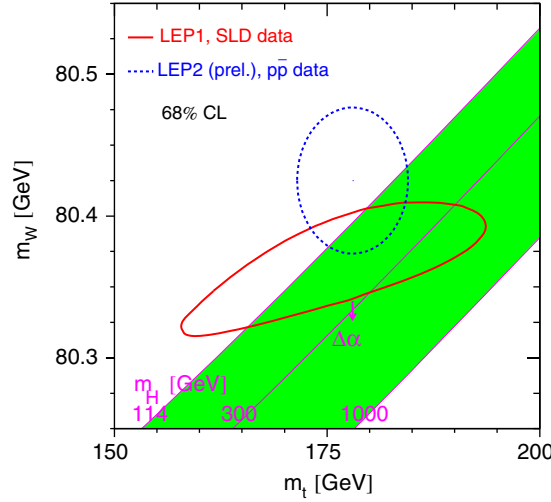
Fig. 8.10. Contour curves of 68% probability in the (m_t, m_W) plane. The shaded band shows the SM prediction based on the value for G_F for various values of the Higgs-boson mass and fixed \Delta\alpha_{\text{had}}^{(5)}(m_Z^2) ; varying the hadronic vacuum polarisation by \Delta\alpha_{\text{had}}^{(5)}(m_Z^2) = 0.02758 \pm 0.00035 yields an additional uncertainty on the SM prediction shown by the arrow labeled \Delta\alpha . The direct measurement of m_W used here is preliminary.
