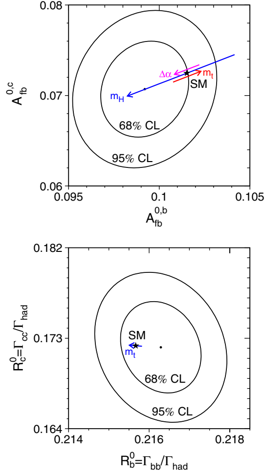
Fig. 5.18. Contours in the A_{FB}^{0,c} - A_{FB}^{0,b} and R_c^0 - R_b^0 planes from the LEP and SLD data, corresponding to 68% confidence levels assuming Gaussian systematic errors. The SM prediction for m_t = 178.0 \pm 4.3 GeV, m_H = 300_{-186}^{+700} GeV and \Delta\alpha_{had}^{(5)}(m_Z^2) = 0.02758 \pm 0.00035 is also shown.
