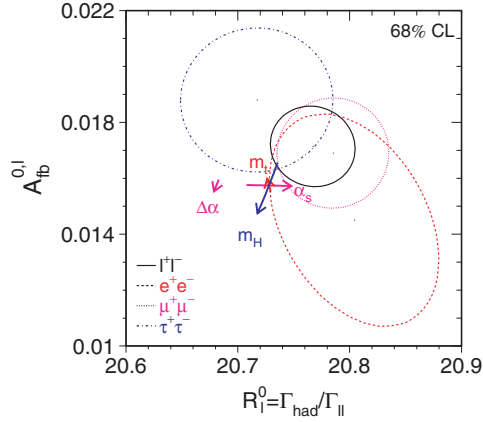
Fig. 2.11. Contour lines (68% CL) in the R_\ell^0 - A_{\text{FB}}^{0,\ell} plane for e^+e^- , \mu^+\mu^- and \tau^+\tau^- final states and for all leptons combined. For better comparison the results for the \tau lepton are corrected to correspond to the massless case. The SM prediction for m_Z = 91.1875 GeV, m_t = 178.0 GeV, m_H = 300 GeV, and \alpha_S(m_Z^2) = 0.118 is also shown as the intersection of the lines with arrows, which correspond to the variation of the SM prediction when m_t , m_H and \alpha_S(m_Z^2) are varied in the intervals m_t = 178.0 \pm 4.3 GeV, m_H = 300^{+700}_{-186} GeV, and \alpha_S(m_Z^2) = 0.118 \pm 0.003 , respectively. The arrow showing the small dependence on the hadronic vacuum polarisation \Delta\alpha_{\text{had}}^{(5)}(m_Z^2) = 0.02758 \pm 0.00035 is displaced for clarity. The arrows point in the direction of increasing values of these parameters.
