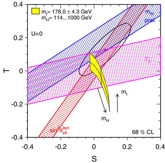
Fig. E.2. Contour curve of 68% probability in the (T, S) plane. Also shown are \pm 1 standard deviation bands corresponding to the measurements of \Gamma_{\ell\ell}, m_W and \sin^2 \theta_{\text{eff}}^{\text{lept}} . The shaded region shows the predictions within the SM for m_t = 178.0 \pm 4.3 GeV (Tevatron Run-I) and m_H = 300_{-186}^{+700} GeV, for a fixed hadronic vacuum polarisation of \Delta\alpha_{\text{had}}^{(5)}(m_Z^2) = 0.02758 . The SM reference point at which all STU parameters vanish is chosen to be: \Delta\alpha_{\text{had}}^{(5)}(m_Z^2) = 0.02758 , \alpha_S(m_Z^2) = 0.118 , m_Z = 91.1875 GeV, m_t = 175 GeV, m_H = 150 GeV. The constraint U = 0 is always applied. The direct measurement of m_W used here is preliminary.
