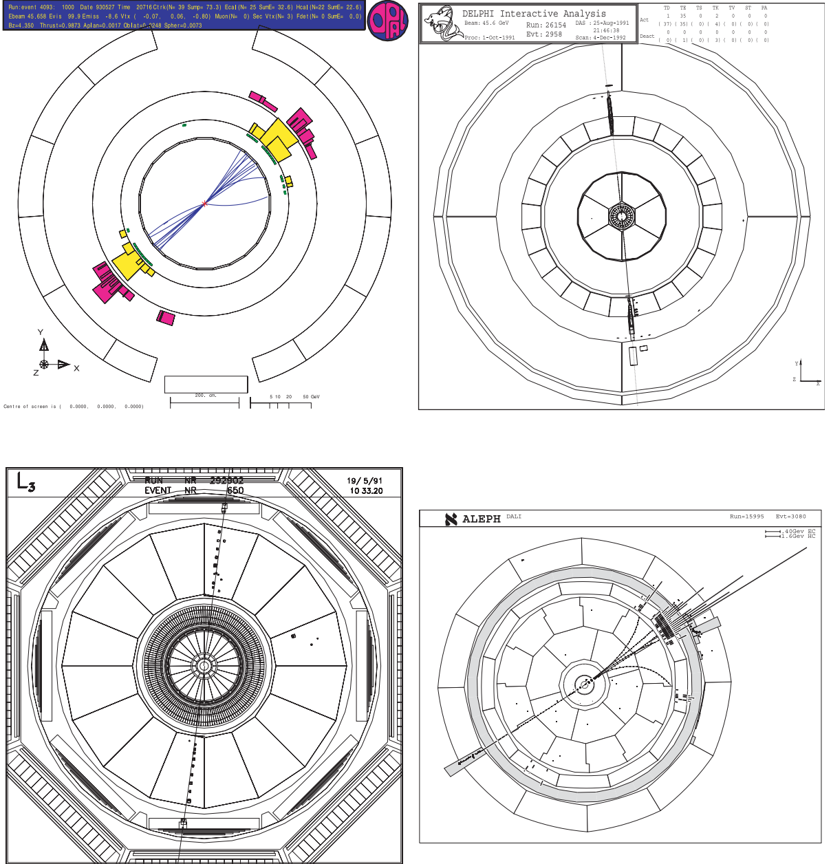
Fig. 1.7. Pictures of q\bar{q} , e^+e^- , \mu^+\mu^- and \tau^+\tau^- final states, visualised with the event displays of the OPAL, DELPHI, L3 and ALEPH collaborations, respectively. In all views, the electron–positron beam axis is perpendicular to the plane of the page. The stability of the electron and the long lifetime of the muon allow these fundamental Z decays to be directly observed, while the low-multiplicity products of \tau decays are confined to well-isolated cones. Hadronic Z decays result in higher-multiplicity jets of particles produced in the QCD cascades initiated by the initial q\bar{q} pair.
