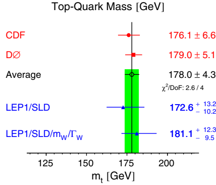
Fig. 8.8. Results on the mass of the top quark. The direct measurements of m_t at Run-I of the Tevatron (top) are compared with the indirect determinations (bottom).
