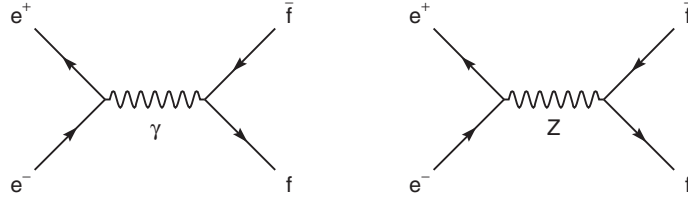
Fig. 1.1. The lowest-order s -channel Feynman diagrams for e^+e^- \rightarrow f\bar{f} . For e^+e^- final states, the photon and the Z boson can also be exchanged via the t -channel. The contribution of Higgs boson exchange diagrams is negligible.
