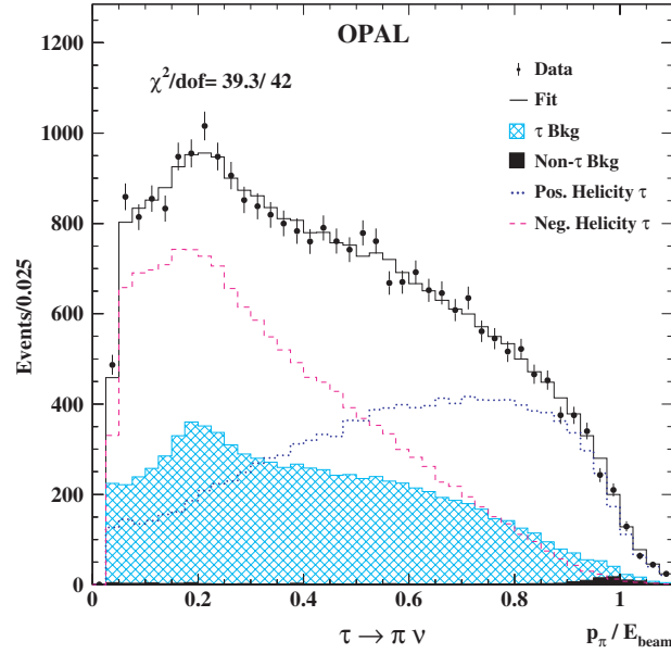
Fig. 4.3. The measured distributions in the polarisation-sensitive variable for the \tau \rightarrow \pi \nu decays in the OPAL experiment. The variable is the ratio of the measured charged hadron momentum to the beam energy, which is an approximation of x_\pi = E_\pi / E_\tau . The data, shown by points with error bars, are integrated over the whole \cos \theta_{\tau^-} range. Overlaying this distribution are Monte Carlo distributions for the positive (dotted line) and negative (dashed line) helicity \tau leptons and for their sum including background, assuming a value for \langle \mathcal{P}_\tau \rangle equal to the fitted polarisation. The hatched histogram represents the Monte Carlo expectations of contributions from cross-contamination from other \tau decays and the dark shaded histogram the background from non- \tau sources. The level of agreement between the data and Monte Carlo distributions is quantified by quoting the \chi^2 and the number of degrees of freedom.
