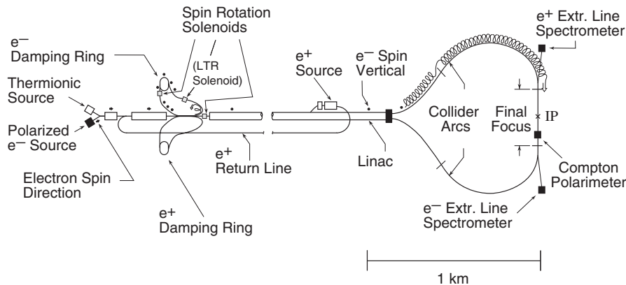
Fig. 1.4. The SLC linear collider complex, showing the electron source, the damping rings, the positron source, the 3 km long linac and arcs and the final focus. The helix and arrow superimposed on the upper arc schematically indicate the electron spin precession which occurs during transport.
