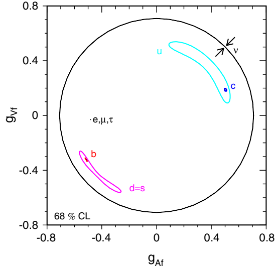
Fig. F.3. Comparison of the effective vector and axial-vector coupling constants for fermions. For the light-quark contours ( u and d = s ), a second solution exists, mirroring the contour curves at the origin. The allowed area for neutrinos, assuming three generations of neutrinos with identical vector couplings and identical axial–vector couplings, is bounded by circles centred at the origin since the invisible partial width constrains the sum of the squares of the effective couplings only.
