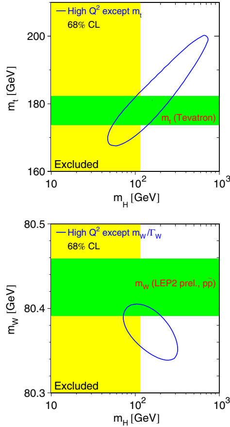
Fig. 8.11. Contour curves of 68% probability in (top) the (m_t, m_H) plane and (bottom) the (m_W, m_H) plane, based on all 18 measurements except the direct measurement of m_t and the direct measurements of m_W and \Gamma_W , respectively. The direct measurements of these excluded observables are shown as the horizontal bands of width \pm 1 standard deviation. The vertical band shows the 95% confidence level exclusion limit on m_H of 114.4 GeV derived from the direct search at LEP-II [39]. The direct measurements of m_W and \Gamma_W used here are preliminary.
