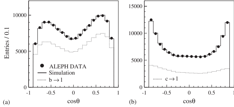
Fig. 5.10. Reconstructed \cos \theta distribution from the ALEPH asymmetry measurements with leptons for (a) the b-enriched and (b) the c-enriched sample [141]. The full histogram shows the expected raw angular distribution in the simulation. The dashed histogram show the signal component.
