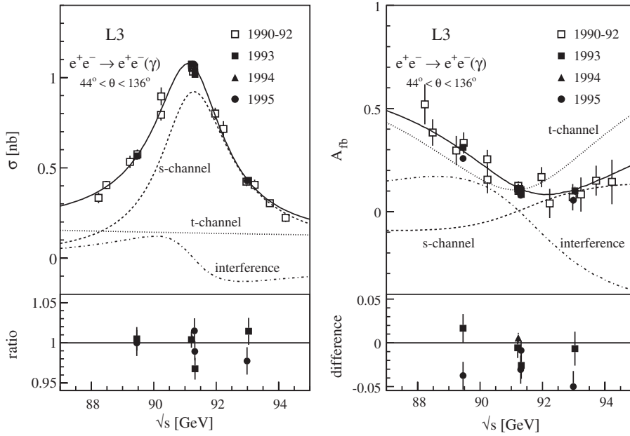
Fig. 2.4. The energy dependence and the contributions from the s - and t -channel diagrams and from the s - t interference for observables in the e^+e^- channel. Shown are the total cross-section (left) and the difference between the forward and backward cross-sections after normalisation to the total cross-section (right). The data points measured by the L3 collaboration refer to an angular acceptance of |\cos \theta| < 0.72 , an acollinearity \eta < 25^\circ and a minimum energy of E_{e^\pm} > 1 GeV. The lines represent the model-independent fit to all L3 data.
