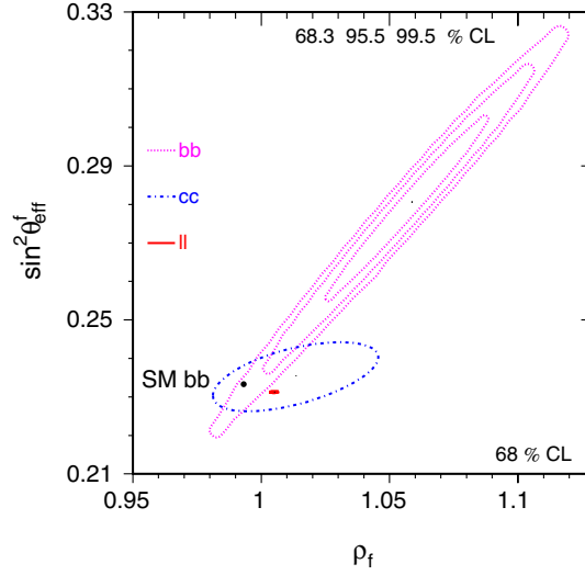
Fig. 7.5. Comparison of \rho_f and the effective electroweak mixing angle \sin^2 \theta_{\text{eff}}^f for leptons, b and c-quarks. The SM expectation for b-quarks is shown as the dot ( \rho_b < 1 ); those of c-quarks and of leptons are not drawn as they lie at the same area as the experimental contour curve for leptons ( \rho_\ell > 1 ). Only the 68% CL contour is shown for c-quarks and leptons. On the scale of this plot, variations of the SM prediction with m_t , m_H and \Delta\alpha_{\text{had}}^{(5)}(m_Z^2) are negligible.
