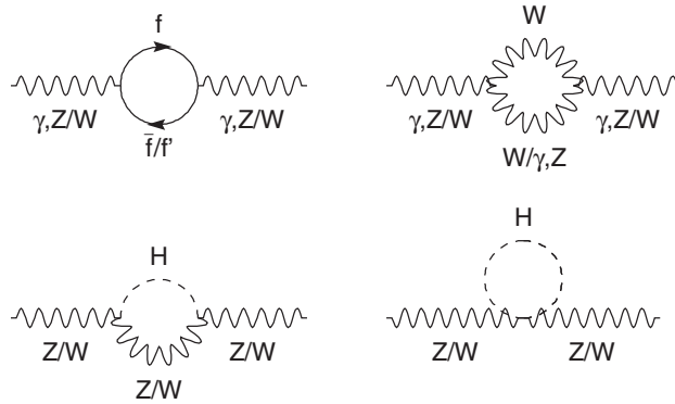
Fig. 1.9. Higher-order corrections to the gauge boson propagators due to boson and fermion loops.
