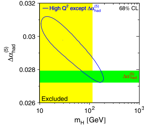
Fig. 8.12. Contour curve of 68% probability in the (\Delta\alpha_{\text{had}}^{(5)}(m_Z^2), m_H) plane, based on all 18 measurements except the constraint on \Delta\alpha_{\text{had}}^{(5)}(m_Z^2) . The direct measurements of the excluded observable is shown as the horizontal bands of width \pm 1 standard deviation. The vertical band shows the 95% confidence level exclusion limit on m_H of 114.4 GeV derived from the direct search at LEP-II [39]. The direct measurements of m_W and \Gamma_W used here are preliminary.
