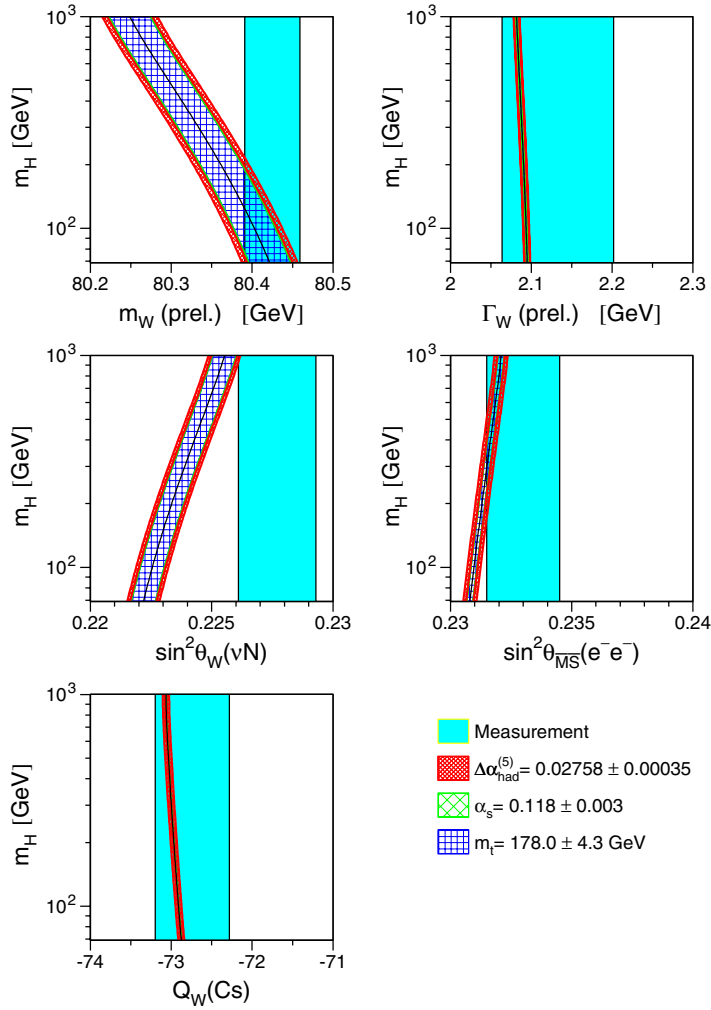
Fig. 8.7. Comparison of the combined measurements of m_W and \Gamma_W , and the results from low Q^2 processes \sin^2 \theta_W (\nu N) , \sin^2 \theta_{\overline{MS}}(m_Z) (e^-e^-) and Q_W (APV) with the SM prediction as a function of the mass of the Higgs boson. The measurement with its uncertainty is shown as the vertical band. The width of the SM band arises due to the uncertainties in \Delta\alpha_{\text{had}}^{(5)}(m_Z^2) , \alpha_s(m_Z^2) and m_t in the ranges indicated. The total width of the band is the linear sum of these uncertainties. The direct measurements of m_W and \Gamma_W used here are preliminary.
