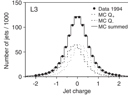
Fig. 6.1. The Q_+ and Q_- distributions obtained from Monte Carlo simulation by L3. Their sum is compared to the sum of the Q_F + Q_B \equiv Q_+ + Q_- distributions for 1994 data.
