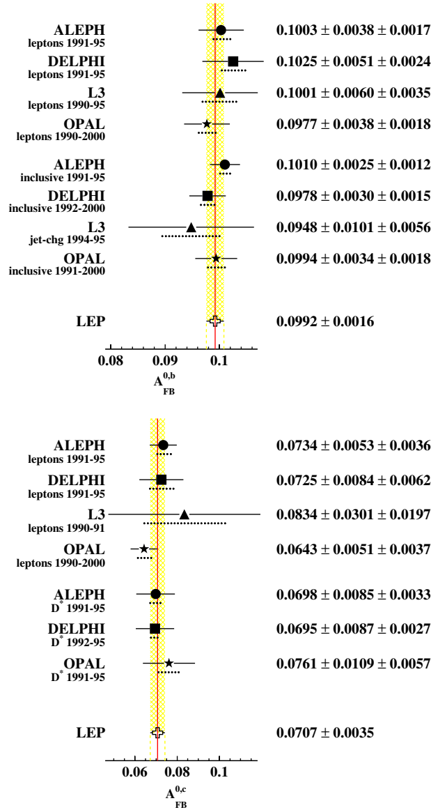
Fig. 5.14. A_{FB}^{0,b} and A_{FB}^{0,c} measurements used in the heavy flavour combination, corrected for their dependence on parameters evaluated in the multi-parameter fit described in the text. The A_{FB}^{0,b} measurements with D-mesons do not contribute significantly to the average and are not shown in the plots. The experimental results are derived from the ones shown in Tables C.3 to C.8 combining the different centre of mass energies. The dotted lines indicate the size of the systematic error.
