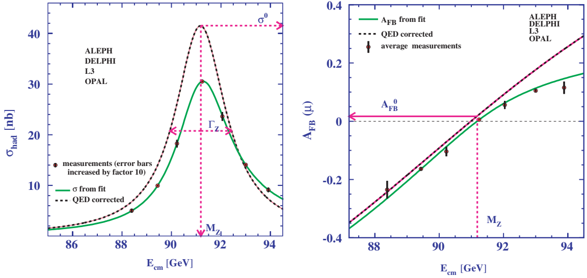
Fig. 1.12. Average over measurements of the hadronic cross-sections (left) and of the muon forward–backward asymmetry (right) by the four experiments, as a function of centre-of-mass energy. The full line represents the results of model-independent fits to the measurements, as outlined in Section 1.5. Correcting for QED photonic effects yields the dashed curves, which define the Z parameters described in the text.
