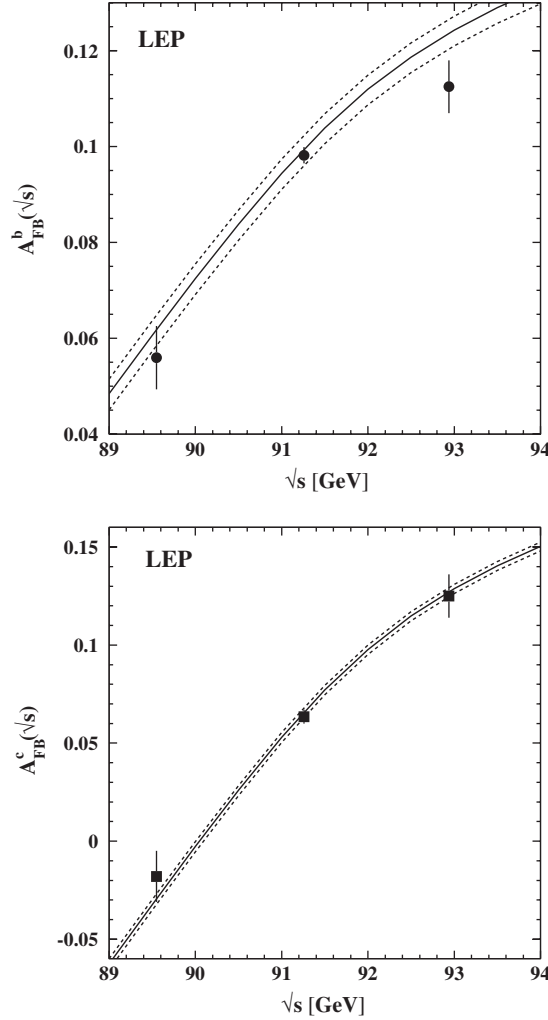
Fig. 5.16. Energy dependence of A_{FB}^b and A_{FB}^c . The solid line represents the SM prediction for m_t = 178 GeV, m_H = 300 GeV, the upper (lower) dashed line is the prediction for m_H = 100 (1000) GeV.
