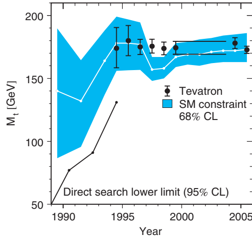
Fig. 1.16. Comparison of direct and indirect determinations of the mass of the top quark, m_t , as a function of time. The shaded area denotes the indirect determination of m_t at 68% confidence level derived from the analysis of radiative corrections within the framework of the SM using precision electroweak measurements. The dots with error bars at 68% confidence level denote the direct measurements of m_t performed by the Tevatron experiments CDF and DØ. Also shown is the 95% confidence level lower limit on m_t from the direct searches before the discovery of the top quark. Predictions and measurements agree well.
