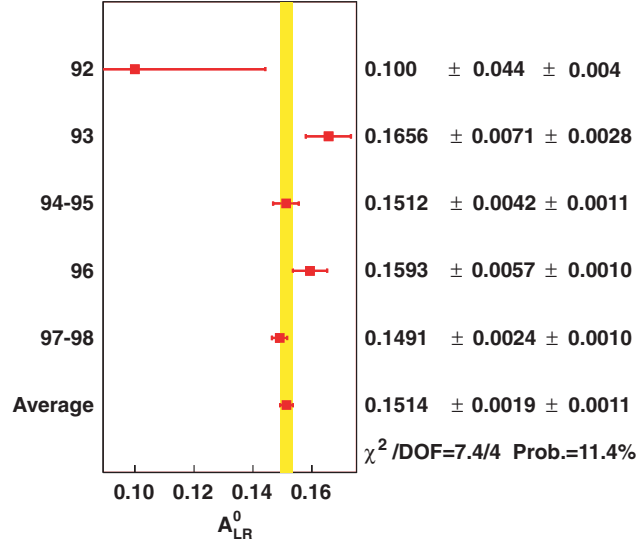
Fig. 3.6. A compilation of the published SLD A_{LR}^0 results, ordered by year. The final average is formed including correlations in systematic errors.
