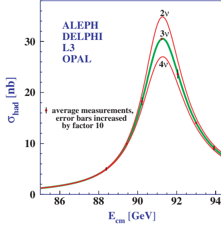
Fig. 1.13. Measurements of the hadron production cross-section around the Z resonance. The curves indicate the predicted cross-section for two, three and four neutrino species with SM couplings and negligible mass.
