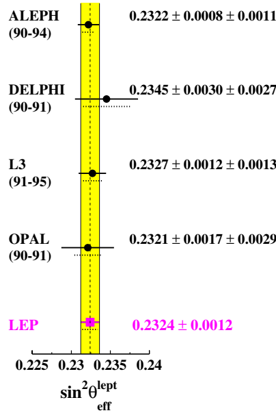
Fig. 6.2. The input values and derived average of \sin^2 \theta_{\text{eff}}^{\text{lept}} from Q_{\text{FB}}^{\text{had}} measurements. The total uncertainties are indicated by the solid lines, and the systematic contribution to the uncertainties by the dotted lines.
