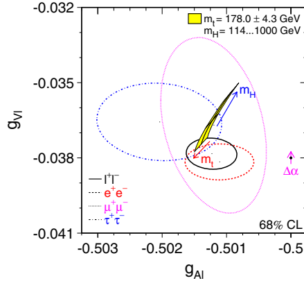
Fig. 7.3. Comparison of the effective vector and axial-vector coupling constants for leptons (Tables 7.7 and 7.8). The shaded region in the lepton plot shows the predictions within the SM for m_t = 178.0 \pm 4.3 GeV and m_H = 300^{+700}_{-186} GeV; varying the hadronic vacuum polarisation by \Delta\alpha_{\text{had}}^{(5)}(m_Z^2) = 0.02758 \pm 0.00035 yields an additional uncertainty on the SM prediction shown by the arrow labeled \Delta\alpha .
