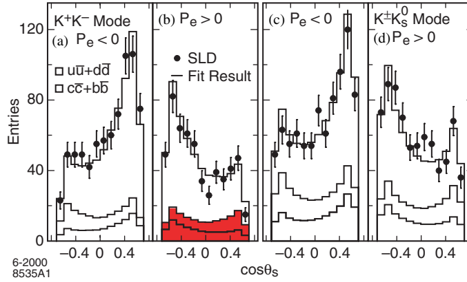
Fig. F.2. Measured s-quark polar angle distributions (dots) for selected SLD events in the (a),(b) K^+K^- and (c),(d) K^\pm K_S^0 modes, produced with (a),(c) left- and (b),(d) right-polarised electron beams. The histograms represent the result of a simultaneous fit to the four distributions, and the upper (lower) hatched areas indicate the estimated u\bar{u} + d\bar{d} ( c\bar{c} + b\bar{b} ) backgrounds.
