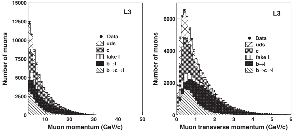
Fig. 5.5. Muon momentum and transverse momentum spectra obtained by L3, together with expectations from simulation for the contributions from the various sources.
