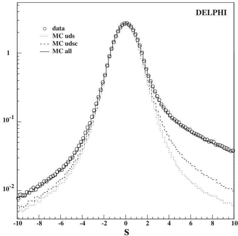
Fig. 5.1. Impact parameter significance from DELPHI for data and simulation. The contributions of the different quark flavours are shown separately. The normalisation is arbitrary.
