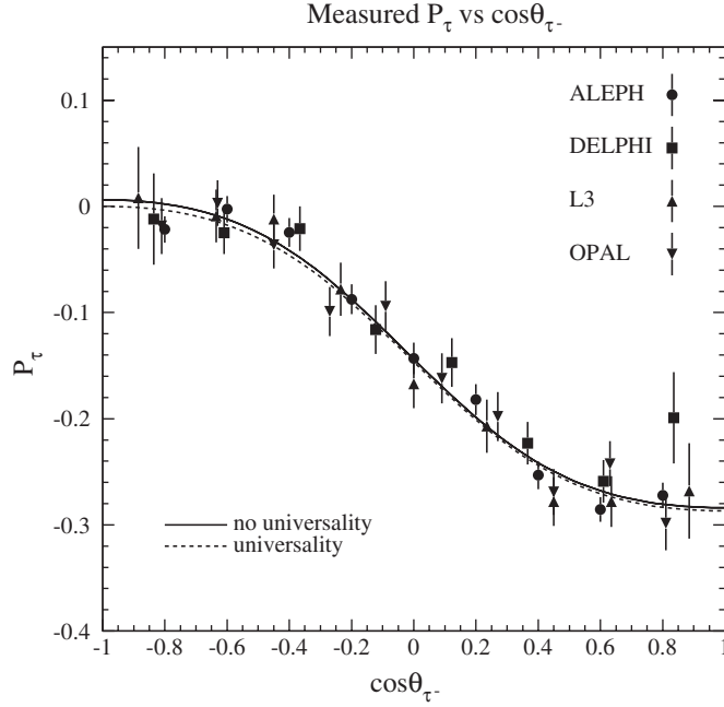
Fig. 4.7. The values of \mathcal{P}_\tau as a function of \cos \theta_{\tau-} as measured by each of the LEP experiments. Only the statistical errors are shown. The values are not corrected for radiation, interference or pure photon exchange. The solid curve overlays Eq. (4.2) for the LEP values of \mathcal{A}_\tau and \mathcal{A}_e . The dashed curve overlays Eq. (4.2) under the assumption of lepton universality for the LEP value of \mathcal{A}_\ell .
