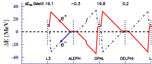
Fig. 2.8. Typical variations of the beam energy around the LEP ring during the 1993 run. Energy losses from synchrotron radiation in the arcs, and in wiggler magnets between the ALEPH and OPAL IPs, are compensated by acceleration in the radio frequency cavities mounted in the straight sections on both sides of L3 and OPAL. The detailed modelling results in significant corrections on the centre-of-mass energy at the IPs between acceleration sections, as indicated by the numbers on the top.
