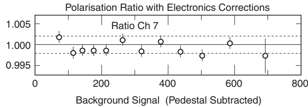
Fig. 3.3. The linearity of channel 7 is shown for a wide range of detector background levels (expressed here in pedestal subtracted ADC counts). Plotted on the vertical axis is the fully corrected polarisation result, normalised to the “zero background” case. The result here is seen to be constant to within 0.2% over the full range. Running conditions varied widely, but on average were a total response of 500 counts, including 300 counts of signal.
