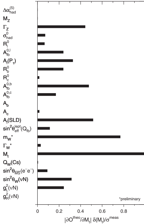
Fig. 8.1. Sensitivity of each pseudo-observable to the mass of the top quark, defined as the partial derivative of the SM calculation of the observable with respect to m_t , relative to the total measurement error \sigma on the pseudo-observable, and multiplied by the \pm 4.3 GeV uncertainty \delta in the Tevatron Run-I measurement of m_t . The other SM input parameters are kept fixed at values \Delta\alpha_{\text{had}}^{(5)}(m_Z^2) = 0.02758 , \alpha_S(m_Z^2) = 0.118 , m_Z = 91.1875 GeV, and m_H = 150 GeV. The direct measurements of m_W and \Gamma_W used here are preliminary.
