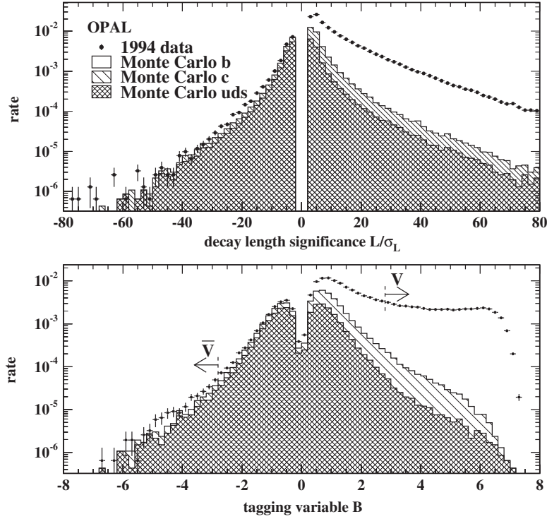
Fig. 5.3. Decay length significance L/\sigma_L (top) and neural network tagging variable (bottom) for the OPAL secondary vertex based b-tag [125]. The gaps around zero significance are due to neural network preselection cuts removing jets with no significant secondary vertex. v and \bar{v} are the cut values used in the R_b analysis.
