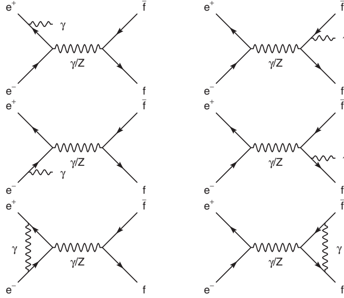
Fig. 1.11. Some of the lowest order QED corrections to fermion-pair production. Together with photonic box diagrams, which give much smaller contributions, these form a gauge-invariant sub-set included in the radiator functions H_{\text{QED}} . Weak boxes are added explicitly to the kernel cross-section [32].
