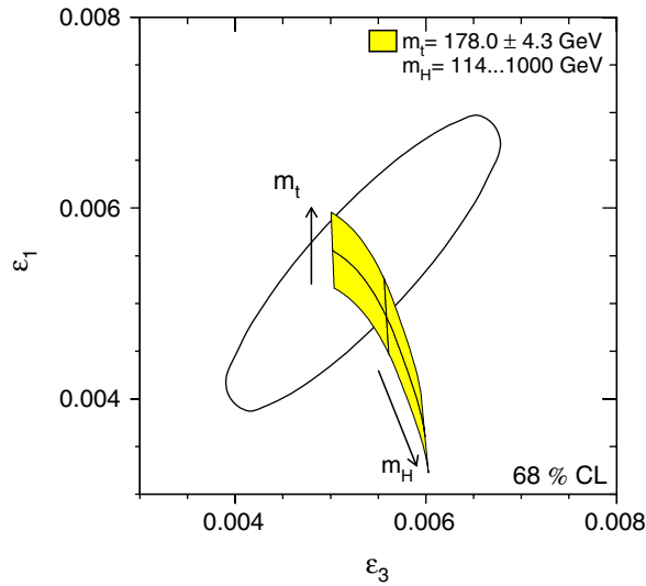
Fig. E.1. Contour curve of 68% probability in the (\epsilon_3, \epsilon_1) plane. The shaded region shows the predictions within the SM for m_t = 178.0 \pm 4.3 GeV (Tevatron Run-I) and m_H = 300_{-186}^{+700} GeV, for a fixed hadronic vacuum polarisation of \Delta\alpha_{\text{had}}^{(5)}(m_Z^2) = 0.02758 . The direct measurement of m_W used here is preliminary.
