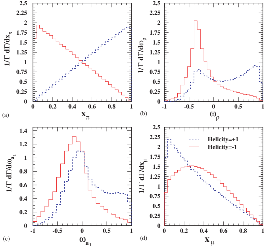
Fig. 4.2. Monte Carlo simulated distributions of polarisation sensitive kinematic variables defined in the text for (a) \tau \rightarrow \pi \nu , (b) \tau \rightarrow \rho \nu , (c) \tau \rightarrow a_1 \nu and (d) \tau \rightarrow \mu \nu decays for positive and negative helicity \tau leptons excluding the effects of selection and detector response.
