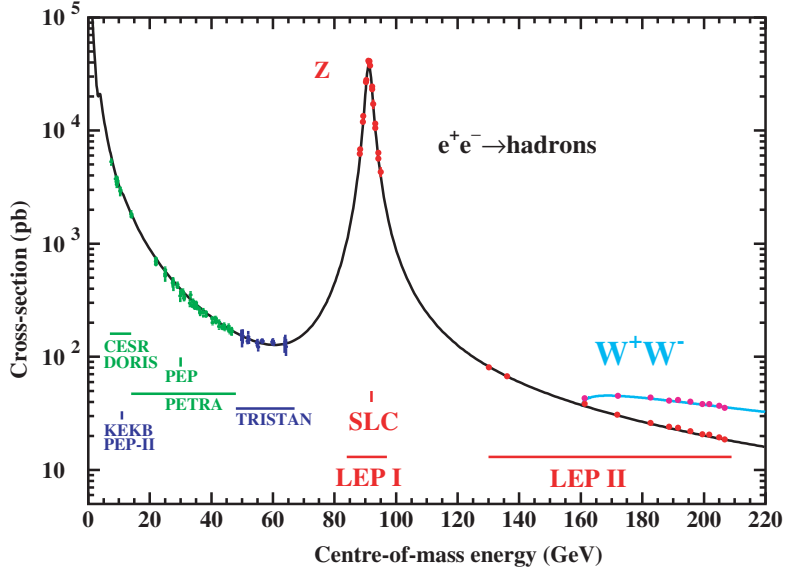
Fig. 1.2. The hadronic cross-section as a function of centre-of-mass energy. The solid line is the prediction of the SM, and the points are the experimental measurements. Also indicated are the energy ranges of various e^+e^- accelerators. The cross-sections have been corrected for the effects of photon radiation.
