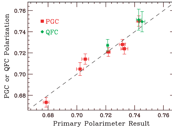
Fig. 3.4. The polarised gamma counter (PGC) and quartz fibre calorimeter (QFC) photon detector polarisation results (vertical axis) compared to the primary electron detector polarimeter measurements (horizontal axis).
