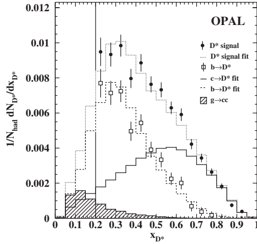
Fig. 5.6. D^{*\pm} momentum spectrum for all events and for b\bar{b} and c\bar{c} events from OPAL normalised to the beam energy after subtraction of combinatorial background [130].
