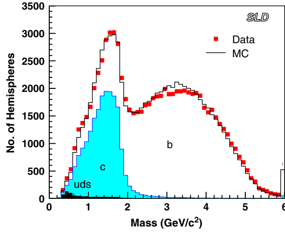
Fig. 5.4. Reconstructed vertex mass from SLD for data and simulation.
