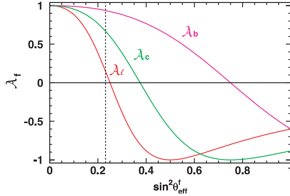
Fig. 1.14. In the SM the variation of \mathcal{A}_f with \sin^2 \theta_{\text{eff}}^f is controlled by the charge and weak isospin assignment of the fermion species concerned. The measured values of \sin^2 \theta_{\text{eff}}^f are near the vertical line. In this region, \mathcal{A}_\ell depends strongly on \sin^2 \theta_{\text{eff}}^{\text{lept}} , while \mathcal{A}_b depends much more weakly on \sin^2 \theta_{\text{eff}}^b .
