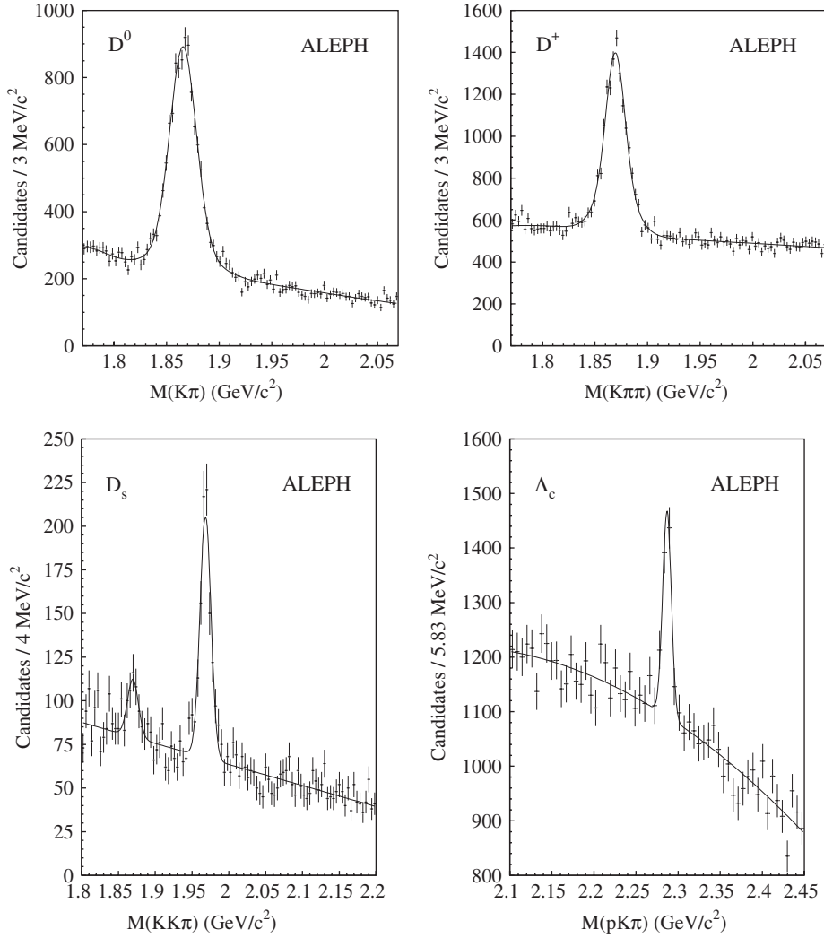
Fig. 5.7. Mass spectra for D^0 \rightarrow K^- \pi^+ , D^+ \rightarrow K^- \pi^+ \pi^+ , D_s \rightarrow K^+ K^- \pi^+ and \Lambda_c^+ \rightarrow p K^- \pi^+ obtained by ALEPH [131].
