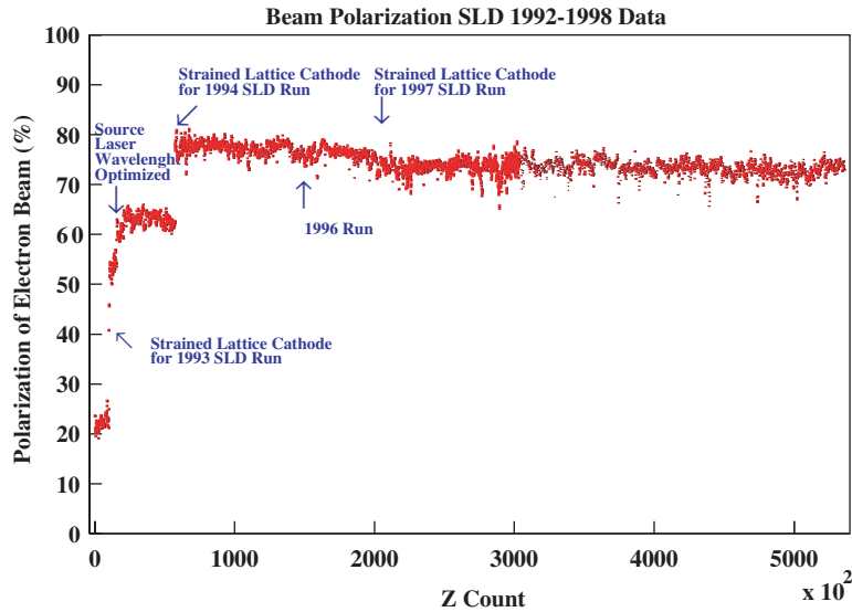
Fig. 1.5. The amount of longitudinal electron polarisation as a function of the number of recorded Z decays at SLD.
