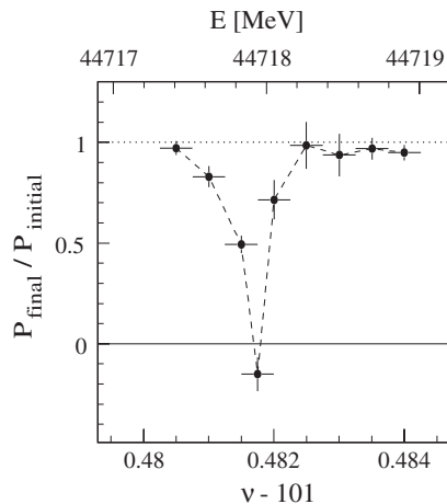
Fig. 2.6. Measurement of the width of the artificially excited spin resonance which is used for the energy calibration of LEP (from Ref. [54]). The drop in the observed polarisation level is shown as a function of the “fractional spin tune”, i.e. the spin tune \nu minus its integer part of 101.
