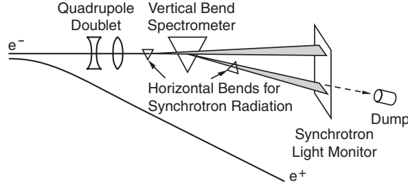
Fig. 3.5. The energy spectrometer for electrons (a similar device is used on the positron side) uses a precision bend magnet and synchrotron-radiation-producing deflector magnets before and after the bend, in order to determine the beam bend angle.
