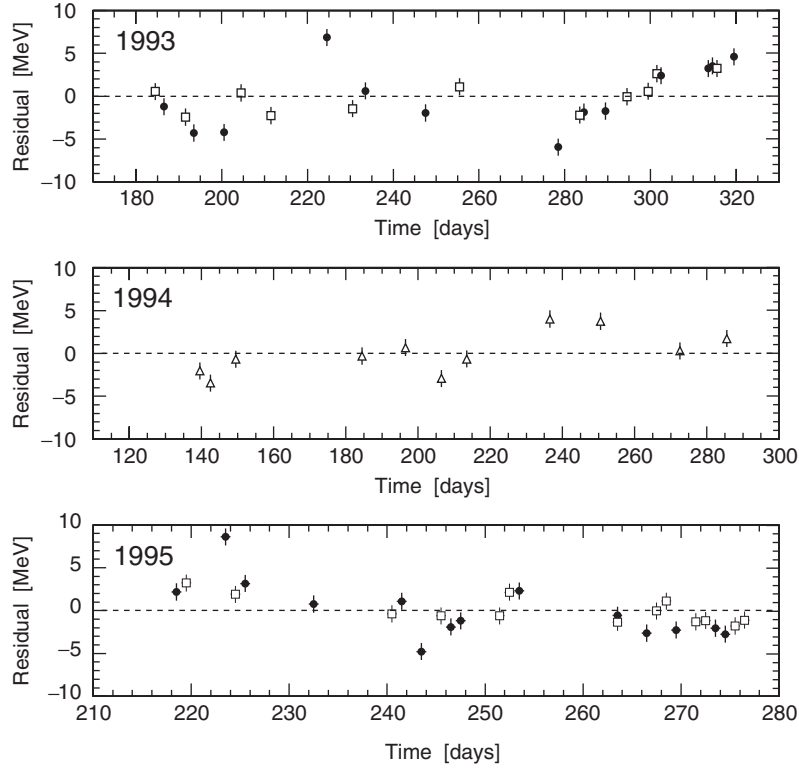
Fig. 2.7. Difference between centre-of-mass energies measured by resonant depolarisation and from the energy model (from Ref. [15]). The black circles are for peak -2 , the open triangles for peak energies and the open squares are for peak +2 energy points. The error bars have a size of \pm 1 MeV.
