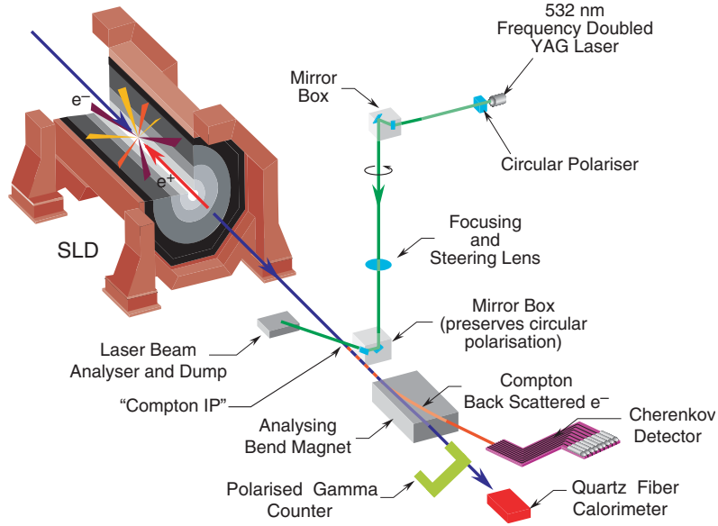
Fig. 3.1. A conceptual diagram of the SLD Compton Polarimeter. The laser beam, consisting of 532 nm wavelength 8 ns pulses produced at 17 Hz and a peak power of typically 25 MW, were circularly polarised and transported into collision with the electron beam at a crossing angle of 10 mrad approximately 30 m from the IP. Following the laser/electron-beam collision, the electrons and Compton-scattered photons, which are strongly boosted along the electron beam direction, continue downstream until analysing bend magnets deflect the Compton-scattered electrons into a transversely-segmented Cherenkov detector. The photons continue undeflected and are detected by a gamma counter (PGC) and a calorimeter (QFC) which are used to cross-check the polarimeter calibration.
