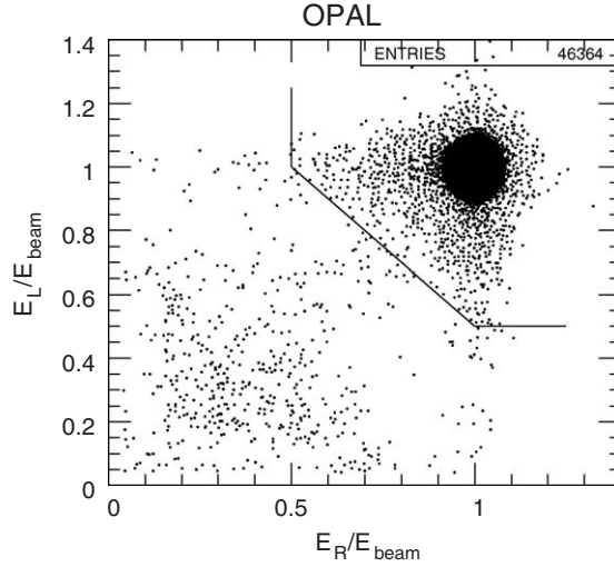
Fig. 2.2. Fraction of the beam energy observed in the left and right luminosity calorimeters of the OPAL experiment, after all cuts except the one on the deposited energies. The lines indicate the acceptance region for the signal events. Initial state photon radiation leads to tails towards lower deposited energies. Background events from accidental coincidences populate the low-energy regions in both calorimeters.
