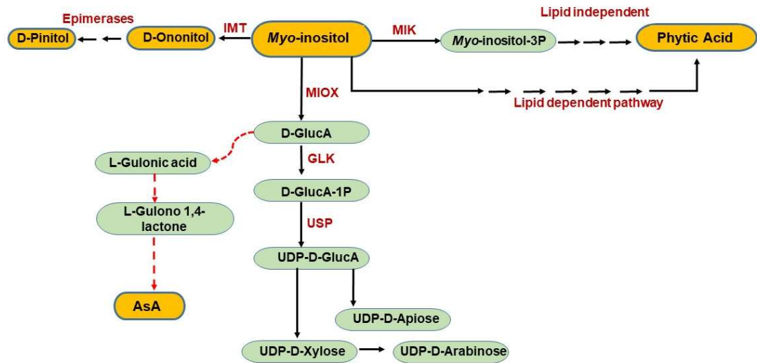
Figure 1: Myo-inositol oxidation pathway and its interconnection to other pathways. The pathways towards L-ascorbic acid are represented with dot line, which is active in the animal system, whereas in plants it exists or not is in debate. The pathway towards cell wall biosynthesis is active in the plant system. The myo-inositol catalyzed into D-GlucA (D-glucuronic acid) by MIOX (myo-inositol oxygenase). D-GlucA converted into D-GlucA-1P (D-glucuronic acid- 1-phosphate) with the help of GLK (glucuronokinase). , D-GlucA-1P further catalyzed into UDP-D-GlcA by USP (UDP-sugar pyrophosphorylase). UDP-D-GlcA is an important precursor of numerous cell wall polysaccharides i.e. UDP-D-GaIA (UDP-D-galacturonic acid), UDP-D-xylose, UDP-D-apiose, and UDP-D-Arabinose. IMT - inositol methyltransferase. Myo-inositol kinase (MIK).
