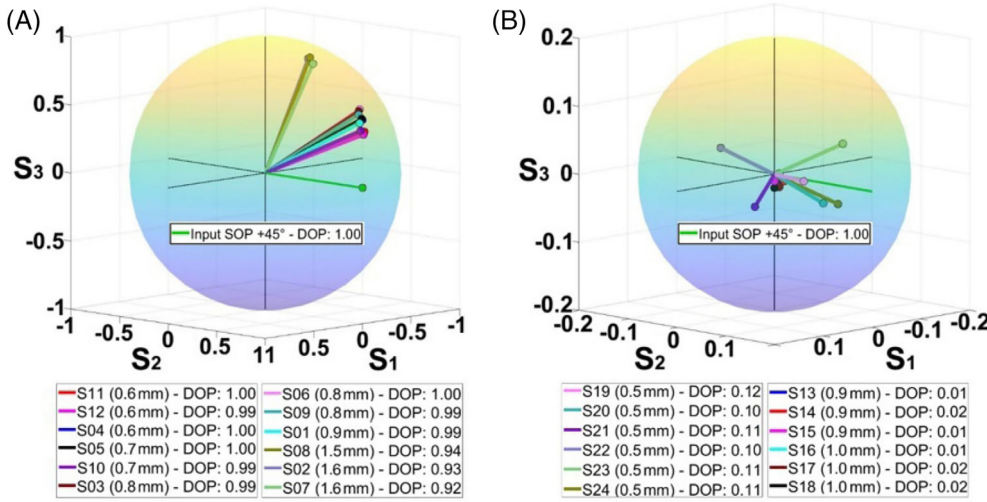
FIGURE 5 Stokes vectors representation on the Poincaré sphere for experiments conducted in lobster (A) and rat sciatic (B) nerves. The incident light on sample is linearly polarized at +45^\circ with DOP = 1.00 (green vector). The color labels in (A) and (B) are organized based on the nerve diameter, from the thinnest to the thickest. The Stokes parameters for all samples ( S_i ) are reported in the Table S1)
