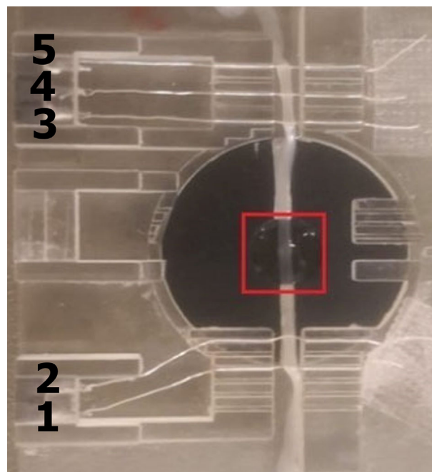
FIGURE 2 NC with the stimulation and recording electrodes placed in the grooves and a lobster nerve (first rostral leg) in the middle channel. The electrodes distribution is (1) anode, (2) cathode, (3) GND, (4) CNAP+ and (5) CNAP-. The section of the sample illuminated and its surroundings (red box) are wet with Ringer solution
