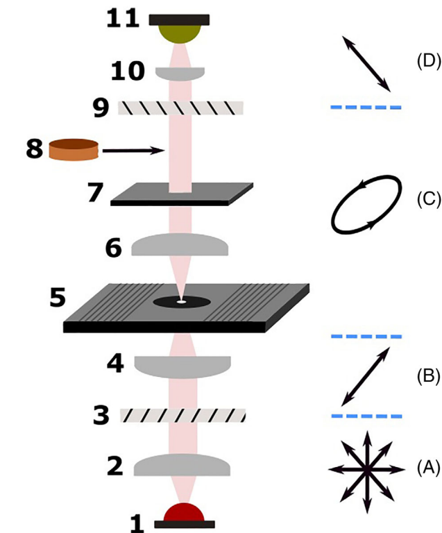
FIGURE 3 Schematic of the setup. The optical components are housed in a vertical cage mount. On top, a metallic box contained the optical channel: PD, filters and amplifier stages. LED (1). Collimation lens (2). Polarizer (3). Focusing lens (4). NC with the pinhole and the grooves for the electrodes (5). Collimation lens (6). Slit (7). Quarter waveplate (8) inserted in the optical system for the Stokes parameters measurement. Analyzer (9). Focusing lens (10). PD (11). Unpolarized light (A). Linear polarization +45^\circ (B). Elliptical polarization (C). Linear polarization -45^\circ (D)
