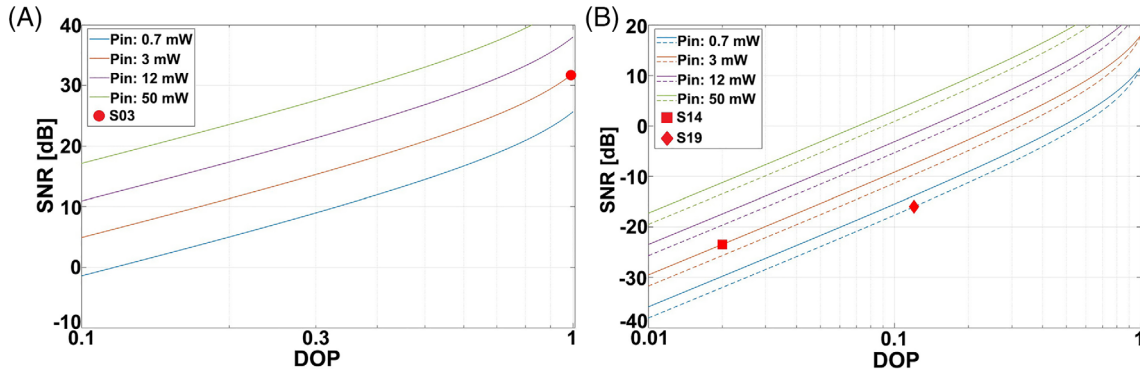
FIGURE 7 Variation of the SNR with the DOP for several optical powers ( P_{in} ) from Equation (10), with parameters corresponding to our experiments with lobster and rat sciatic nerves. The receiver bandwidth is 890 Hz. (A) Lobster (S03). The sample exhibited \phi_R = 0.6 rad, \Delta\phi = 57 \mu rad, DOP = 0.99 and \beta T_u = 0.19 ( P_{in} = 3 mW, P_{out} = 570 \mu W). (B) Rat (main nerve trunk S14 and peroneal branch S19). For the main trunk (solid): DOP = 0.02 and \beta T_u = 0.008 ( P_{in} = 3 mW, P_{out} = 25 \mu W); for the peroneal branch (dashed): DOP = 0.12 and \beta T_u = 0.015 ( P_{in} = 0.7 mW, P_{out} = 10 \mu W). In these plots, we assumed a resting retardance and a retardance variation corresponding to lobster nerves of similar thickness, that is, in the main trunk \phi_R = 0.6 rad, \Delta\phi = 57 \mu rad and in the peroneal branch \phi_R = 0.48 rad, \Delta\phi = 40 \mu rad. We note that despite the smaller \beta T_u coefficient, the SNR is expected to be slightly larger in the main trunk because of a higher \phi_R and \Delta\phi . The red dot in (A) indicates the experimental SNR, while the red marks in (B) show the theoretical SNR with the corresponding experimental parameters
