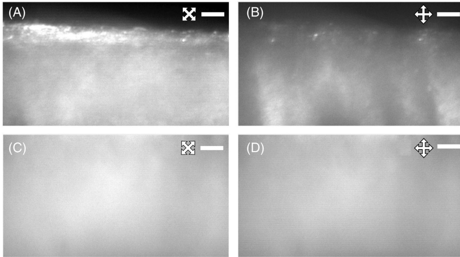
FIGURE 6 Cross-polarized images of the peroneal branch of a rat sciatic nerve. The sample is oriented at 45^\circ (A–C) or aligned (B–D) with the axes of the polarizers. The scale bar corresponds to 50 \mu\text{m} and the cross represents the orientation of the polarizer and the analyzer. (A) and (B) Edge of the nerve, the average brightness in B is \approx 24\% smaller than in (A). (C) and (D): Central part of the nerve, the average brightness in (D) is \approx 11\% smaller than in (C)
