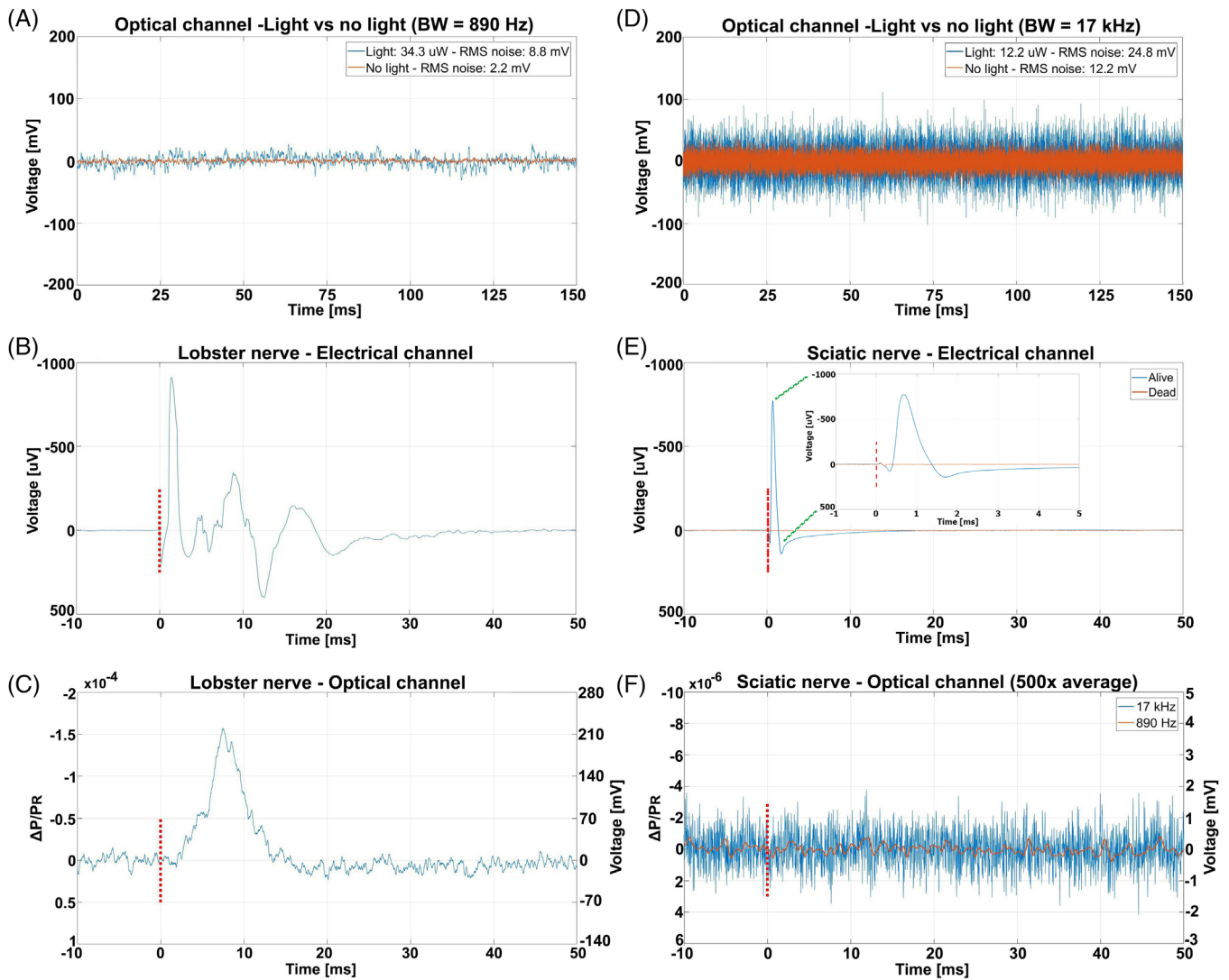
FIGURE 4 Typical electrical and optical recordings in lobster walking leg nerves (left column, S01) and rat sciatic nerves (right column, S14). Both samples exhibited similar thickness ( \approx 0.9 \text{ mm} ). (A) and (D) signal recorded at the output of the optical channel, without and with incident light in the resting state, showing shot noise limited measurements in both experiments. The power reaching the PD is \approx 34 \mu\text{W} and \approx 12 \mu\text{W} , respectively. (B) and (E) Electrical CNAPs. The voltage amplitude refers to the input of the electrical channel. (C) and (F), recordings in the optical channel. A raw single trace is shown for the experiment in lobster nerve, while an average over 500 trials is displayed for rat SN. Despite numerical filtering (890 Hz bandwidth and averaging), no birefringence signal can be seen
