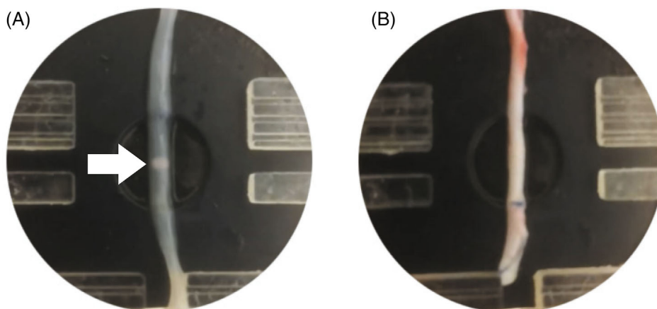
FIGURE 1 (A) Lobster walking leg nerve. (B) Rat sciatic nerve, main trunk. Both samples have the same thickness ( \approx 0.9 mm). The 1 mm diameter pinhole over which the nerves are placed can be seen as a white dot in A (white arrow), thanks to the relative transparency of the crustacean sample. This is not the case in (B), due to the opacity of the nerve
