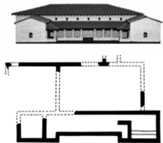
Reconstruction drawing and model of the Gallo-Roman villa in Jette, third century AD
