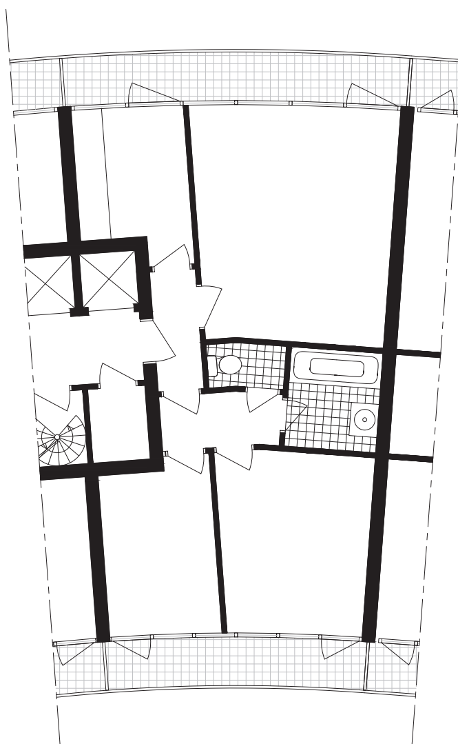
Unit plan 1:100
