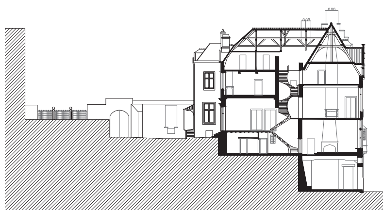
Cross section 1:500
