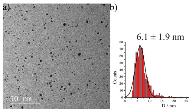
Fig. 1 TEM micrograph and the corresponding particle core size histogram of gold nanoparticles synthesized in the presence of the calix[4]arene 2 to give AuNPs 3a .
