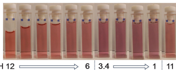
Fig. 2 The change in color of a colloidal dispersion of AuNPs 3c in HEPES buffer adjusted to various pH values. The dispersion is stable upon addition of HCl from pH 12 down to pH 6 ( \lambda_{\text{max}} shifts from 522 to 527 nm), while from pH 3.4 to 1 the \lambda_{\text{max}} shifts from 536 to 543 nm and the absorption broadens, resulting in a purple color. These effects are reversed upon addition of NaOH to get to pH 11 ( \lambda_{\text{max}} 526 nm).
