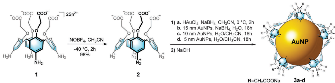
Scheme 1 Synthesis of calix[4]arene-tetra-diazonium salt 2 and AuNPs 3a . AuNPs 3b–d were obtained by grafting 2 onto citrate-protected particles.
