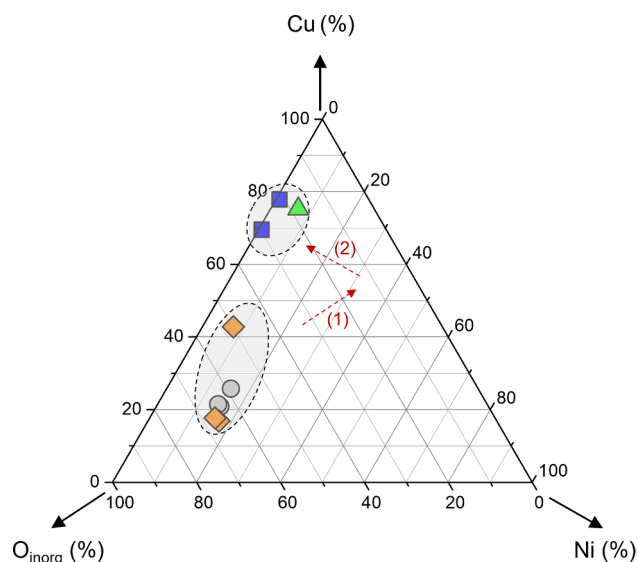
Fig. 5. Ternary diagrams presenting the sums of mole fractions determined by XPS: elements related to the inorganic matter Cu, Ni and inorganic oxygen ( O_{inorg} ) on 90Cu-10Ni samples after immersion in SFW (●), H 2 O 2 (◆), GAc (▲) and GOx (■). O_{inorg} was computed using Eq. (6) and O_{org} using Eq. (3).
