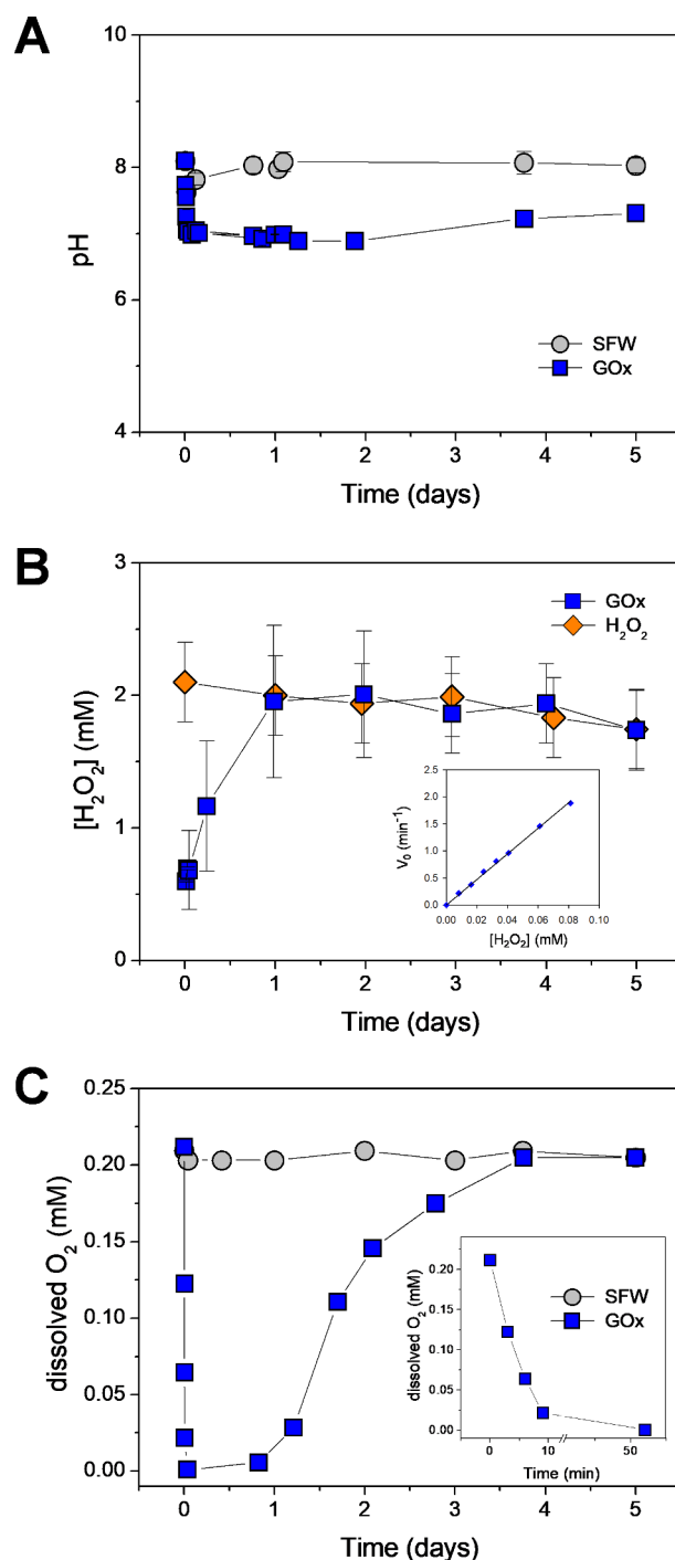
Fig. 1. Evolution of (A) pH, (B) concentration of \text{H}_2\text{O}_2 , [\text{H}_2\text{O}_2] , and (C) dissolved \text{O}_2 as function of time during 5 days in (●) SFW, (◆) \text{H}_2\text{O}_2 and (■) GOx media, as indicated. (B, inset) relationship between the activity of peroxidase (initial velocity V_0 ) and the concentration of \text{H}_2\text{O}_2 .
