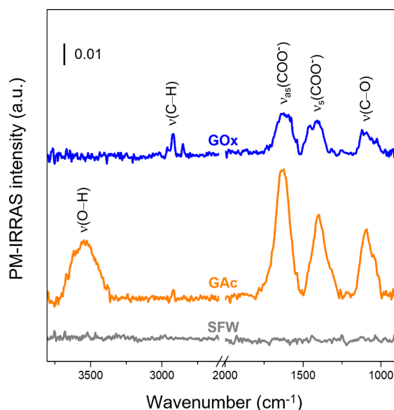
Fig. 8. PM-IRRAS spectra recorded on 90Cu-10Ni samples after immersion period of 5 days in SFW, GAc and GOx, as indicated.
