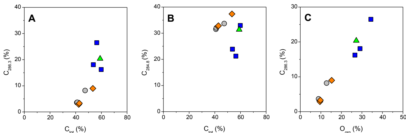
Fig. 7. Relationship between molar concentrations measured by XPS recorded on 90Cu-10Ni samples after immersion in SFW (●), H 2 O 2 (◆), GAc (▲) and GOx (■). \text{O}_{\text{org}} was computed using Eq. (3): (A) \text{C}_{286.3} vs \text{C}_{\text{tot}} , (B) \text{C}_{284.8} vs \text{C}_{\text{tot}} , (C) \text{C}_{286.3} vs \text{O}_{\text{org}} .
