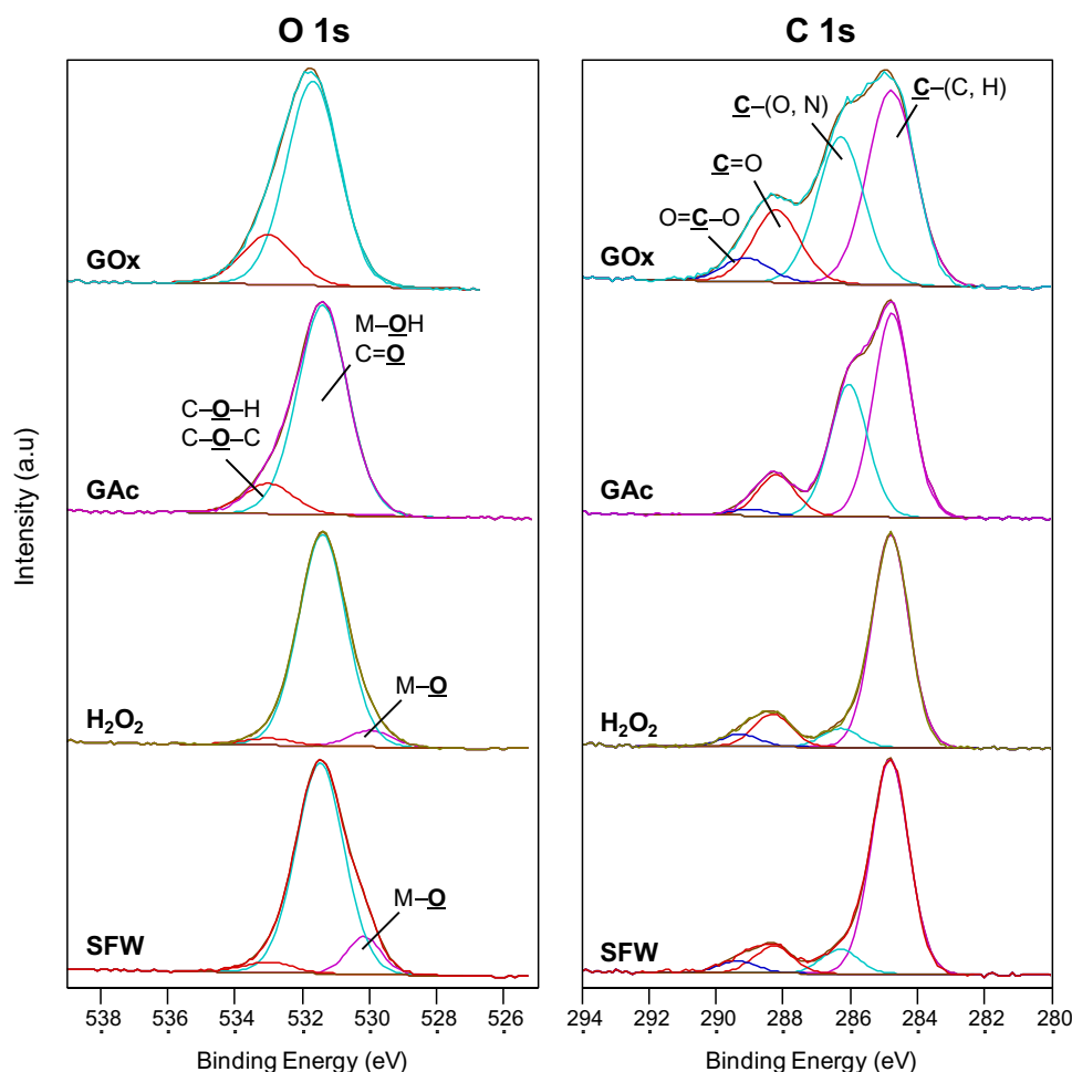
Fig. 2. Representative O 1s and C 1s peaks recorded on 90Cu-10Ni samples after immersion period of 5 days in the different media: SFW, \text{H}_2\text{O}_2 , GAc and GOx.
