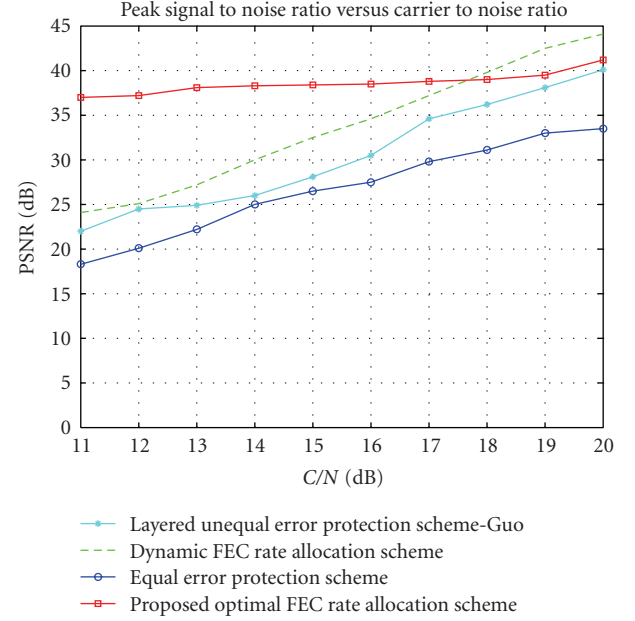
FIGURE 14: PSNR versus carrier-to-noise ratio.
