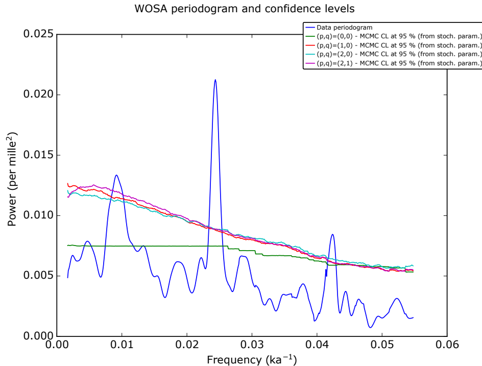
Figure 12. The weighted WOSA periodogram and its 95 % confidence levels for different orders (p, q) of the CARMA process. Note that the marginal posterior distributions of some parameters of the CARMA(2,0) and CARMA(2,1) processes are multimodal, so the analytical approach cannot be applied, and MCMC confidence levels must therefore be used.
