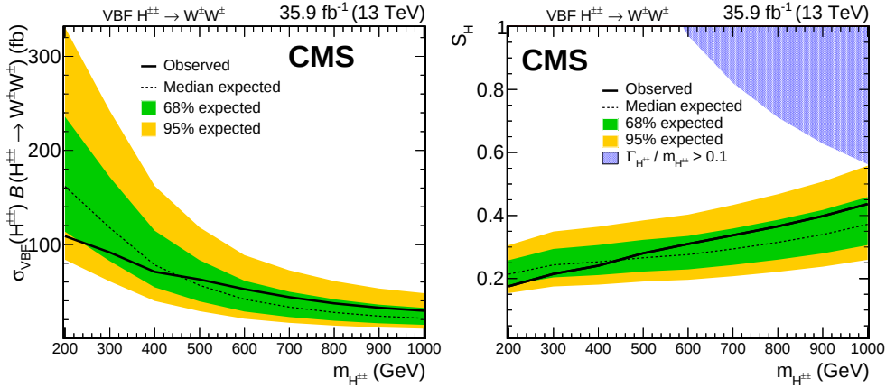
Figure 3: Expected and observed 95% CL upper limits on the cross section times branching fraction, \sigma_{\text{VBF}}(H^{\pm\pm}) B(H^{\pm\pm} \rightarrow W^{\pm}W^{\pm}) (left) and on s_H in the Georgi–Machacek model (right) as a function of doubly charged Higgs boson mass. The blue area in the upper-right corner covers the region where the model is not applicable [39].
