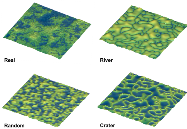
Fig. 1. Detail of the four microtopography types ( 2\text{ m} \times 2\text{ m} ) with depressions partially filled with water (in blue) in order to highlight the contrasting connectivities.
