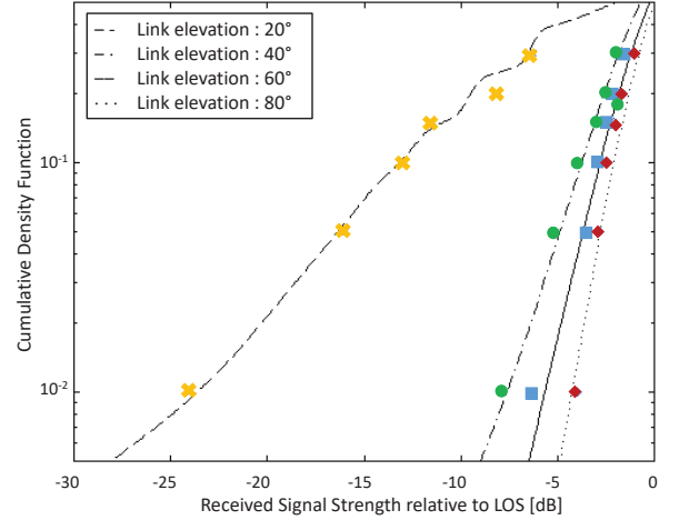
Fig. 2. Comparison between simulation (dashed, dot-dashed, solid and dot lines) and experimental (crosses, circles, squares and diamonds) results at various elevation angles.
