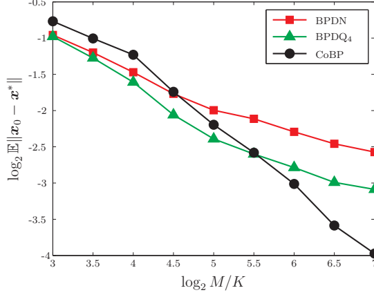
(a) Gaussian QCS of sparse signals.
