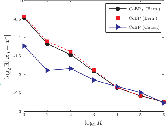
(b) Bernoulli vs Gaussian QCS of sparse signals.
