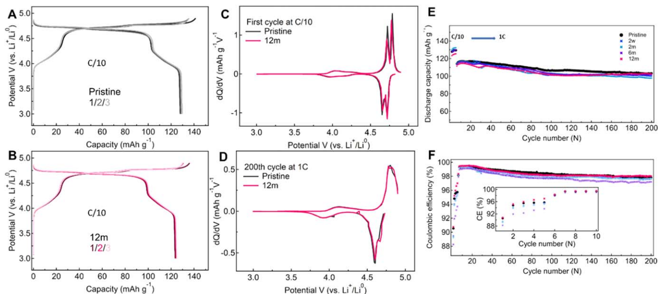
Figure 4. Galvanostatic charge-discharge potential profiles as a function of the specific capacity of the first three cycles for LNMO electrodes cycled in a lithium cell at a rate of C/10 ( 1\text{C} = 147 \text{ mAh g}^{-1} ) for (A) pristine sample and (B) sample exposed for 12 months. (C) The corresponding dQ/dV differential capacity plots at the first cycle, and (D) dQ/dV plots of the 200th cycle at a rate of 1C. Cycling stability test for the pristine LNMO and all the air exposed samples: (E) specific discharge capacity and (F) coulombic efficiency vs cycle number.
