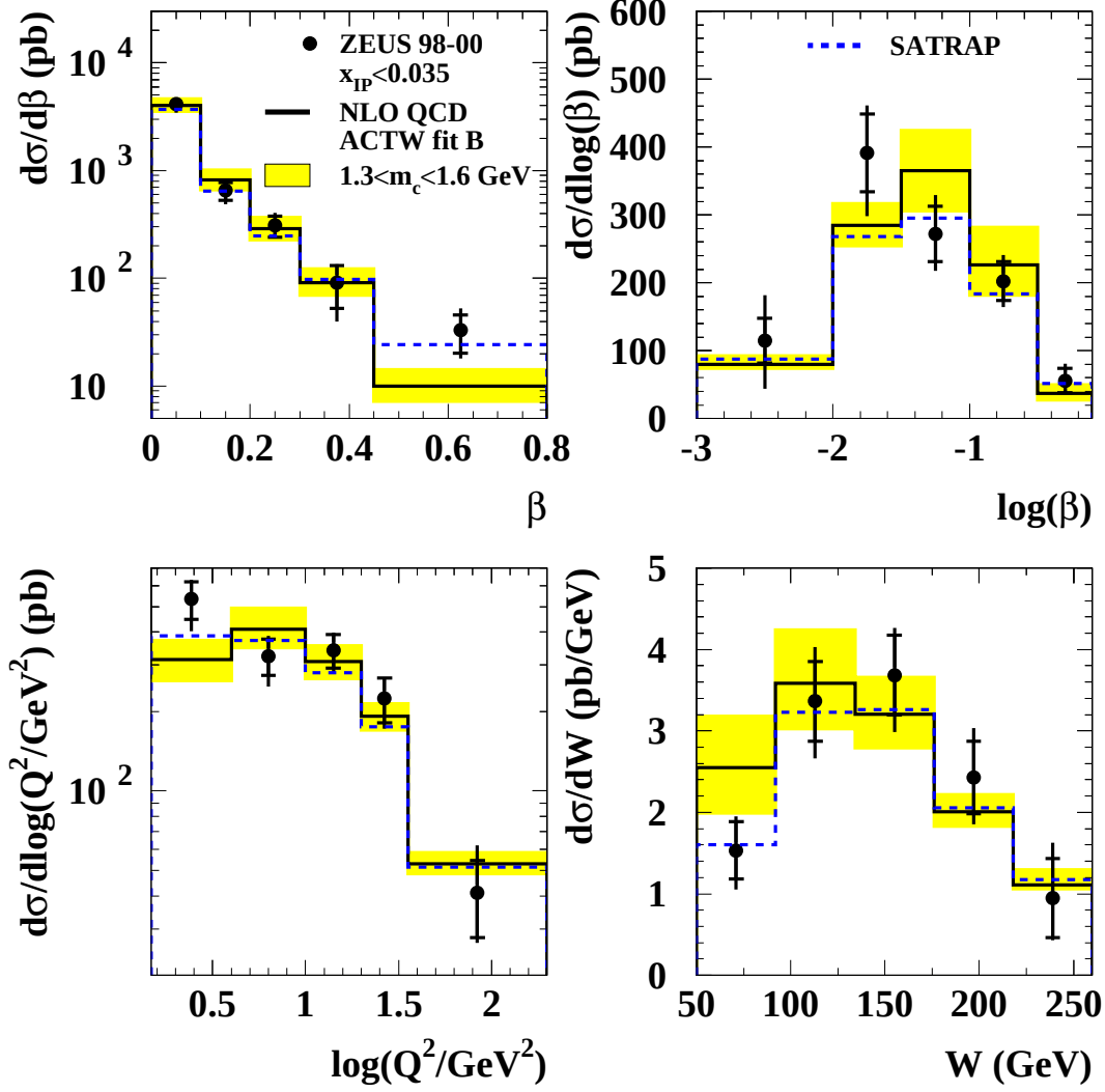
Figure 9: Differential cross sections for diffractive D^{*\pm} production with x_{\mathbb{P}} < 0.035 for the data (dots) compared with the ACTW NLO (solid histogram) and SATRAP (dashed histogram) predictions. The shaded area shows the effect of varying the charm-quark mass in the ACTW NLO prediction. The cross sections are shown as a function of \beta , \log(\beta) , \log(Q^2) and W . The inner error bars indicate the statistical uncertainties, while the outer ones correspond to statistical and systematic uncertainties added in quadrature. The overall normalisation uncertainties arising from the luminosity measurement ( \pm 2.2\% ), from the D^{*\pm} and D^0 branching ratios ( \pm 2.5\% ) and from the proton-dissociative background subtraction ( \pm 4.9\% ) are not indicated.
