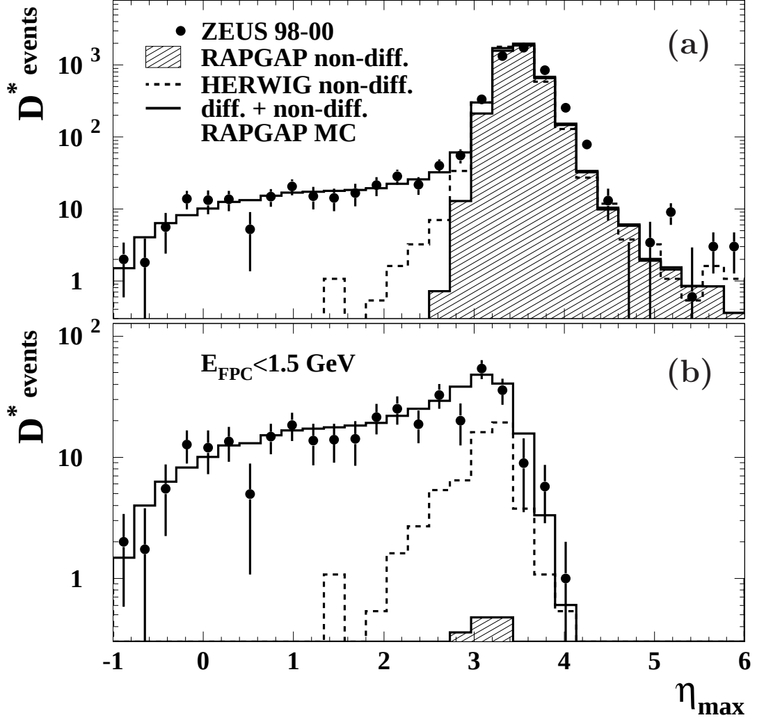
Figure 2: Numbers of reconstructed D^{*\pm} mesons (dots) as a function of \eta_{\max} for DIS events with (a) any E_{\text{FPC}} values and (b) E_{\text{FPC}} < 1.5 \text{ GeV} . The solid histogram shows the sum of the non-diffractive RAPGAP MC (hatched area) and the diffractive RAPGAP MC. The sum was normalised to have the same area as the data. The dashed histogram shows the non-diffractive HERWIG MC.
