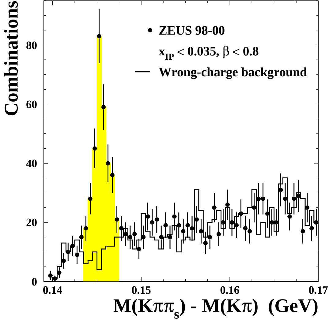
Figure 3: The distribution of the mass difference, \Delta M = M(K\pi\pi_s) - M(K\pi) , for D^{*\pm} candidates (dots) in events with \eta_{\text{max}} < 3 , E_{\text{FPC}} < 1.5 \text{ GeV} , x_{\text{IP}} < 0.035 and \beta < 0.8 . The histogram shows the \Delta M distribution for wrong-charge combinations. Only D^{*\pm} candidates from the shaded band were used for the differential cross-section measurements.
