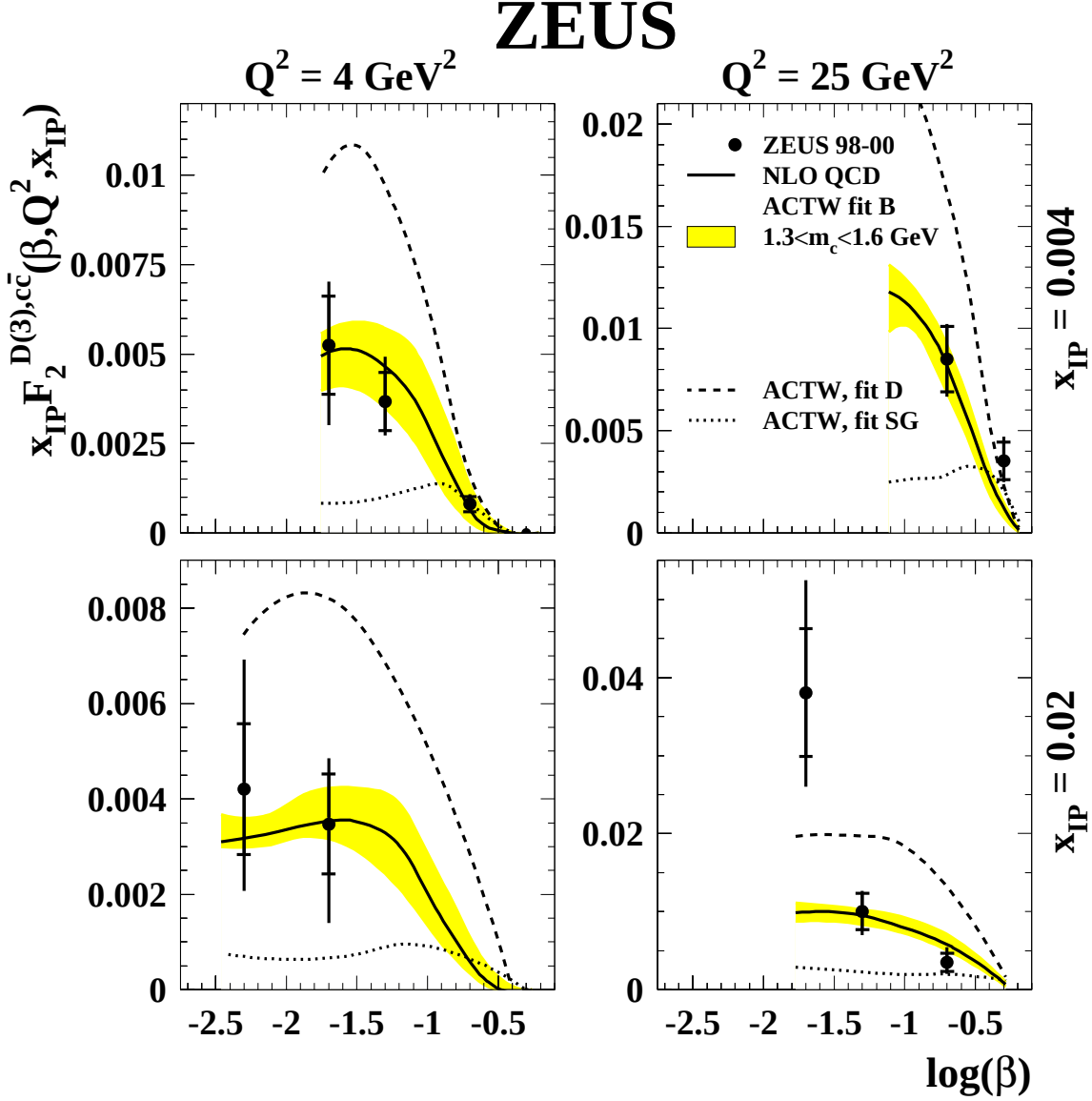
Figure 11: The measured charm contribution to the diffractive structure function of the proton multiplied by x_P , x_P F_2^{D(3),c\bar{c}} , as a function of \beta for different values of Q^2 and x_P (dots). The inner error bars indicate the statistical uncertainties, while the outer ones correspond to statistical and systematic uncertainties added in quadrature. The overall normalisation uncertainties arising from the luminosity measurement ( \pm 2.2\% ), from the D^{*\pm} and D^0 branching ratios ( \pm 2.5\% ) and from the proton-dissociative background subtraction ( \pm 4.9\% ) are not indicated. The curves correspond to the ACTW model prediction; the shaded area shows the effect of varying the charm-quark mass.
