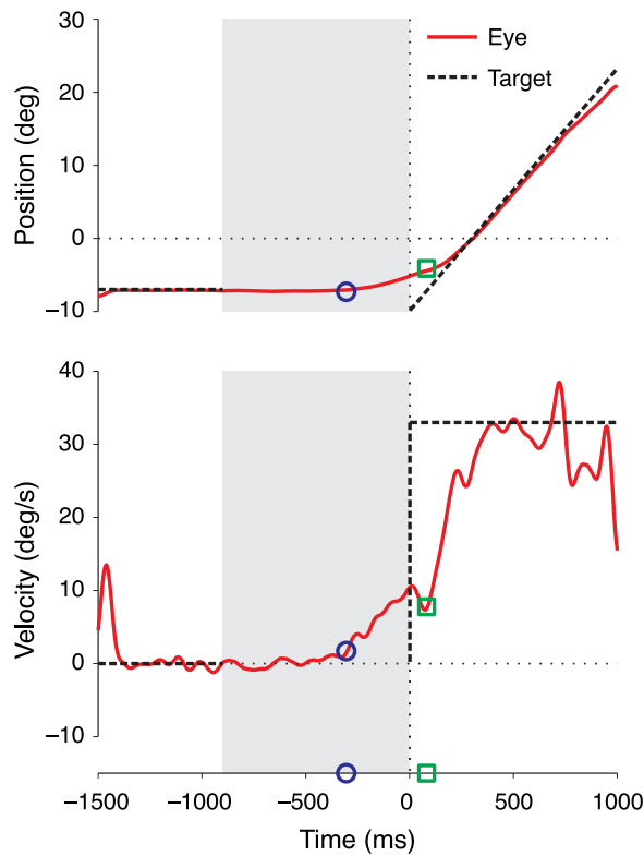
Figure 2. Sample response during the dual task for subject LM. Top panel, eye and target position. Bottom panel, eye and target velocity. The shaded region indicates the delay interval. The detected anticipatory pursuit onset (blue circle) and recorded time of the button press (green square) are marked on both eye traces as well as the x-axis.
