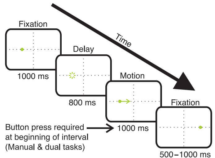
Figure 1. Experimental paradigm. A spot target appeared slightly offset to the left or right of the screen (first panel) and was fixated by the subject. The target disappeared during the delay period (second panel). After the delay in non-catch trials, the spot reappeared moving towards the center of the screen (third panel). It came to rest on the opposite side for a random amount of time (fourth panel). Only the spot was visible on the screen; the horizontal and vertical dashed lines are shown here for reference. The numbers below the panels indicate the duration of each interval.
