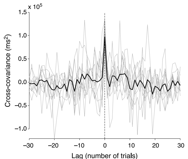
Figure 7. Cross-covariance analysis. For each trial block in the dual task the cross-covariance was computed between anticipatory pursuit onset and manual response times (light gray lines). The mean (dark line) is also shown. The single peak at lag = 0 results from trial-by-trial correlations between the two responses. Subject LM.
