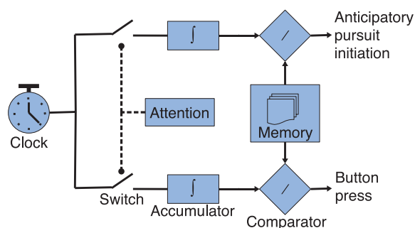
Figure 9. Timing model. The components are based on STT. The clock emits regular pulses that must pass a switch held closed by attention. Pulses that pass through are counted by the accumulator, whose value is checked against a reference stored in memory. When the accumulator and reference values are sufficiently close as determined by the comparator, a response is initiated. Insufficient attention allows the switch to open, causing pulses to be blocked. Thus it takes longer for the accumulator to reach a value close to reference memory, causing a delayed response. During a dual task both branches are active, increasing the load on the attentional component and consequently decreasing the amount of time that the switches are held closed.
