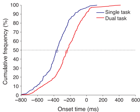
Figure 3. Anticipatory pursuit distributions. Cumulative distributions of anticipatory pursuit onset times for the single and dual tasks. The circles indicate the response mean values; response medians are indicated by the 50th percentile line. Responses occurred significantly later during the dual task. Subject EC.
