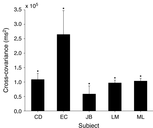
Figure 8. Summary of response correlations. Mean cross-covariance at lag = 0 between all response times, averaged over all trial blocks. Error bars indicate standard error of the between-block mean, and asterisks indicate significance as computed from the bootstrap (see Methods section). All subjects showed significant correlations between ocular and manual timing.
