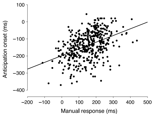
Figure 5. Linear regression of all responses. Each trial in the dual task data set is plotted as a point. The linear regression line is also shown. There is a modest correlation between the responses ( r^2 = 0.18 ). Subject LM.
