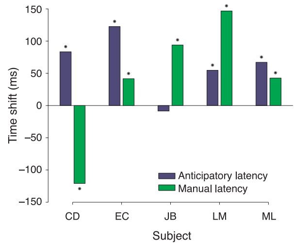
Figure 4. Summary of response time shifts for anticipatory pursuit and button-press responses. Bar height is equal to mean dual task response minus mean single task response. For four out of five subjects, the mean onset of anticipatory pursuit was shifted significantly later in time during the dual task. Four out of five subjects also showed a significantly later shift for the manual response data. Asterisks indicate significance at the 0.01 level.
