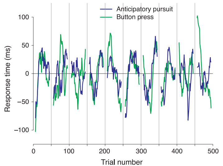
Figure 6. Responses over time. For each trial block (demarcated by the light gray lines), the mean was subtracted from the button-press responses and from the anticipatory pursuit onset times. Corresponding running averages of response times were then computed using a window size of five trials. Note the degree of correspondence between the average curves. Subject LM.
