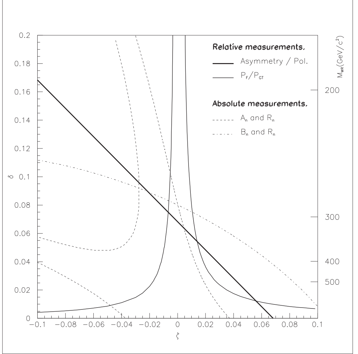
Figure 1: Comparative exclusion plots of the manifest left-right symmetric model parameters provided by various absolute and relative nuclear beta-decay tests at their present levels of precision (90% CL). R_n is the ratio of the neutron-and Fermi decay ft-values
