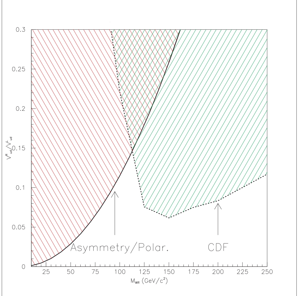
Figure 4: Exclusion-plots of the right(left)-handed Cabibbo-Kobayashi-Maskawa matrix-element ratio as a function of a (light) right-handed gauge-boson mass.
