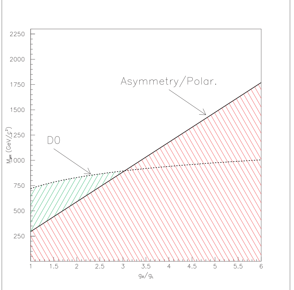
Figure 3: Right-handed gauge-boson limits (at 90% CL) deduced from collider-experiments and nuclear beta-decay of the type discussed in 2.3.2.1 (for \zeta = 0 ) as a function of the gauge-coupling ratio of the right (-left)-handed sectors.
