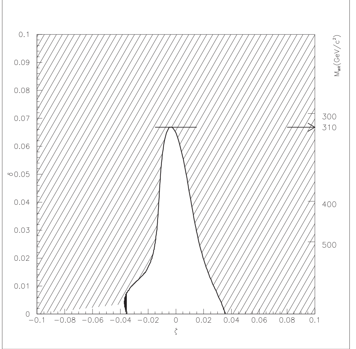
Figure 2: Combination of the constraints presented in Figure 1 on the 90 % CL. The lower limit of the right handed gauge boson mass (independently of the mixing parameter) is represented by an arrow.
