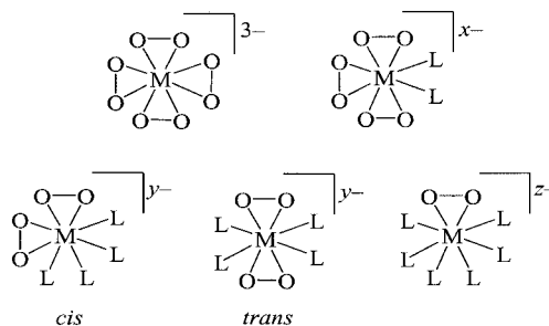
Figure 2. Schematic representation of model stoichiometries considered for the theoretical study ( \text{M} = \text{Nb}^{\text{V}} and \text{L} = oxygen atom from an oxalate ligand).
