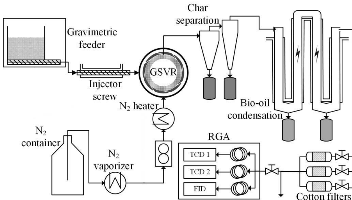
Figure 1. Flow diagram of the Gas-Solid Vortex Reactor (GSVR) demonstration unit for biomass fast pyrolysis.
