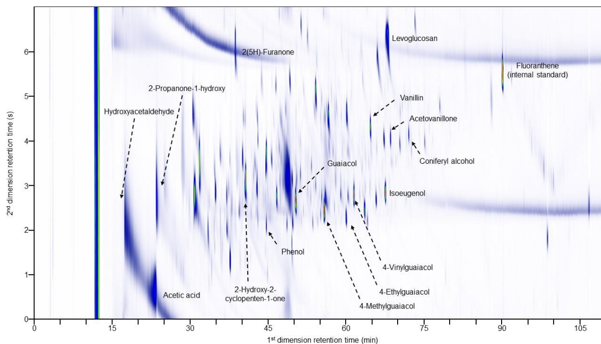
Figure 7. GC×GC-FID chromatogram of pine bio-oil. Some representative compounds are pointed out.
