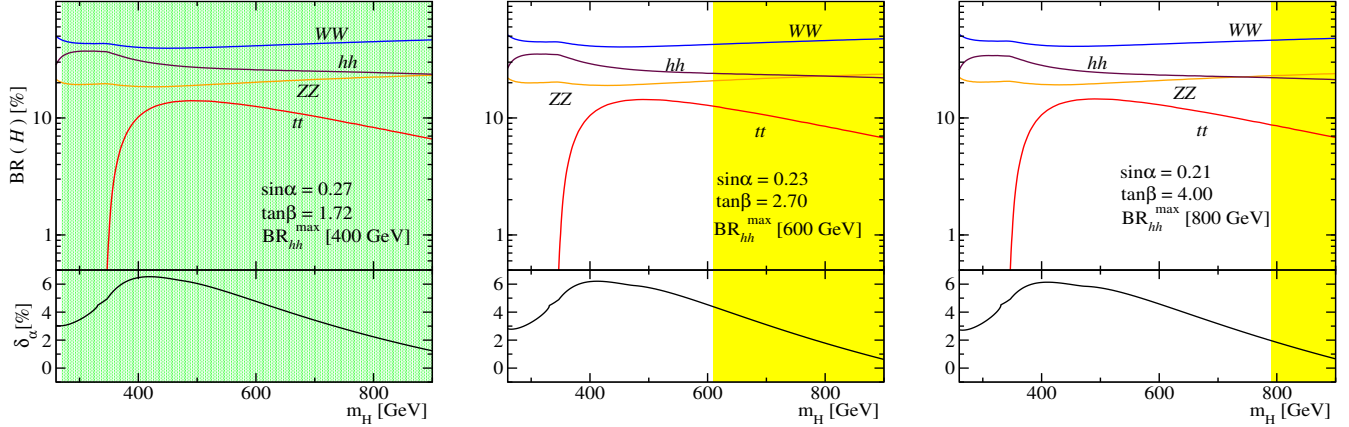
Figure 6: Heavy Higgs branching ratios (in %) as a function of the heavy Higgs mass in the high-mass region. The mixing angle and \tan\beta values are fixed in each panel such that they maximize the H \rightarrow hh branching ratio at LO for a given heavy Higgs mass of 400 (left), 600 (center) and 800 GeV (right) [90]. Decay modes into light fermions and loop-induced decays into gauge bosons lie below \mathcal{O}(0.1)\% and are not shown. The lower subpanels show the relative one-loop EW correction ( \alpha_{\text{em}} parametrization (76)) to \Gamma_{H \rightarrow hh}^{\text{LO}} for the same parameter variations. The shaded (green) area in the left plot is ruled out by the W-mass measurement. Excluded regions in the central and right panels (in yellow) are incompatible with perturbativity and m_W .
