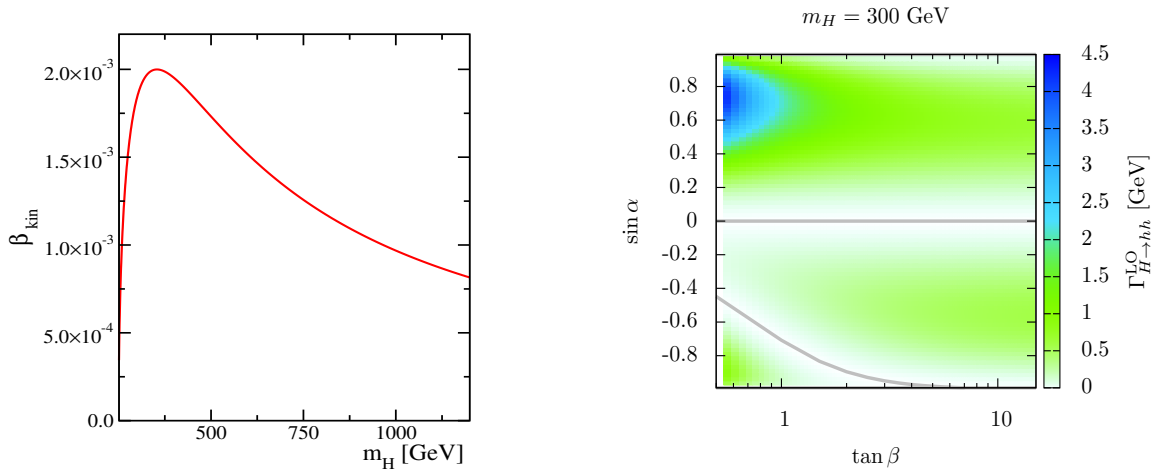
Figure 2: Left panel : kinematical factor \beta_{\text{kin}} = \sqrt{1 - 4m_h^2/m_H^2} as a function of the heavy Higgs mass, for m_h = 125.09 GeV. Right panel : leading-order heavy-to-light Higgs decay width \Gamma_{H \rightarrow hh}^{\text{LO}} [in GeV] over the \sin \alpha - \tan \beta plane for a fixed heavy Higgs mass of m_H = 300 GeV. The grey lines signal the configurations \sin \alpha = 0 and \tan \beta = -\tan \alpha along which \Gamma_{H \rightarrow hh}^{\text{LO}} vanishes.
