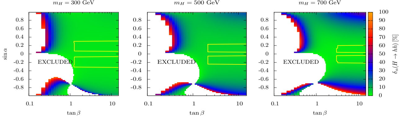
Figure 5: Relative one-loop EW corrections in the \alpha_{\text{em}} -parametrization (76), projected on the \sin \alpha - \tan \beta plane for exemplary heavy Higgs masses in the high-mass region. The white voids correspond to regions with \delta_\alpha \gtrsim 100\% . Renormalization is performed in the improved on-shell scheme. The yellow contour separates the allowed and excluded regions in the parameter space.
