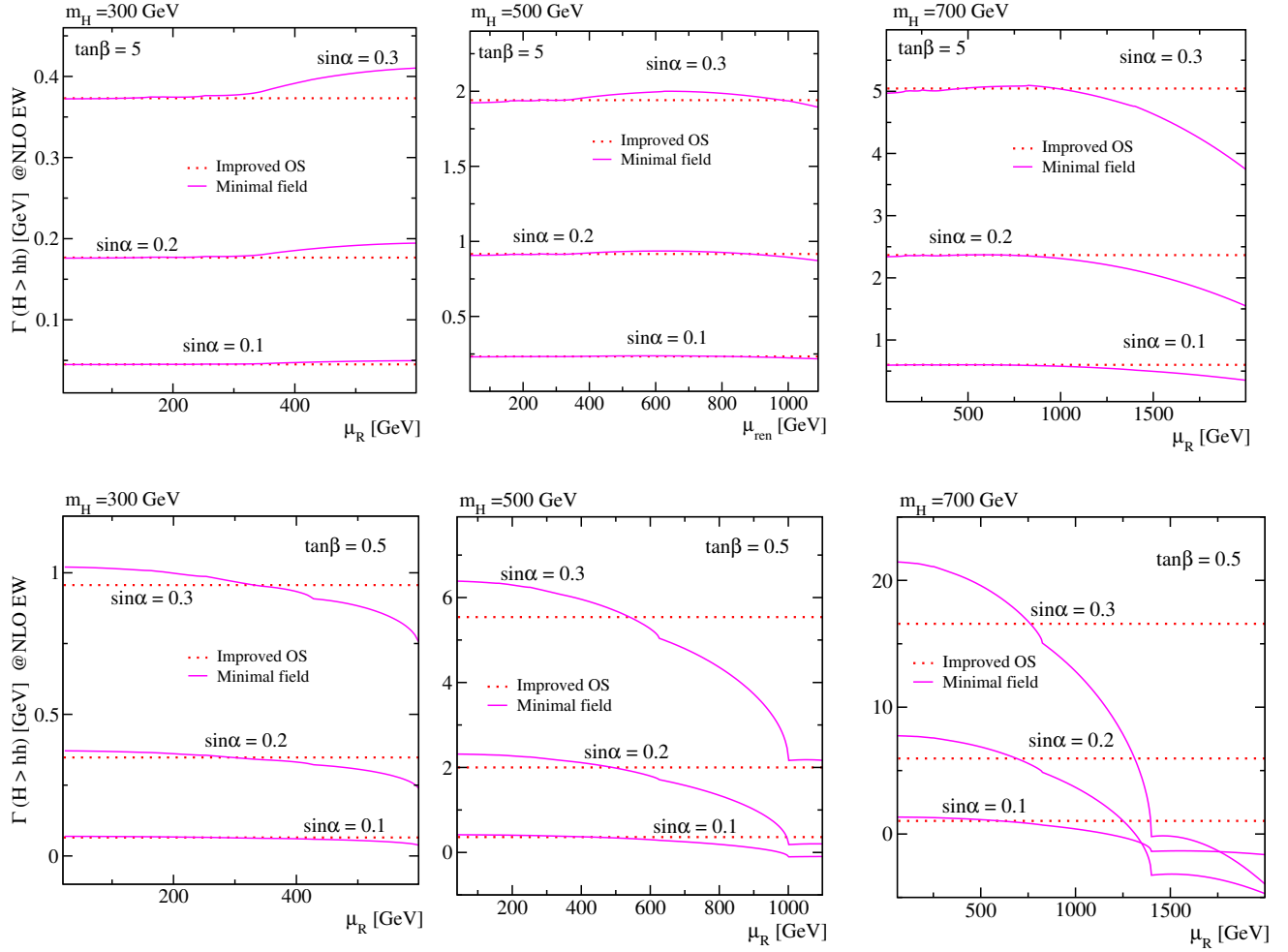
Figure 7: NLO decay width \Gamma_{H \rightarrow hh}^{\text{NLO}} as a function of the renormalization scale in the high-mass region, for exemplary heavy Higgs masses, mixing angles, and \tan\beta choices. The scale-dependent predictions for the minimal field scheme are represented by the solid (magenta) lines. The scale-independent reference value (dotted, red lines) we obtain in the improved OS scheme. Parameter space constraints are not shown.
