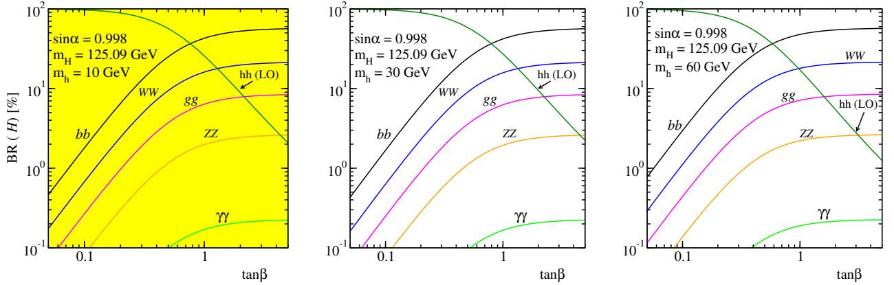
Figure 11: Heavy Higgs branching ratios (in %) as a function of \tan \beta in the low-mass region. The results are shown for representative light Higgs mass values, with fiducial mixing angle \sin \alpha = 0.998 . The whole parameter space region shown in the left panel is excluded by perturbative unitarity.
