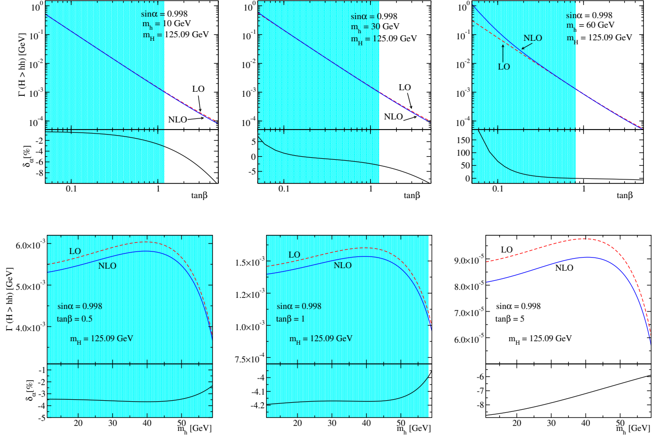
Figure 8: Heavy-to-light Higgs boson width \Gamma_{H \rightarrow hh} in the low-mass region. The results are shown at LO (dashed, red) and NLO (full, blue) as a function of the relevant parameters of the model. The mixing angle is fixed to \sin \alpha = 0.998 in all cases. The lower subpanels show the relative EW one-loop correction in the \alpha_{\text{em}} -parametrization (76). Renormalization is performed in the improved on-shell scheme. The shaded areas in the low \tan \beta and m_h ranges are ruled out by the LHC Higgs signal strength measurements.
