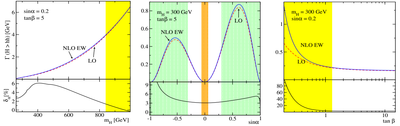
Figure 4: Heavy-to-light Higgs decay width \Gamma_{H \rightarrow hh} in the high-mass region. The results are shown at LO (dashed, red) and NLO (full, blue) as a function of the relevant parameters of the model. The lower subpanels show the relative one-loop EW correction in the \alpha_{\text{em}} -parametrization (76). Renormalization is performed in the improved on-shell scheme. The shaded regions are excluded by constraints (see the text for more details).
