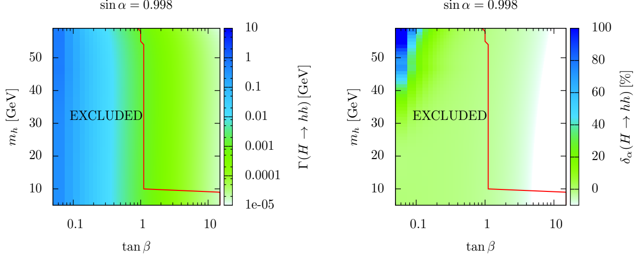
Figure 9: Loop-corrected partial H \rightarrow hh width (left panel) and relative one-loop EW corrections \delta_\alpha in the \alpha_{\text{em}} -parametrization (76), projected on the m_h - \tan\beta plane in the low-mass region. The mixing angle is fixed to the fiducial choice \sin\alpha = 0.998 . Renormalization is performed in the improved on-shell scheme. The regions on the left and below the red contour are excluded by constraints. The strong exclusion in the low mass region follows from direct LEP searches [134].
