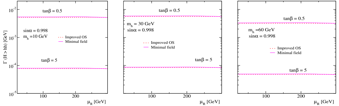
Figure 10: NLO decay width \Gamma_{H \rightarrow hh}^{\text{NLO}} as a function of the renormalization scale in the low-mass region, for exemplary heavy Higgs masses and \tan\beta values. The mixing angle is fixed to \sin\alpha = 0.998 . The scale-dependent predictions for the minimal field scheme are represented by the solid (magenta) lines. The scale-independent reference value (dotted, red lines) we obtain in the improved OS scheme. Parameter space constraints are not shown.
