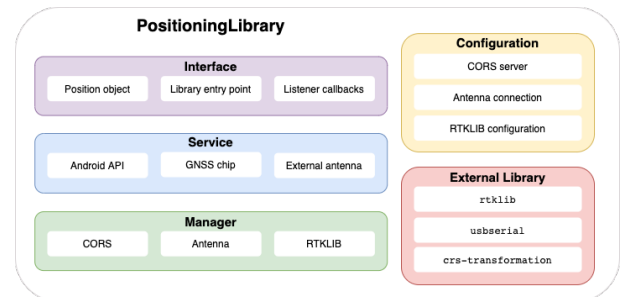
FIGURE 9: OPENPosLIB Architecture
