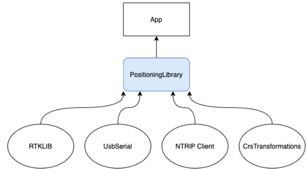
FIGURE 8: Libraries encapsulated by OPENPosLIB
