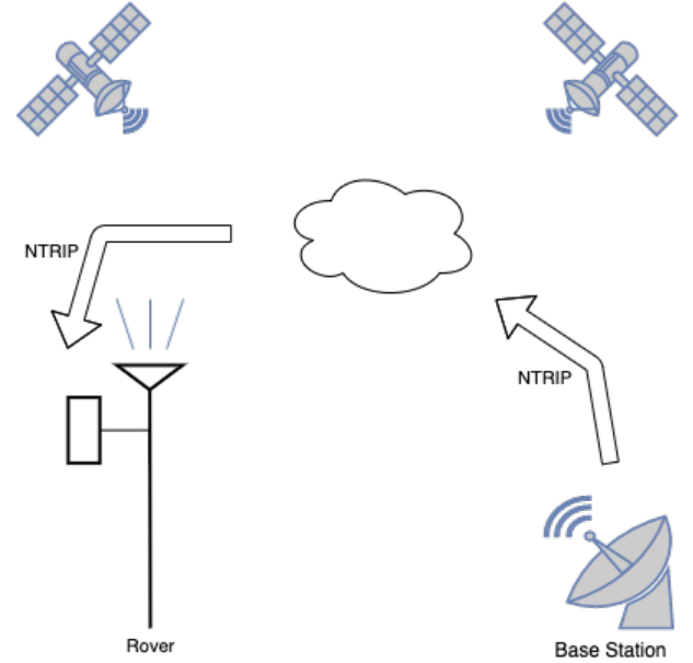
FIGURE 11: Setup of the experiment with NTRIP
