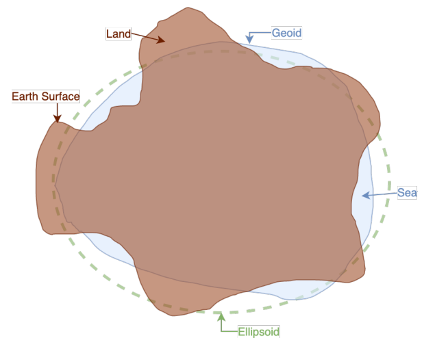
FIGURE 3: Differences between ellipsoid and geoid models of Earth
