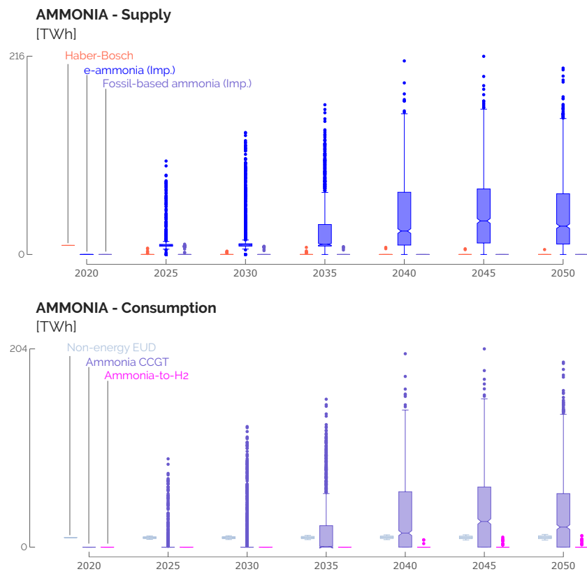
Figure D.3. Distribution of the different streams of supply (top) and consumption (bottom) of ammonia from the Global Sensitivity Analysis (GSA).
