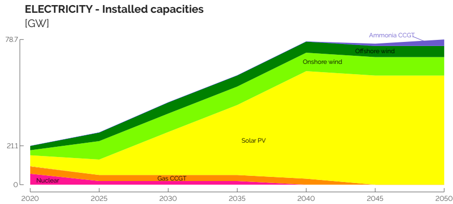
Figure C.3. The electrical production capacity will experience a massive expansion of wind turbines (onshore and then offshore) and a soaring installed capacity of PV. Ammonia CCGT are installed at the end of the transition to provide a flexible capacity as gas CCGT are phased out.
