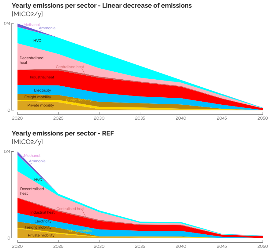
Figure C.11. Respecting the CO 2 budget imposed in the REF case drastically cuts the emissions of the system, especially in the production of High-Value Chemicals (HVC) and the high-temperature heating sector.
