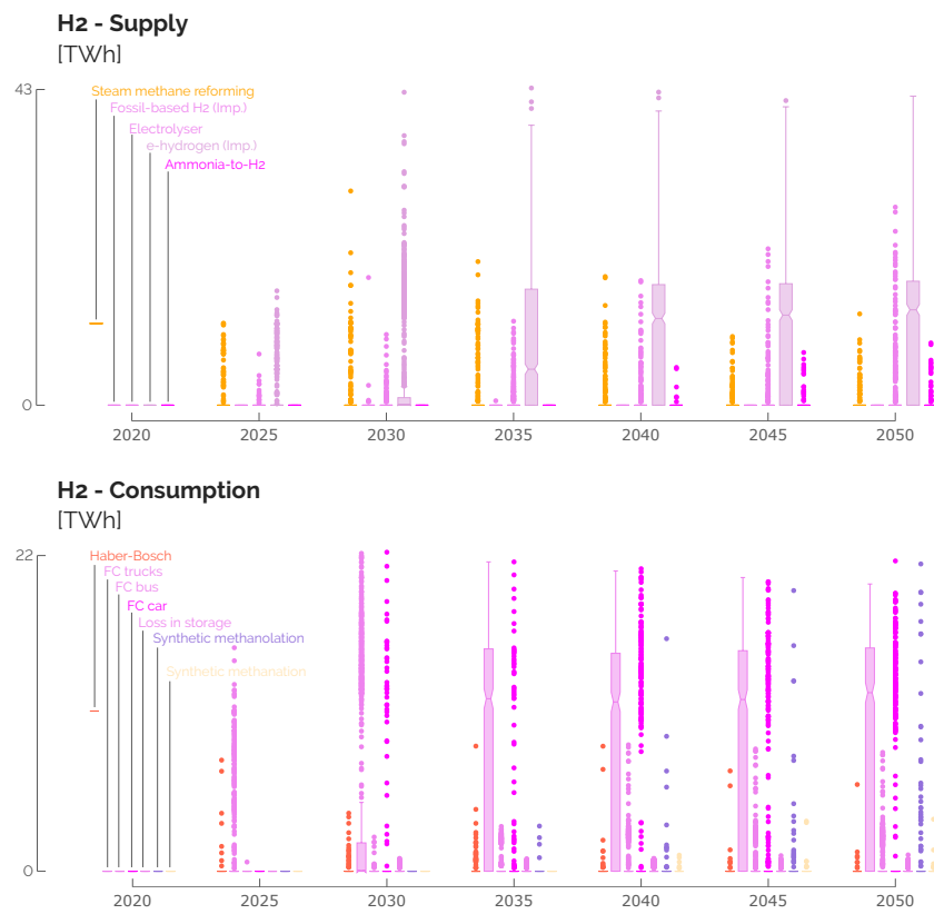
Figure D.2. Distribution of the different streams of supply (top) and consumption (bottom) of hydrogen from the Global Sensitivity Analysis (GSA).
