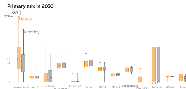
Figure E.4. Comparison of the primary energy mix in 2050 from the RL-based myopic optimisation on the hourly and monthly models. To a lesser extent than the hourly model, the monthly optimisation also captures the need to import more electrofuels when the foresight is limited.
