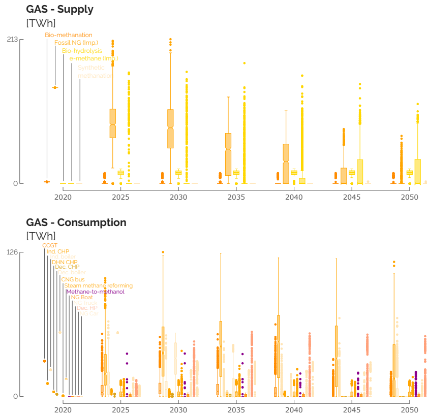
Figure D.1. Distribution of the different streams of supply (top) and consumption (bottom) of methane from the Global Sensitivity Analysis (GSA).
