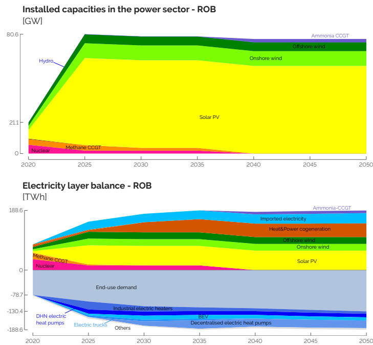
Figure 5.4. Installed capacities and layer balance of the power sector in the ROB case. Compared to the REF case, local VRES are deployed as soon as possible supported by an earlier electrification of the heat and transport sectors. CHP units also represent a higher share of the electricity supply given their higher efficiency at the expense of other flexible production units like ammonia-CCGT.
