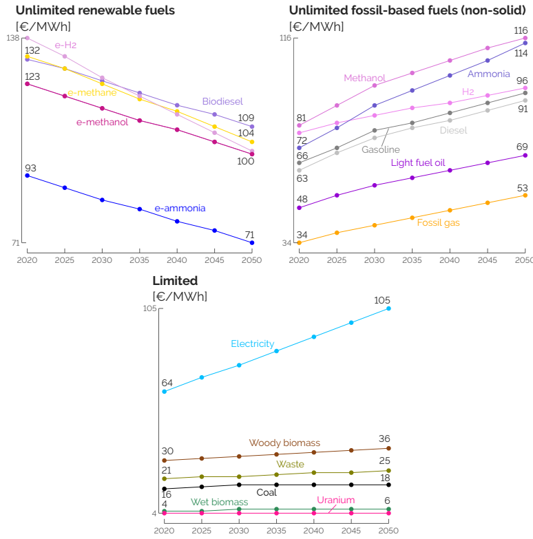
Figure 2.3. Cost of purchasing the different resources. Besides the free local renewables (i.e., sun, wind and hydro) limited by technical potentials, EnergyScope accounts for renewable energy carriers and their respective fossil counterparts (top-left and top-right). These fuels can be imported from abroad without limitation on their availability. Other carriers are limited either by their local potentials (i.e., biomass and waste) or other considerations like the power grid interconnections or the capacity of nuclear power plants.
