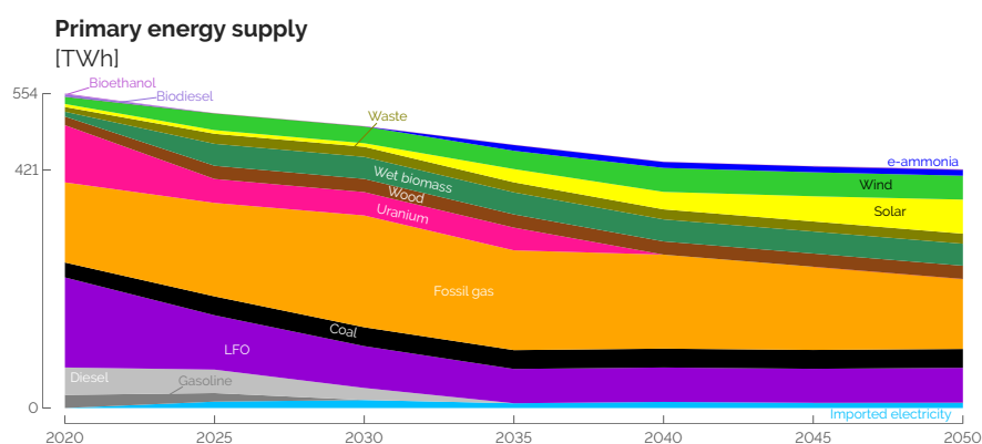
Figure C.12. Primary energy mix of a non-constrained energy transition. In this results, carbon neutrality is not reached in 2050. Some fossil fuels remain used.
