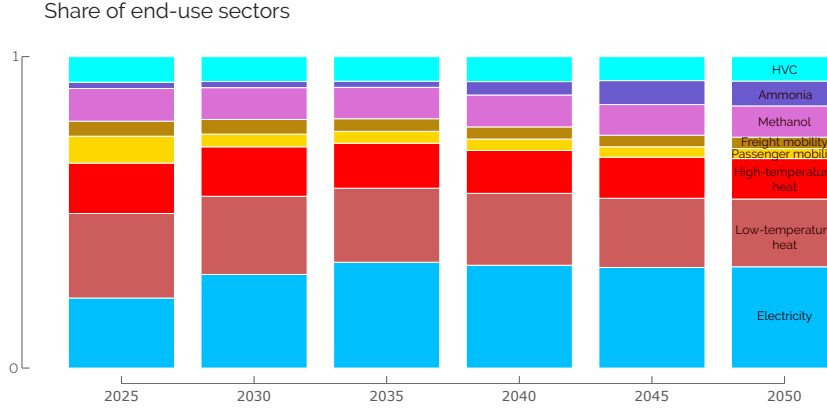
Figure 1.13. Multiplying factors for each of the end-use sectors in the case of the Belgian energy transition. These shares are based on the results of the reference scenario (REF) where nominal values are considered for the uncertain parameters and the transition is optimised through the perfect foresight approach. Over the transition, sectors like electricity (i.e., from 22% in 2025 to 33% in 2050) or ammonia (i.e., from 2% to 8%) become more important due to sector coupling, e.g., e-mobility or ammonia-CCGT.
