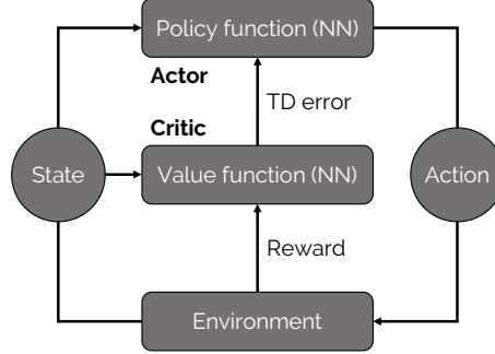
Figure 1.8. General concept of actor-critic-based algorithms. The two NN are trained against each other for the actor to improve the control policy and for the critic to provide a better judgement of the actor’s action via the temporal-difference (TD) error. Graph adapted from [91].
