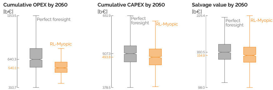
Figure 4.11. Comparison of cumulative OPEX (left), CAPEX (centre) and salvage value (right) in 2050 from the perfect foresight optimisation under uncertainties and the RL-based myopic optimisation.
