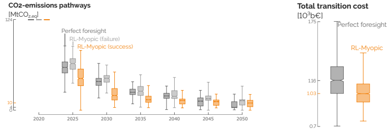
Figure 4.10. Comparison of CO 2 emissions pathways (left) and total transition cost (right) from the perfect foresight optimisation under uncertainties and the RL-based myopic optimisation. Myopic transitions succeed with a more drastic reduction of emissions in the short term and, on average, more favourable economic conditions.
