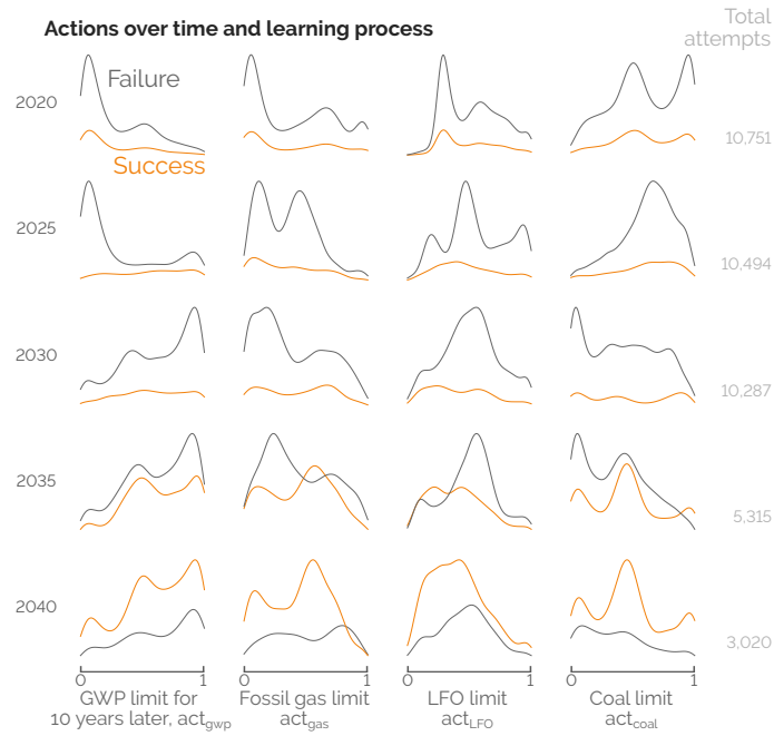
Figure 4.7. Exploration of the action space over the learning process: distribution of occurrence of the different actions at the time they are taken by the agent. The number of remaining attempts decreases with time since infeasible problems and solutions overshooting the CO 2 budget are discarded prematurely, i.e., before 2050. Besides infeasible problems, distributions labelled as “Failure” represent the attempts that overshoot the CO 2 budget by 2050 at the latest. Besides this wide exploration, successes and failures indistinguishably spread over the whole range of actions. In other words, there does not seem to be any clear set of actions to support successful transitions.
