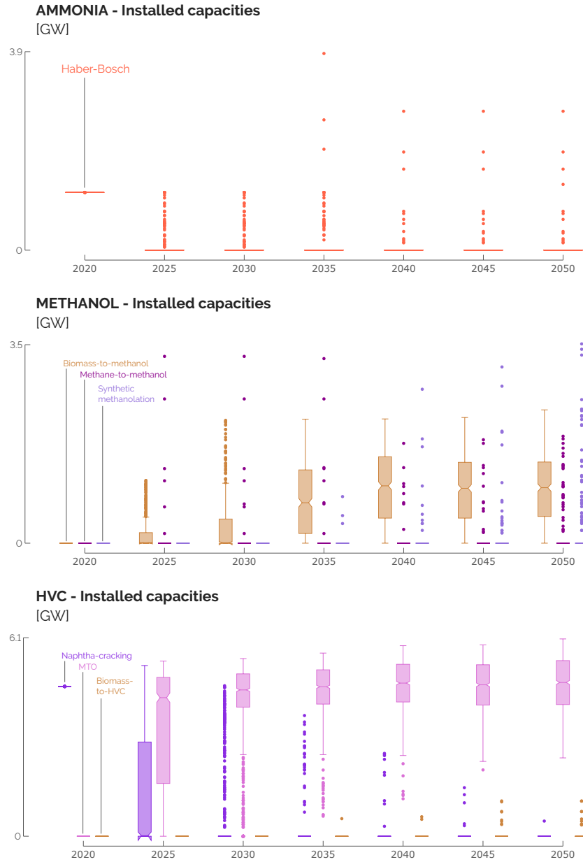
Figure D.6. Distribution of the installed capacities among the end-use sectors of ammonia, methanol and HVC from the Global Sensitivity Analysis (GSA).
