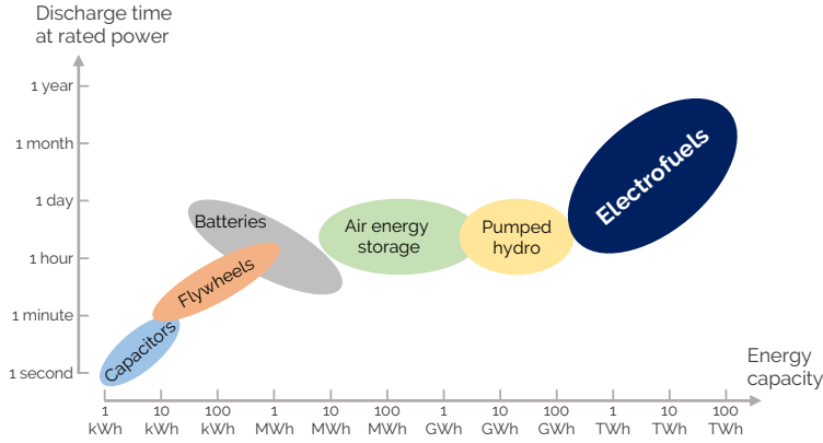
Figure 2. Energy carriers and technologies to store electricity. Electrofuels provide a solution for high-capacity and long-term storage of energy. Graph adapted from [29].
