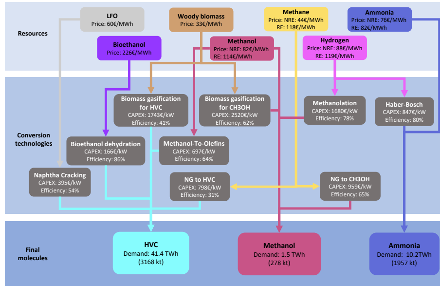
Figure 2.5. Schematic view of the different resources able to produce HVC, ammonia and methanol with their related conversion technologies (including energy efficiency and their CAPEX - in €/kW of final molecules). The efficiencies account for the potential consumption/production of heat and/or electricity within each conversion process. Values stand for 2035. Graph from [121].
