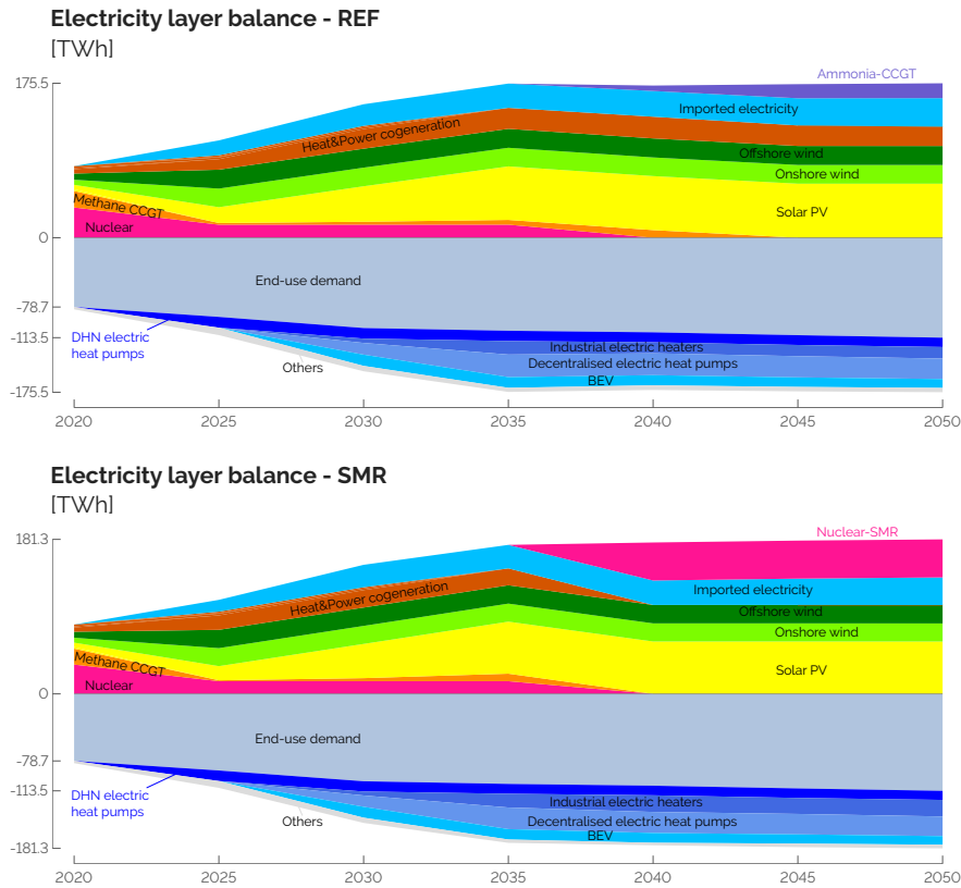
Figure 3.2. Balance between the production and the consumption of electricity in the REF (top) and SMR (down) scenarios. The production of electricity from SMR substitutes more efficient technologies (i.e., CCGT and CHP) and boosts the electrification of the rest of the system, mostly the industrial high-temperature heat sector.
