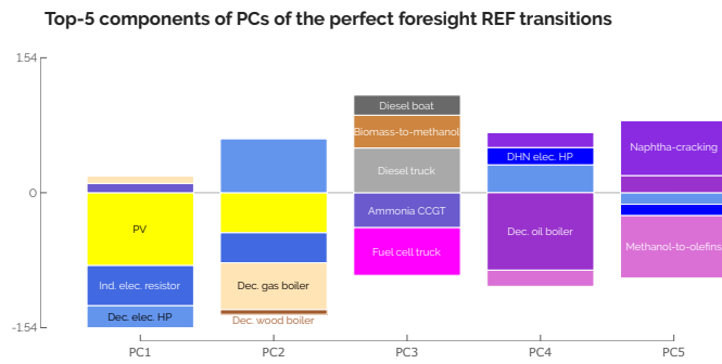
Figure 5.3. Contributions of the top-5 technologies to the different PC transition .
