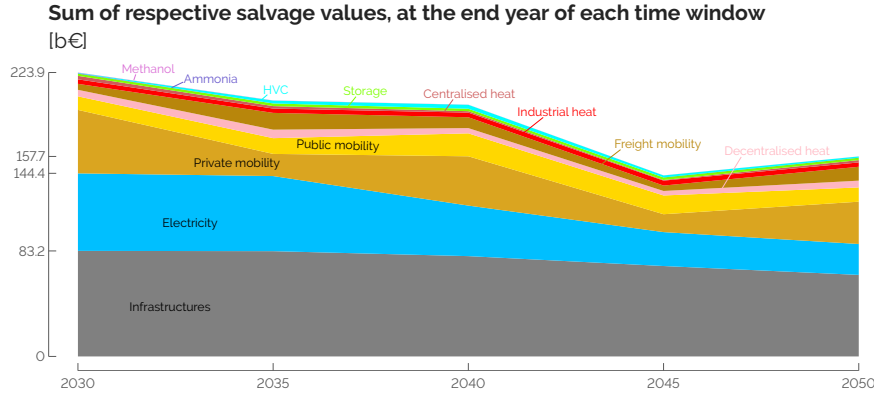
Figure C.9. Sum of the respective salvage values of each sector, per end year of each time window. Altogether, these salvage values represent 223.9 b€, 53% of the cumulative investment costs in 2030, and 157.7 b€, 24% of the cumulative investment costs in 2050.
