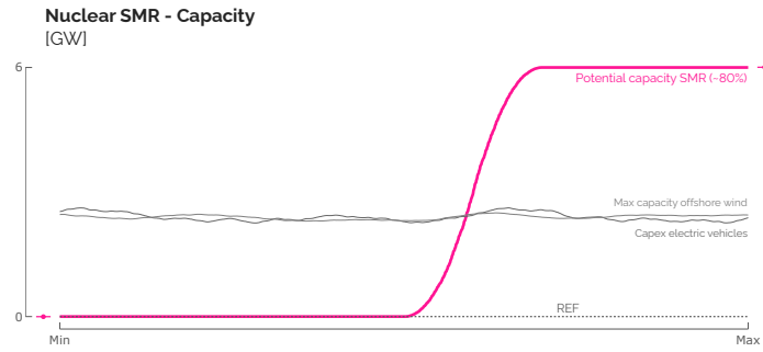
Figure 3.12. Trend lines of the key parameters (and their Sobol' index) on the installed capacity of SMR in 2050. Around these lines, box plots point out the distribution of the output of interest for the extreme values (either bottom-15% or top-15%) of some parameters. The grey dashed line gives the value of the output of interest in the REF case.
