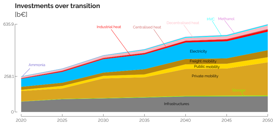
Figure C.5. The cumulative investments over the transition are unequally spread between the sectors. The energy system in 2020 is imposed as the existing energy system and its expenses are split into three main categories: mobility (mainly vehicles), infrastructure (mainly grids) and electricity (mainly thermal power plants). The investments required during the transition represent 150% of the initial investment and are mainly in the same three sectors.
