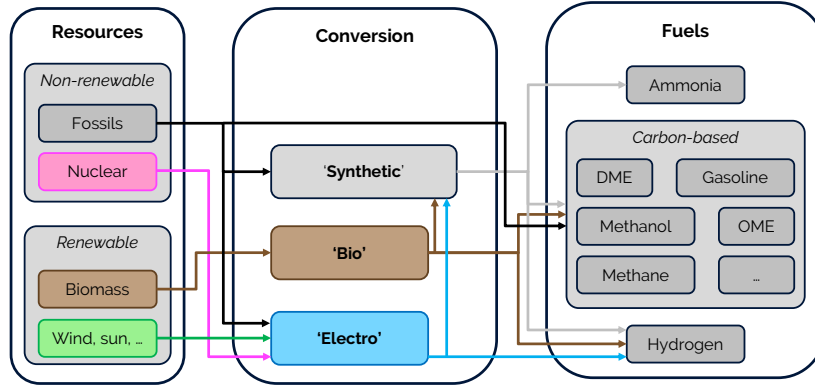
Figure A.1. Overview of the main pathways to produce fuels. The boxes in the “conversion” category illustrates the terminology to use in the different cases: first, a fuel can be defined as bio or electro if the absolute majority of the energy balance of its production consists of biomass or electricity, respectively. Then, a fuel can be defined as synthetic if it has been obtained through a synthesis process from another fuel, regardless of the feedstock. The box “Fuels” gives some examples to illustrate the terminology used and applied to very common fuels.
