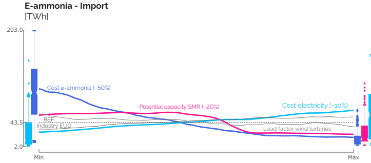
Figure 3.10. Trend lines of the key parameters (and their Sobol' index) on the import of e-ammonia in 2050. Around these lines, box plots point out the distribution of the output of interest for the extreme values (either bottom-15% or top-15%) of some parameters. The grey dashed line gives the value of the output of interest in the REF case.
