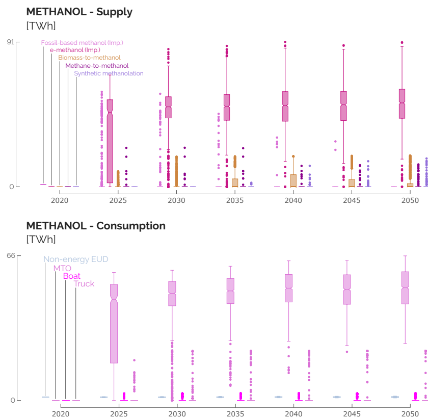
Figure D.4. Distribution of the different streams of supply (top) and consumption (bottom) of methanol from the Global Sensitivity Analysis (GSA).
