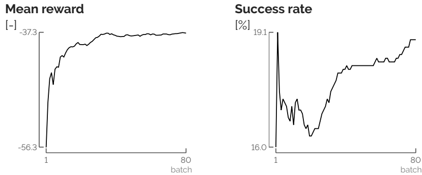
Figure 4.3. Mean reward and success rate of the different learning batches. The stabilisation of the reward curve shows a convergence of the learning process from the agent's point of view. The evolution of the success rate also shows that the reward function aims at more and more successful transitions.
