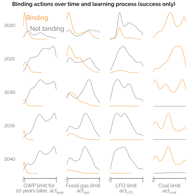
Figure 4.9. Keeping only the successful transitions, distribution of occurrence of binding and not binding actions. Depending on the action and its timing, it is actually constraining the optimisation through EnergyScope Pathway or not. Sweet spots can be identified when considering the limits of GWP and fossil gas consumption. Limiting coal consumption is always constraining, unlike LFO which is “naturally” substituted by EnergyScope Pathway in the near term.
