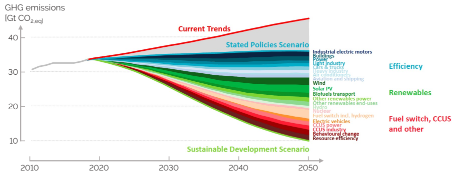
Figure 1. Energy-related CO 2 emissions and reductions by sources in the Sustainable Development Scenario of the International Energy Agency [12].
