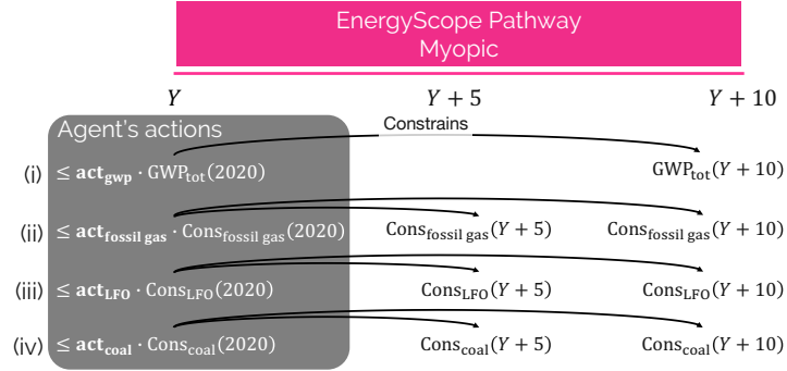
Figure 4.1. Actions available to the decision-maker. Taken at the beginning of the time window to optimise (year Y ), the four actions impact (i) the emissions of the system at the end of the time window (year Y + 10 ) and, (ii-iv) the consumption of fossil gas, LFO and coal at years Y + 5 and Y + 10 . Unlike the first action that sets a target for the end of the time window, the last three aim at limiting the consumption of these fossil resources over the whole time window.
