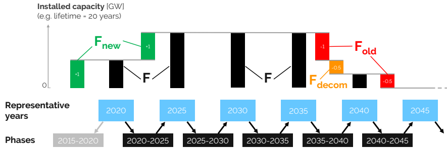
Figure B.5. Example of how the technology capacities and associated variables are evolving.
