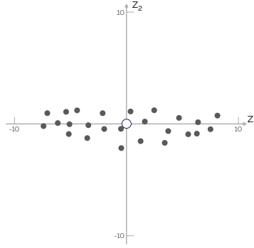
Figure 1.11. Projection of the original observations with respect to their PCs. The variation of the realisations was more significant in the direction of x_2 than x_1 . Once projected with respect to their PCs, the variation is even more significant in the direction of z_1 than in either of the original variables, as it captures most of their variance.
