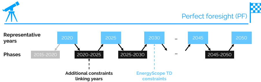
Figure B.4. The pathway methodology relies on 7 representative years (blue boxes) where the model ESTD is applied. Moreover, the formulation accounts for linking constraints (black boxes) and an initial condition (grey box). The overall problem is the pathway model.
