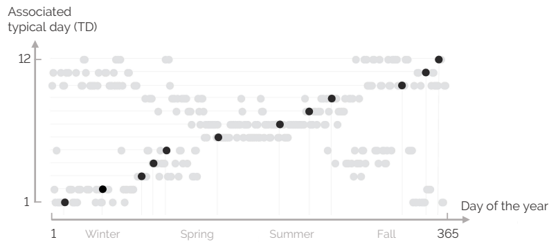
Figure B.2. Association of each day of the year (gray dots) to one of the 12 typical days (TDs) (black dots). Graph adapted from Limpens et al. [52].
