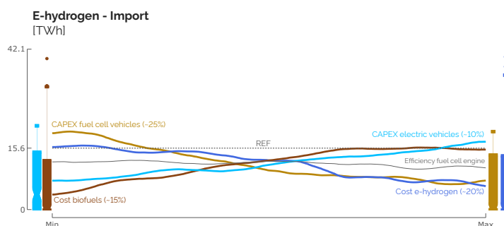
Figure 3.9. Trend lines of the key parameters (and their Sobol' index) on the import of e-hydrogen in 2050. Around these lines, box plots point out the distribution of the output of interest for the extreme values (either bottom-15% or top-15%) of some parameters. The grey dashed line gives the value of the output of interest in the REF case.
