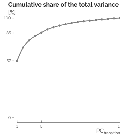
Figure 1.15. Cumulative share of the sum of the transition variance versus the number of PC_{\text{transition}} . Passing a certain threshold, here 85%, the number of PC_{\text{transition}} to consider increases significantly compared to the share of transition variance that they capture.
