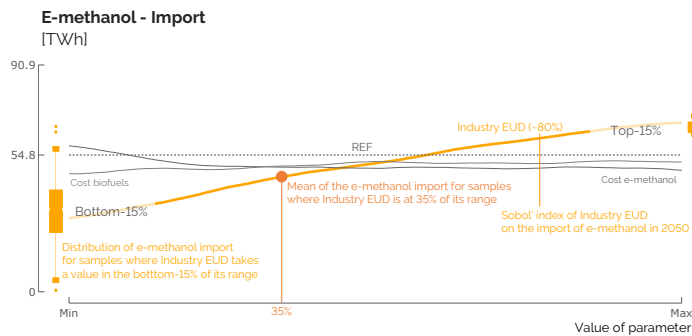
Figure 3.8. Trend lines of the key parameters (and their Sobol' index) on the import of e-methanol in 2050. Around these lines, box plots point out the distribution of the output of interest for the extreme values (either bottom-15% or top-15%) of some parameters. The grey dashed line gives the value of the output of interest in the REF case.
