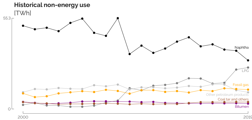
Figure 2.1. Historical data for the non-energy use in Belgium [120]. “Other oil products” account for tar and sulphur. This group also includes by-products of the oil-refining industry like aromatics (e.g., Benzene, Toluene and Xylene (BTX)) and olefins (e.g., propylene). Graph adapted from [121].
