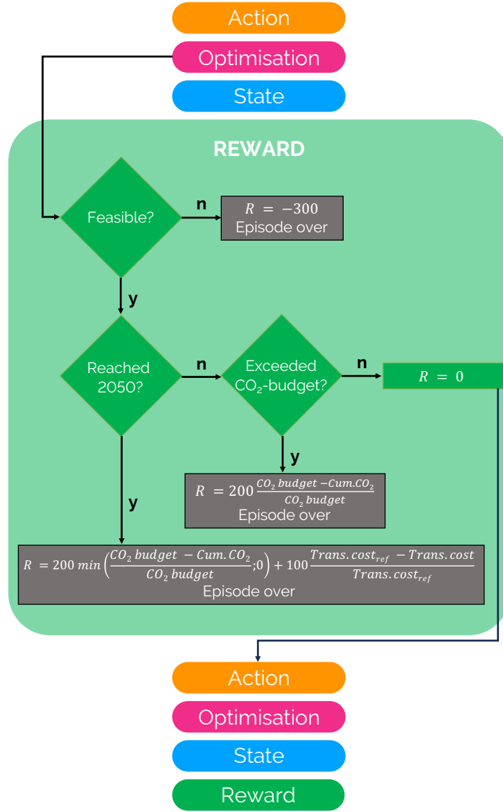
Figure 4.2. Reward function, R . Before 2050, the episode is prematurely ended and a negative reward is given if the optimisation is infeasible or if the \text{CO}_2 budget is exceeded. If the optimisation provides a solution and the \text{CO}_2 budget is not exceeded, the episode continues. Finally, if the episode goes until 2050, the reward is a weighted sum between the capped cumulative emissions and the total transition cost, and the episode terminates. After terminating an episode, the process starts over at the initial state, i.e., 2020.
