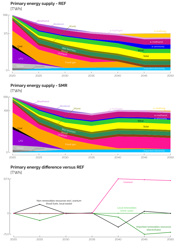
Figure 3.5. (Top) Primary energy mix over the transition for the REF and SMR cases. (Down) Difference of the mix between the two cases after aggregation per category. In line with Rixhon et al. [132], uranium is considered as a non-renewable resource. It is nevertheless dissociated from other non-renewable resources for the sake of clarity. The imported electricity is split between imported non-renewable and renewable resources between the current share of renewables, i.e., 37.41% [159], and an assumed 100%-renewable European electricity mix by 2050.
