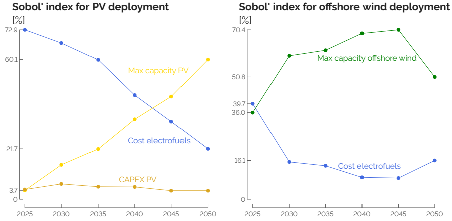
Figure 3.13. Parameters impacting the deployment of PV and offshore wind over the transition. Progressively, the impact of the uncertainty on the maximum potential increases, unlike the one on the cost of purchasing electrofuels.
