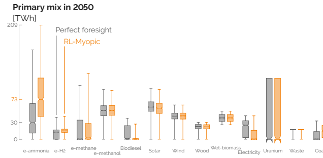
Figure 4.12. Comparison of the primary energy mix in 2050 from the perfect foresight optimisation under uncertainties and the RL-based myopic optimisation. The biggest difference is about e-ammonia to supply CCGT.
