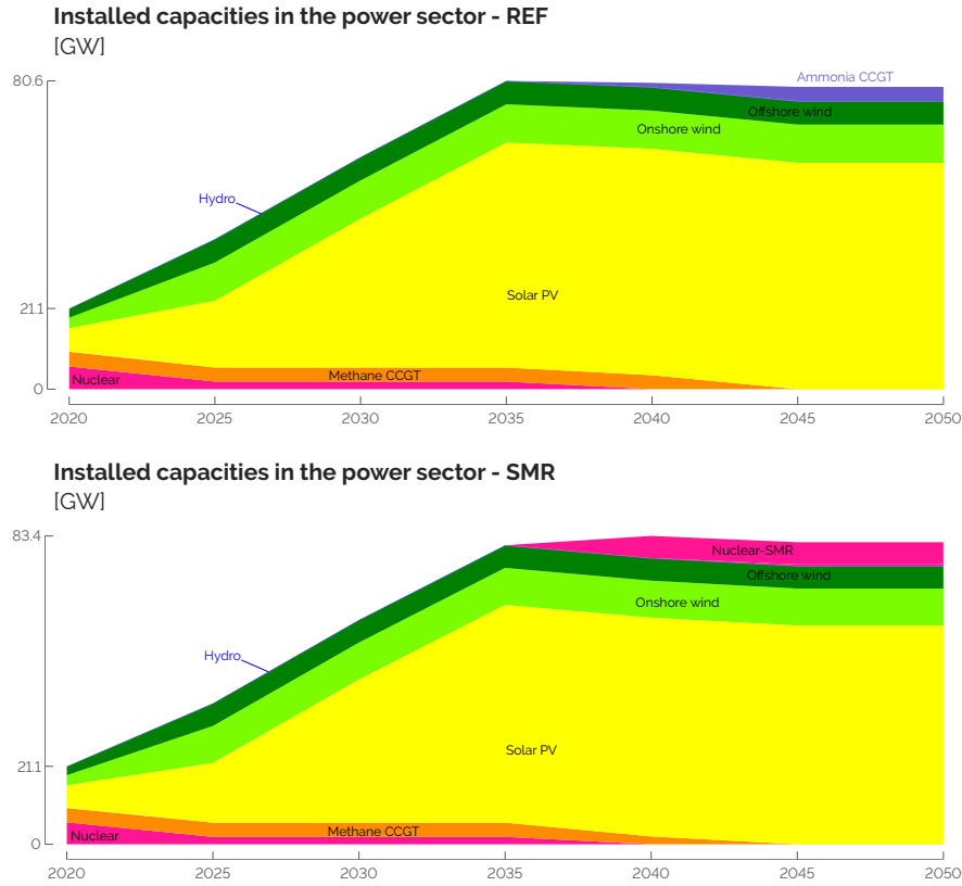
Figure 3.1. Installed capacities in the power sector in the REF (top) and SMR (down) scenarios. As soon as available (i.e., 2040), Small Modular Reactor (SMR) is deployed to its maximum potential (i.e., 6 GW) to substitute more expensive flexible generation units (i.e., methane and ammonia CCGT).
