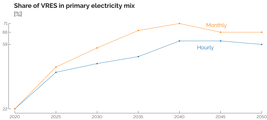
Figure C.13. Share of VRES (i.e., solar and wind) in the electricity primary mix for the monthly and hourly time resolutions.
