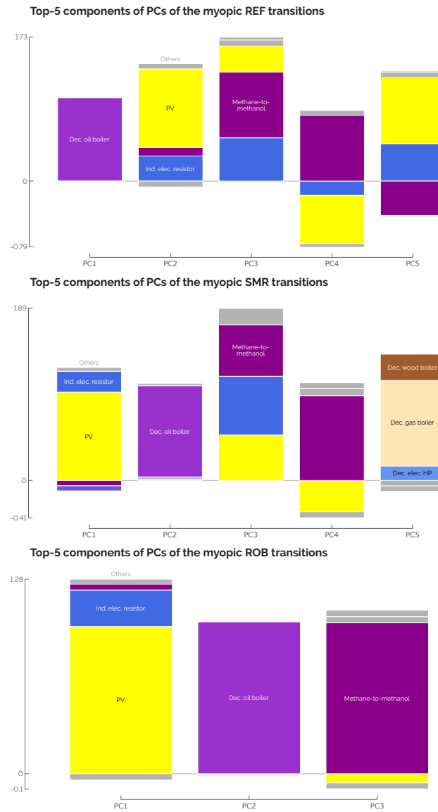
Figure 5.5. Contributions of the top-5 technologies to the PCs of myopic transitions for the REF, SMR and ROB cases. The variation of PV, industrial electric resistors and LT-heat technologies still have a major contribution of the variation in the system roadmaps. At the early stages of the myopic transitions, the installation methane-to-methanol is also subject to significant variations.
