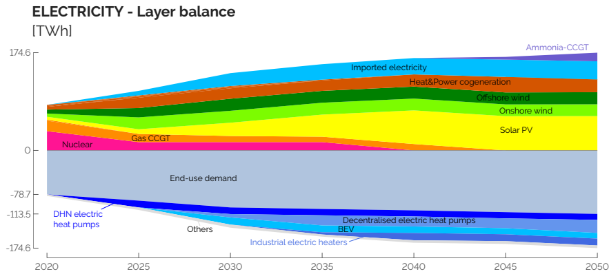
Figure C.4. The electricity supply (positive values) will remain a mix of different technologies where the backup is first mainly provided by gas-CCGT and then imported electricity, heat and power cogeneration and later ammonia-CCGT. The electricity demand (negative values) is led by the electricity end-use demand, but the share used to electrify heat (heat pumps), vehicles (cars, trains, trams...) and industrial heaters drastically increases. This enables a flexible demand that can facilitate the integration of intermittent renewables.
