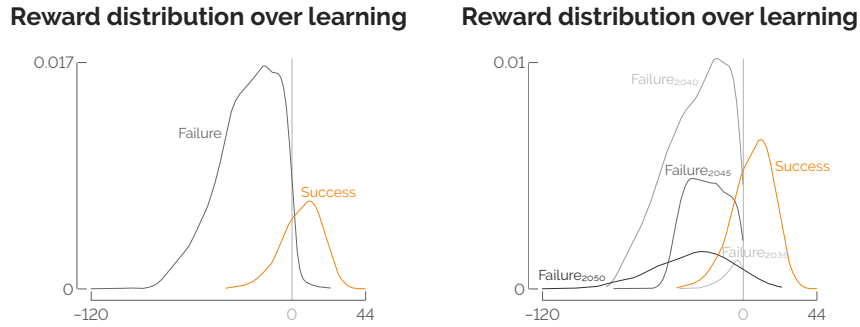
Figure 4.4. Reward distribution between successes and failures. Graph on the right-hand side details at the end of which time window the failure occurred. The “tipping year” is 2040 as failing the transition by 2040 represents 57% of all the failures. Beyond this point, through this learning process, succeeding the transition represents 38% of the episodes.
