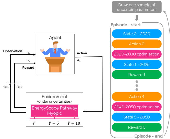
Figure 1.7. The Reinforcement Learning (RL) framework applied to the myopic optimisation of the energy transition pathway between 2020 and 2050. Here, the agent interacts with its environment, i.e., the energy-system model on a limited decision window of 10 years. At the beginning of each episode, a different sample of uncertain parameters is drawn and affects the environment, EnergyScope Pathway, according to the methodology detailed in Section 1.2.1.
