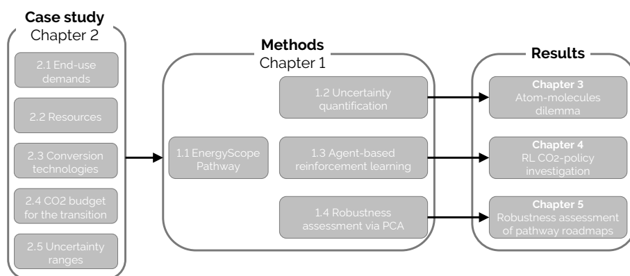
Figure 3. Structure of the thesis. Beyond Chapter 2 that describes the case study of Belgium, Chapters 3, 4 and 5 collect the analyses resulting from the application of the different methodologies developed in Chapter 1. Given the (quasi-)independence of the analyses presented in the last three chapters, they can be read separately.
