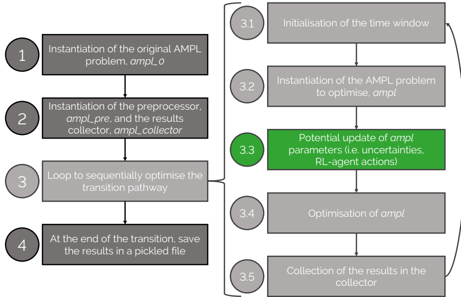
Figure 1.4. Diagram of the iterative optimisation of the whole-energy system transition pathway. Myopic optimisation of the pathway consists of a sequence of smaller LP problems limited to their respective 10-year time window. If the optimisation is not deterministic, step 3.3 is the one where the values of some parameters are changed due to uncertainties (see Section 1.2) or the actions taken by the Reinforcement Learning-agent (see Chapter 4)
