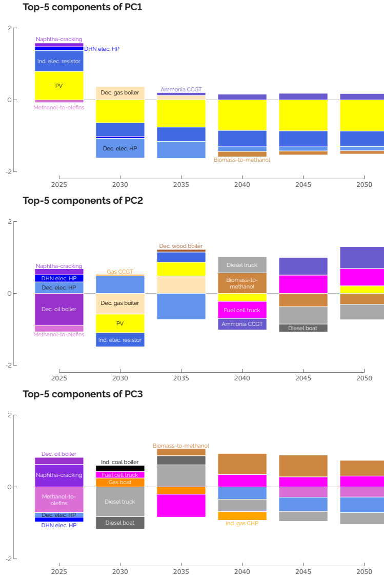
Figure 5.2. Contributions of the top-5 technologies to the first three PCs over the different representative years. Where the variation of PV panels supported by the electrification of the HT heat via industrial electric resistors are the main varying drivers over the whole transition, there are tipping years like 2025 for the production of HVC (i.e., naphtha-cracker to MTO) or 2025-2030 for the production of LT heat (i.e., from oil and gas boilers to electric HP).
