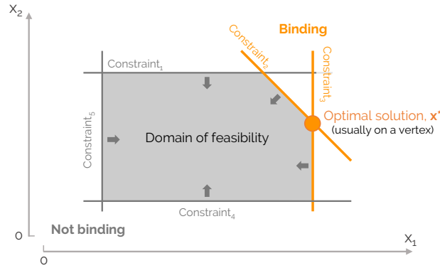
Figure 4.8. Binding versus non-binding constraints. In LP where the feasibility domain is non-empty and bounded, the constraints defined a convex feasibility domain in the space of variables (here, x_1 and x_2 ). The optimal solution usually locates on a vertex of this domain, i.e., the intersection of several constraints (here, constraints 2 and 3) limiting the solution. These constraints are considered binding, i.e., having a limiting impact on the optimal solution.
