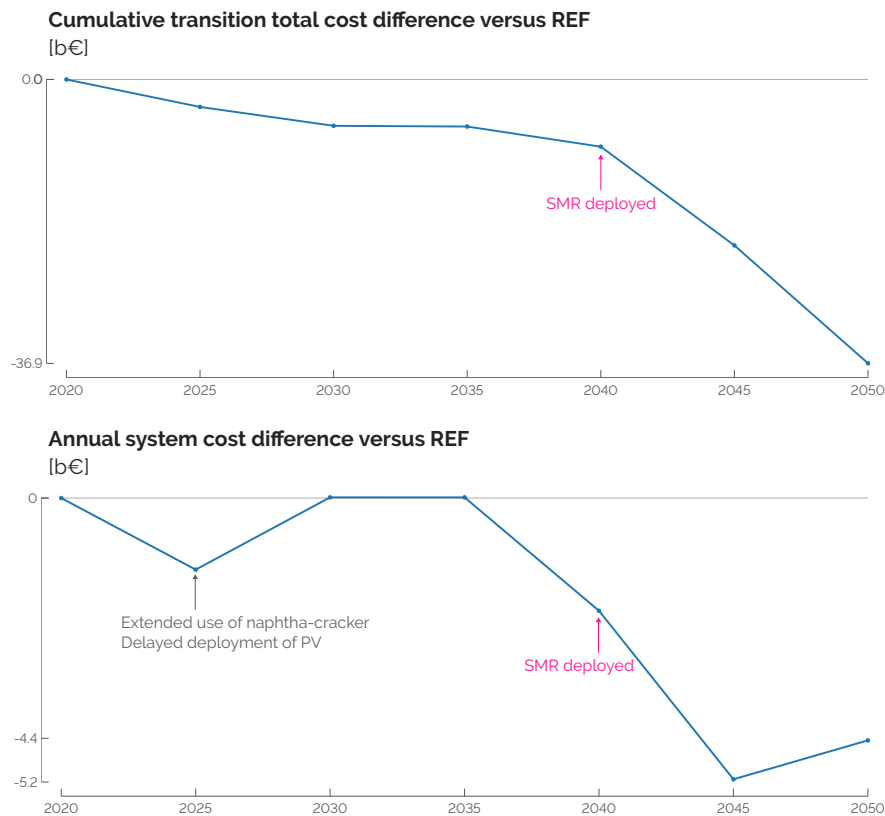
Figure 3.3. (Top) Cumulative transition cost and (down) annual system cost differences between the SMR and the REF cases. Including SMR ends up in a cheaper overall transition (-36.9 b€) and cheaper whole-energy system by 2050 (-4.4 b€).
