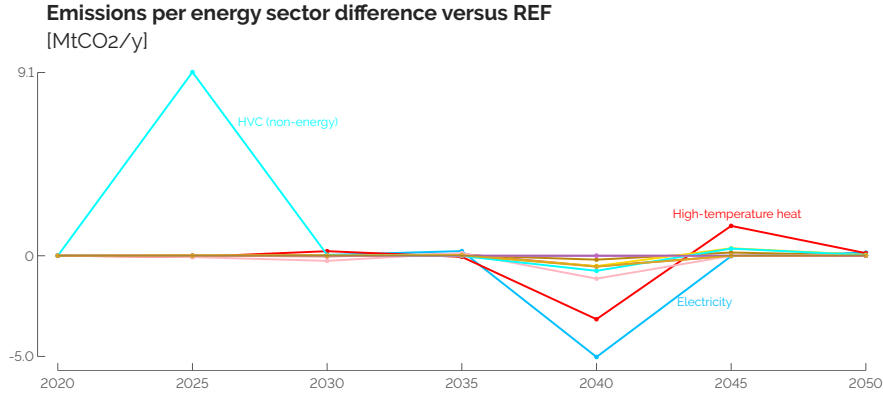
Figure 3.4. Emissions per energy sector difference between the SMR and the REF cases. The deployment of SMR from 2040 onward allows maintaining longer the use of Light Fuel Oil (LFO) for the production of High-Value Chemicals (HVC).
