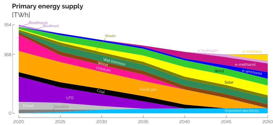
Figure C.2. Primary energy emitting GHG (below Uranium) are decreasing linearly with fossil gas remaining until 2045. A part of this energy is replaced by renewable ones and starting from 2040, a significant share of electrofuels. As end-use demands slightly increase (see Figure 2.2), the drop represents energy efficiency (i.e., providing the same services with less primary energy).
