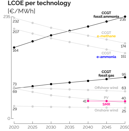
Figure 2.4. Levelised cost of energy (LCOE) for the main technologies in the power sector. Grey and black curves are related to technologies running on renewable and fossil resources, respectively. SMR is cheaper than the other flexible options. CCGT running on e-ammonia is cheaper than its e-methane alternative.
