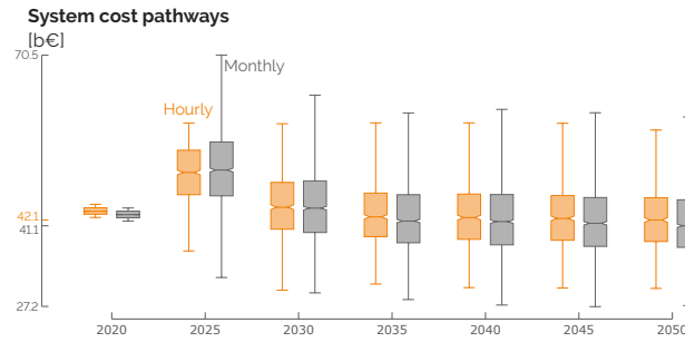
Figure E.2. Comparison of annual system cost pathways from the RL-based myopic optimisation on the hourly and monthly models.
