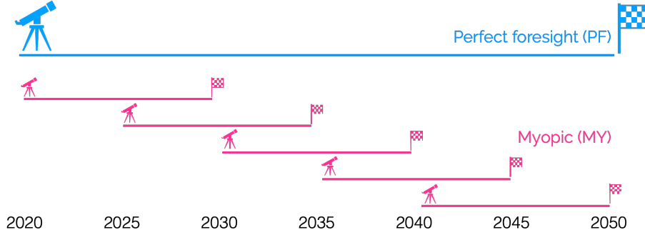
Figure 1.2. The myopic approach (in pink) uses several instances of the pathway model, illustrated in Figure 1.1, as a sequence of different and linked Linear Programming (LP) problems. In this example, the pathway instance has a time horizon of 10 years ( N_{\text{year, opti}} = 10 ) with a 5 year-overlap ( N_{\text{year, overlap}} = 5 ). As a comparison, the perfect foresight (in blue) has a time horizon of 30 years.
