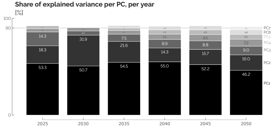
Figure 5.1. PCs capturing at least 90% of the total variance of their respective representative year of the transition.
