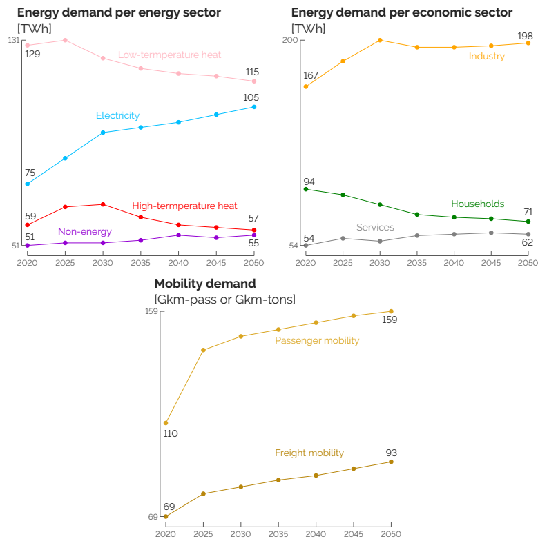
Figure 2.2. EnergyScope splits the whole-energy system end-use demands (EUD) into two sets: (non-)energy and transport-related. This figure presents the yearly values of each of these demands. In the top-right graph, the non-energy demand has been fully associated with the industrial demand. This highlights the significant level of industrialisation of Belgium compared to the other sectors.
