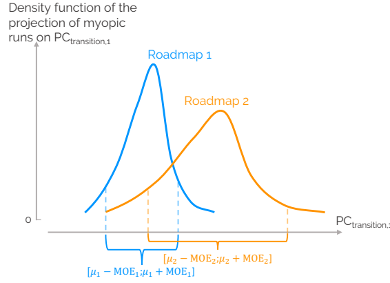
Figure 1.17. Projection on the first PC of the transition, PC_{transition,1} , of the different myopic runs under uncertainties based on different roadmaps. Given that the distribution resulting from roadmap 1 spans over a more narrow range of this PC of the transition, we conclude that this roadmap is more robust than roadmap 2 according to the direction of variation described by PC_{transition,1} .
