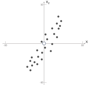
Figure 1.9. Original observations of a two-dimension dataset, x_1 and x_2 .
