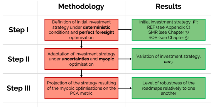
Figure 1.16. Overview of the three-step methodology to assess the robustness of roadmaps. Schematic adapted from [39].
