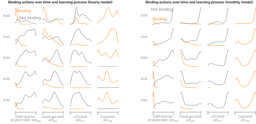
Figure E.1. Binding versus non-binding constraints on the hourly and monthly models: distribution of occurrences. When the agent learns on the monthly model, the actions are binding in the similar timing and similar ranges as when learning on the hourly model.
