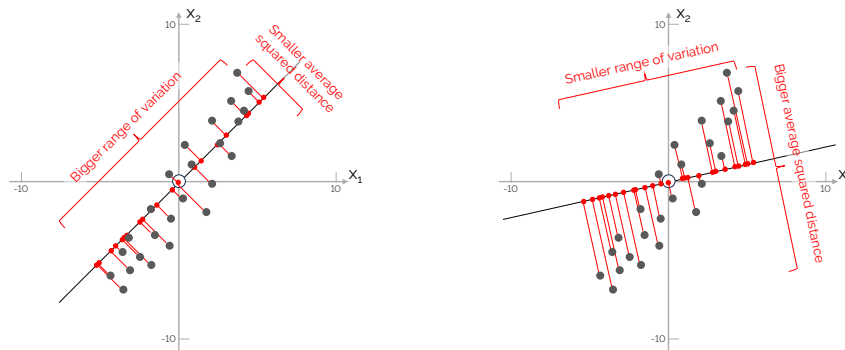
Figure 1.10. Two different projections (red dots) of the original observations (grey dots). The projection on the left captures a bigger variance than the projection on the right. At the same time, the average squared distance between the original observations and their respective projection is smaller for the projection on the left. Consequently, the left projection is closer than the right projection to be the first PC.
