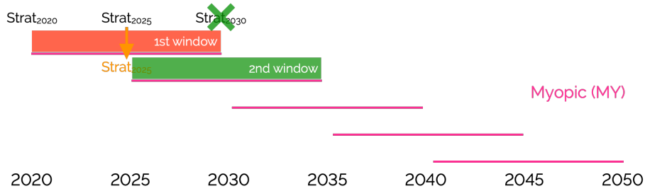
Figure 1.3. Sequential optimisation of the transition pathway in the myopic approach: (i) first time window optimisation, (ii) set-up of the initial conditions of the second time window, (iii) second time window optimisation discarding intermediate results from the first time window optimisation.
