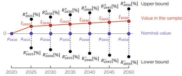
Figure 1.5. Expansion of the width of the uncertainty range for type III parameters. \mu_{2020}, \mu_{2025}, \dots, \mu_{2050} are the nominal values equal to 0 as the uncertain parameters represent a relative increase/decrease of actual parameters of the model. R^+ and R^- are respectively the upper and lower bounds of the range and \xi_{2025}, \xi_{2030}, \dots, \xi_{2050} are the values taken by one parameter for a specific sample of the GSA for each of the representative years of the transition, always starting from the nominal value in 2020, \mu_{2020} . The graph has been adapted from [47].
