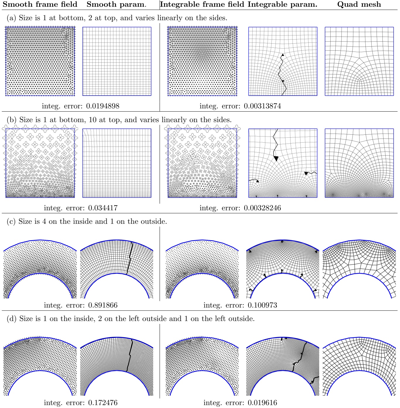
Figure 8: Comparison of smooth frame fields and integrable frame fields when sizes are imposed on boundaries. For each frame field the corresponding parametrization is illustrated, and a quad mesh is computed using guidance from the integrable frame field. All frame fields are isotropic. For cases (a) and (b) we also illustrate the polynomials p_{\mathbf{T}}(\theta) corresponding to the frames.
