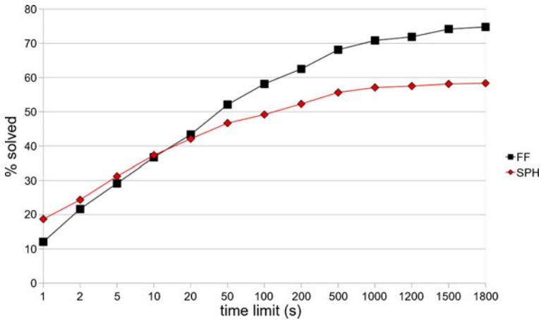
Fig. 12 Delay side constraints: number of instances solved in a given time limit
