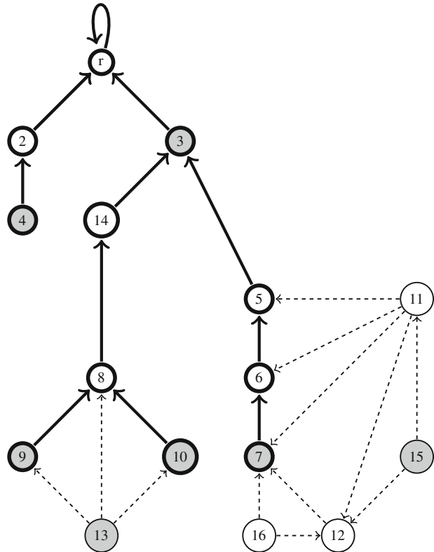
Fig. 6 Partial solution: BA_P contains only one rooted tree ( q = 6 )
