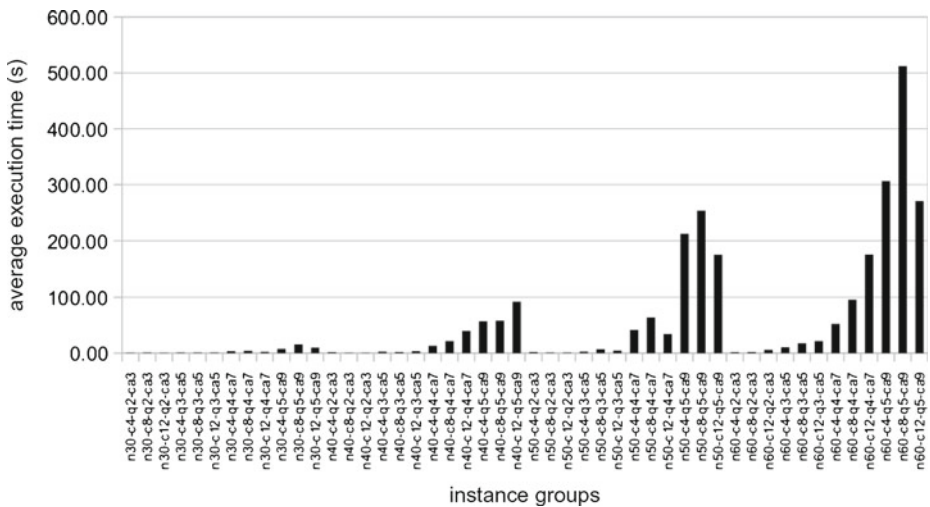
Fig. 10 Average of execution time of the SPH algorithm for ten instances of each group in the first class
