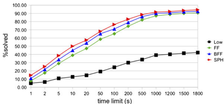
Fig. 9 Complete algorithms: comparison between FF, BFF, SPH, and low heuristics in term of number of instances solved in a given time limit (second instance class)
