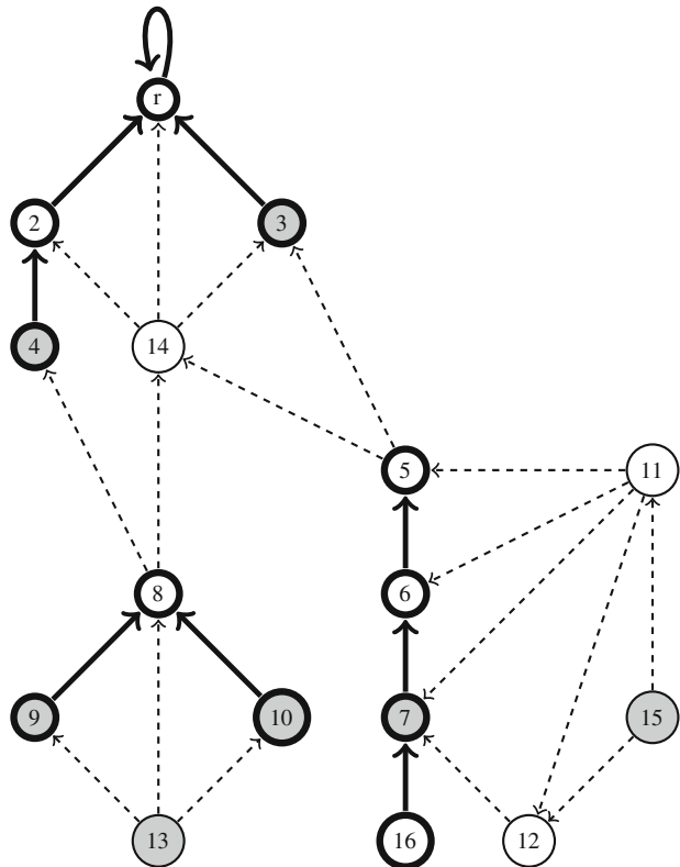
Fig. 2 Partial solution: grey nodes are multicast nodes, the value of q is 6
