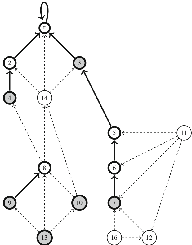
Fig. 7 Partial solution: BA_P contains more than one rooted tree ( q = 6 )
