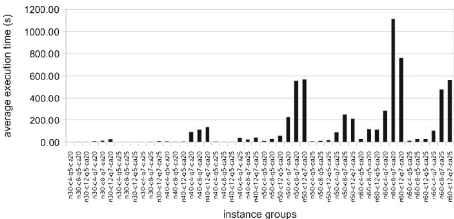
Fig. 11 Average of execution time of the SPH algorithm for ten instances of each group in the second class
