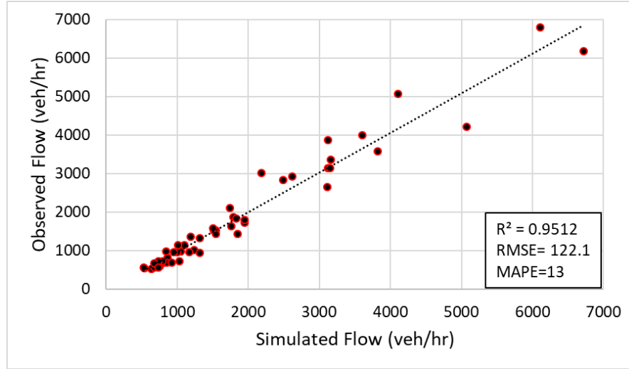
Figure 5: Observed and simulated hourly traffic volumes
