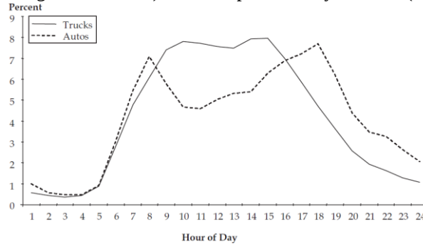
Figure 4: Typical hourly Distribution of Traffic Demand (NCHRP, 2004)
